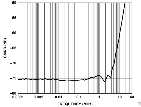
Figure 29. AC CMMR vs. Input Frequency
