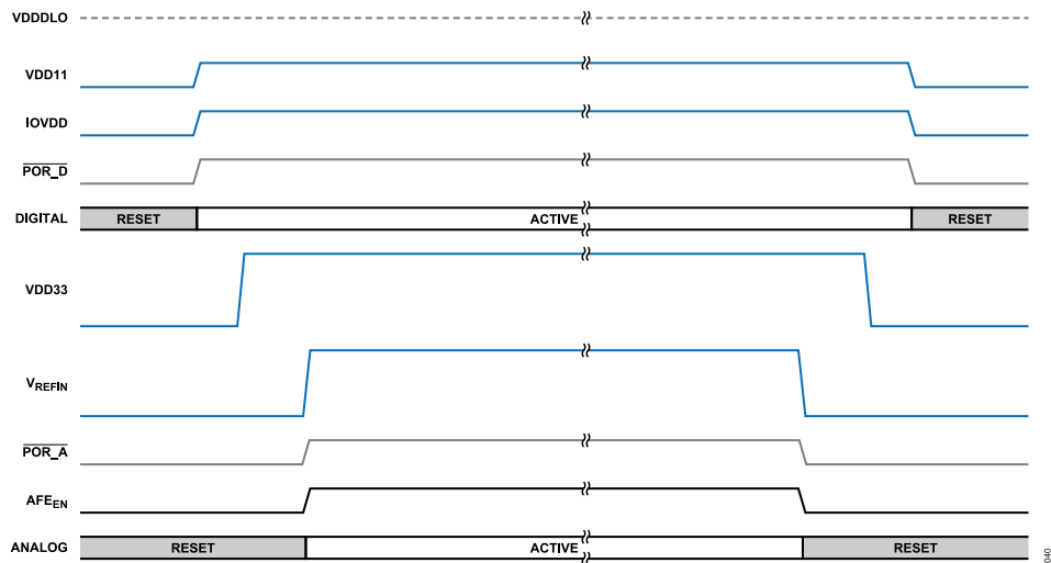
Figure 41. Power Supply Sequence, Externally Generated IOVDD, VDD11
