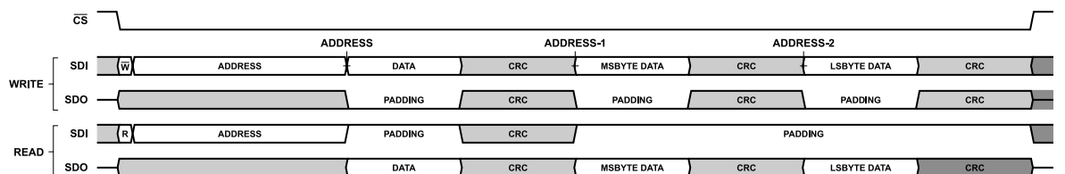
Figure 68. Streaming Mode Configuration with CRC Enabled, STRICT_REGISTER_ACCESS = 0 (Disabled), ADDR_ASCENSION = 0
