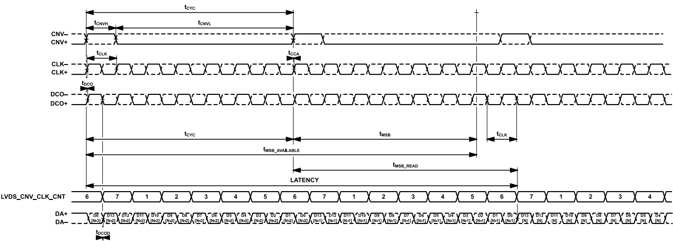
Figure 74. Single Lane LVDS, Echo Clock Mode, LVDS_CNV_CLK_CNT Position Example
