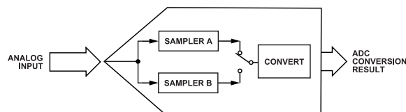
Figure 30. Simplified Representation of the AD4086 SAR ADC
