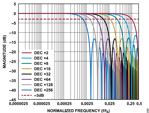
Figure 98. Sinc1 Filter Response, All Decimation Rates
