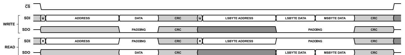
Figure 67. Single Instruction Mode Configuration with CRC Enabled, ADDR_ASCENSION = 1
