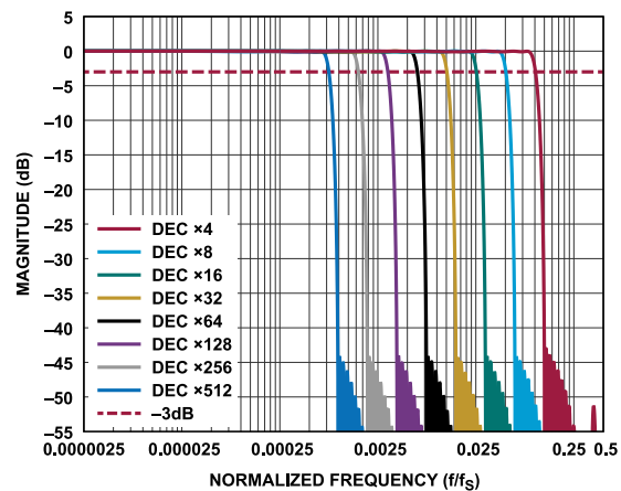
Figure 102. Sinc5 + Compensation Filter Response
