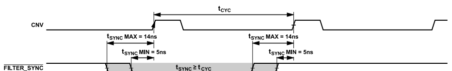
Figure 93. Filter Reset Timing
