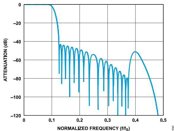
Figure 100. Sinc5 + Compensation Filter Response, Decimate by 2
