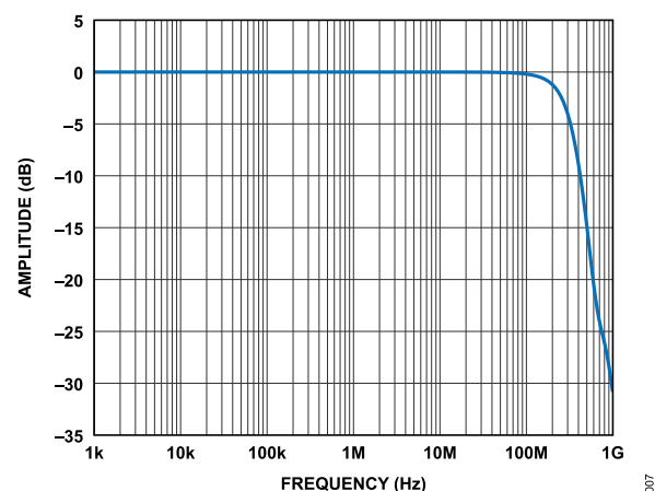
Figure 7. Small Signal -3\text{ dB} Bandwidth at 40MSPS
