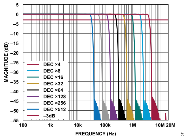
Figure 11. Sinc5 + Compensation Filter Response, f_s = 40\text{MHz}
