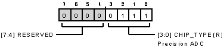
Figure 108. Chip Type Register
