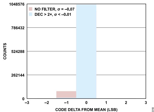
Figure 18. Histogram of Codes, Sinc5 + Compensation, No Filter, Decimate 2x, Decimate 4x ... Decimate 512x
