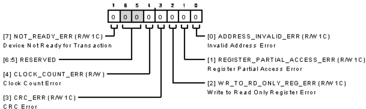
Figure 119. Interface Status A Register
