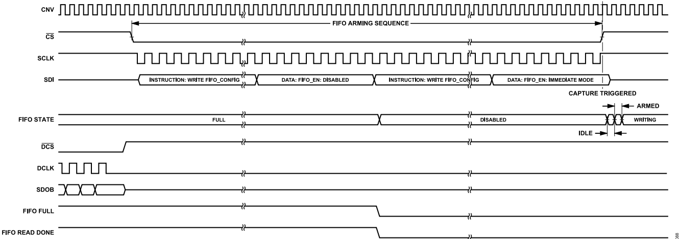
Figure 86. Immediate Trigger Mode Rearming
