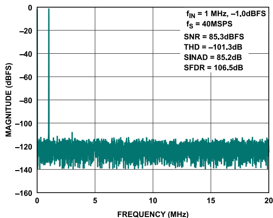
Figure 4. FFT 40MSPS, f_{IN} = 1\text{ MHz} , -1.0\text{ dBFS}
