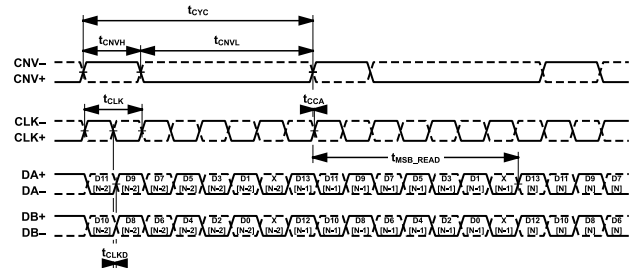
Figure 72. Continuous Conversion Timing, LVDS Data Interface, Dual Data Lane, Self Clock Mode
