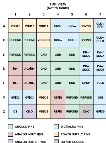
Figure 2. Pin Configuration
