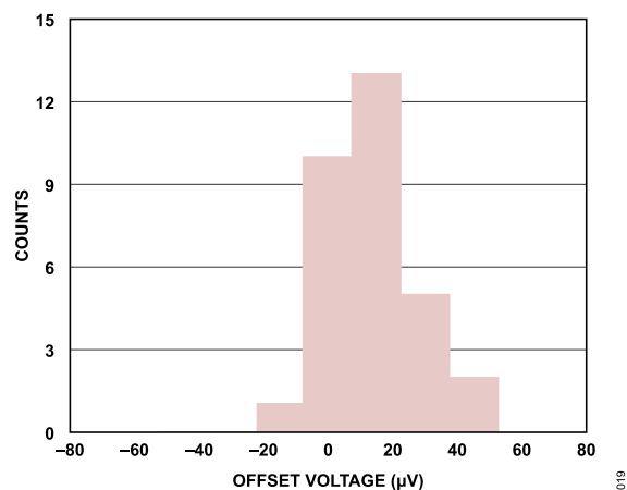
Figure 19. Offset Voltage Histogram
