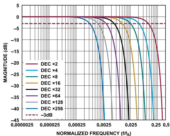
Figure 99. Sinc5 Filter Response, All Decimation Rates
