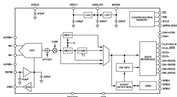
Figure 1. AD4086 Functional Block Diagram
