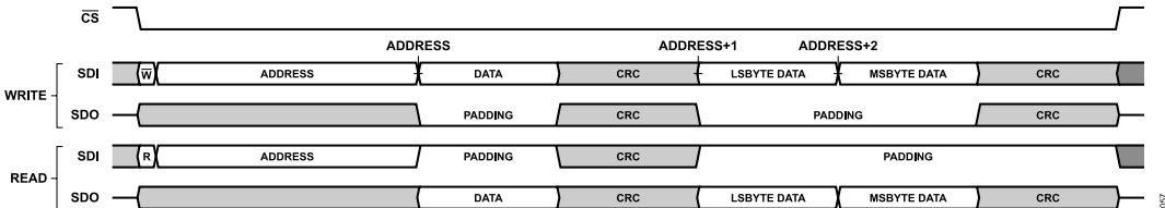
Figure 66. Streaming Mode Configuration with CRC Enabled, ADDR_ASCENSION = 1
