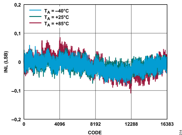
Figure 14. INL vs. Code for Various Temperatures, 40MSPS
