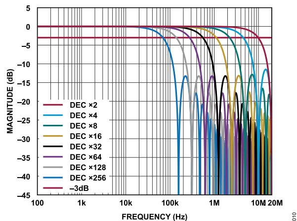
Figure 10. Sinc5 Filter Response, f_s = 40\text{MHz}
