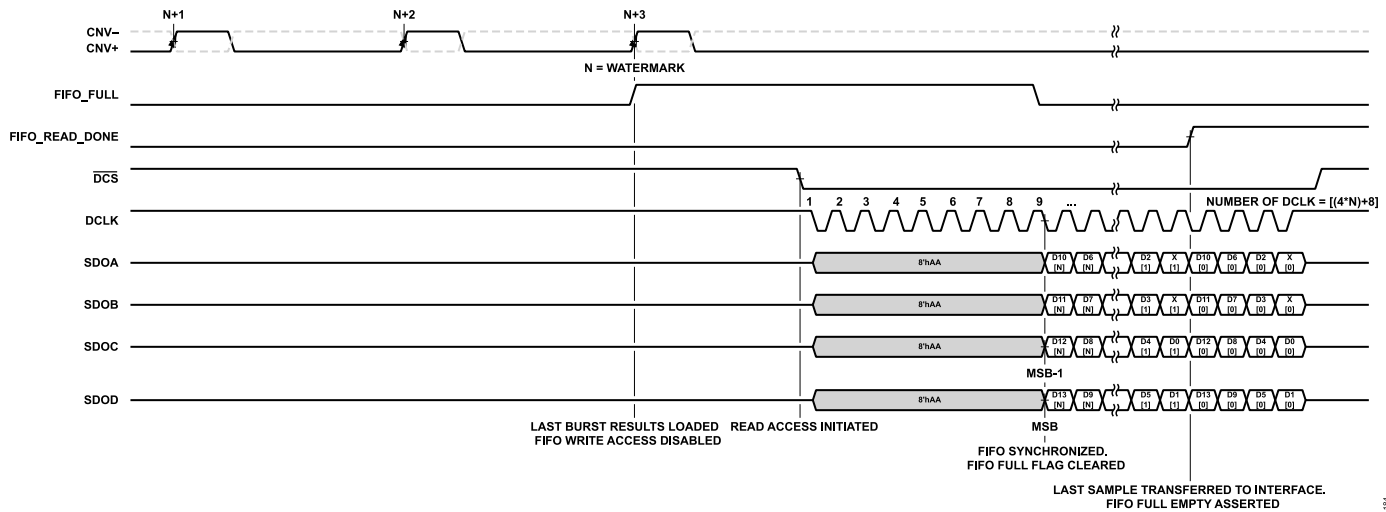
Figure 83. Asynchronous Capture Read Timing, Data FIFO Enabled, Quad Data Lane Configuration
