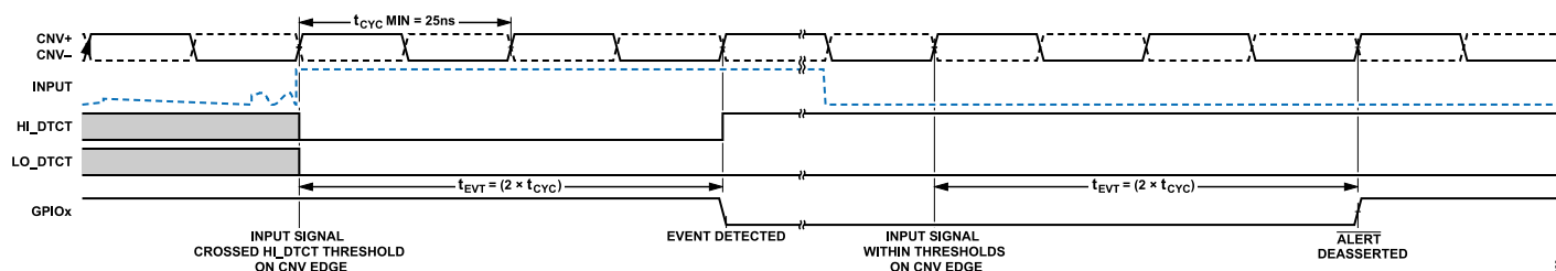
Figure 78. Event Detection Timing
