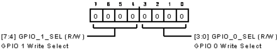
Figure 126. GPIO Configuration B Register
