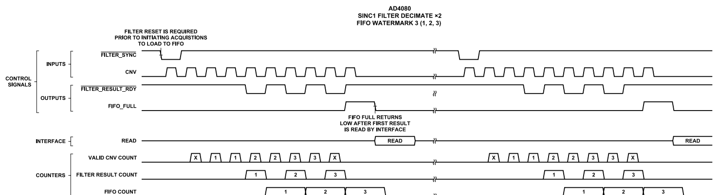
Figure 94. Description of Filter Timing with FIFO
