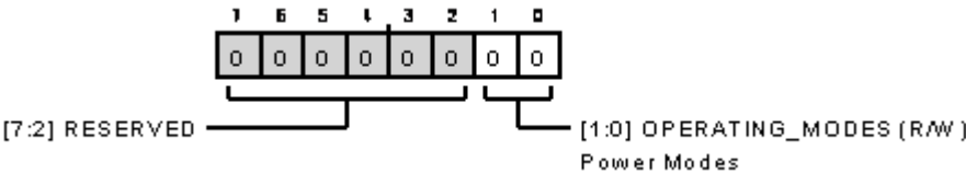
Figure 107. Device Configuration Register
