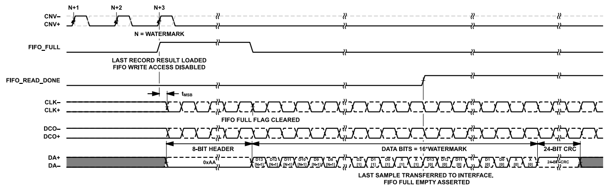
Figure 84. Asynchronous Capture Read Timing, Data FIFO Enabled, LVDS Configuration
