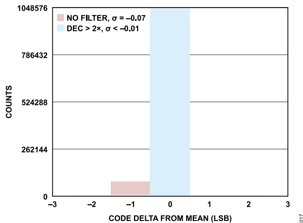
Figure 17. Histogram of Codes, Sinc5, No Filter, Decimate 2x, Decimate 4x ... Decimate 256x
