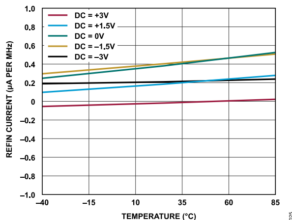
Figure 25. Dynamic REFIN Current vs. Temperature
