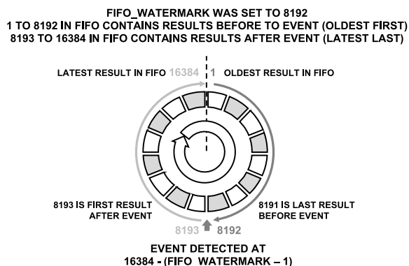
Figure 88. Event Capture Mode Read All FIFO Mode Example, FIFO Filling
