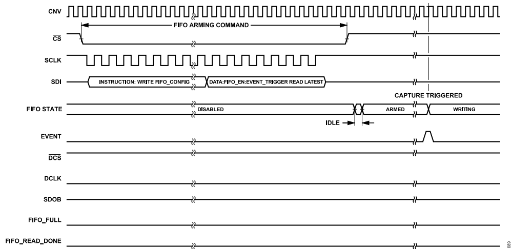
Figure 87. Event Triggered Capture, Read Latest WATERMARK Arming
