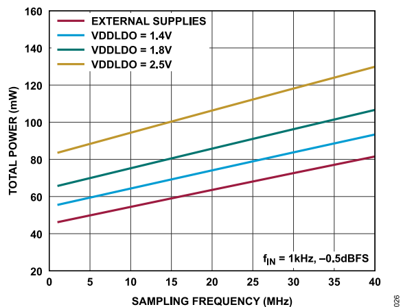
Figure 26. Total Power vs. Sampling Frequency
