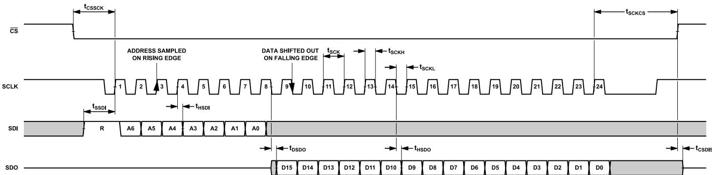
Figure 59. Configuration SPI Timing, Data Read Frame, 8-Bit Instruction Mode, Steaming Mode, Multibyte Register
