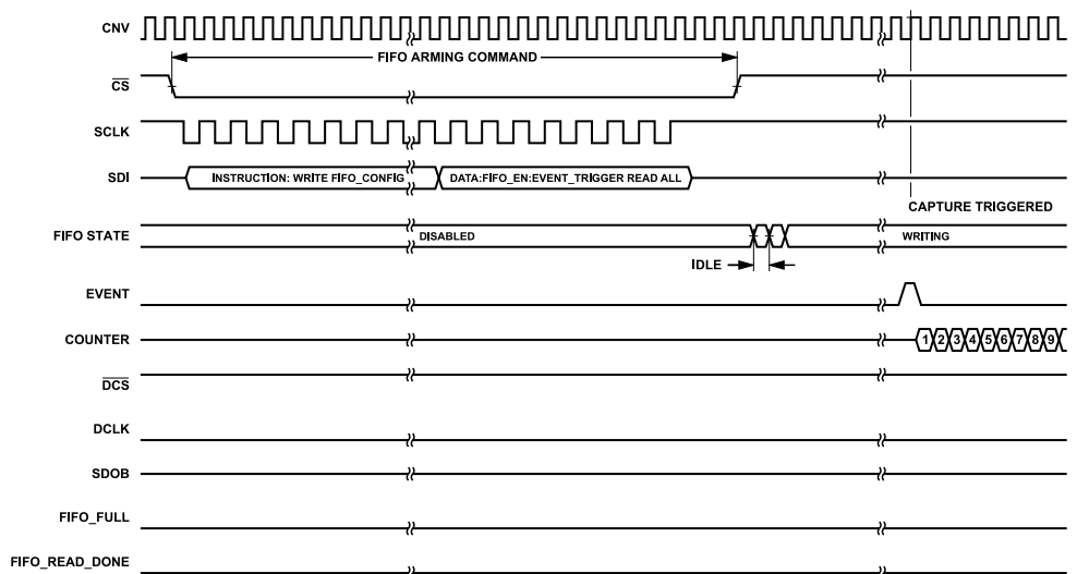
Figure 90. Event Trigger Capture Mode, Read All FIFO Rearming
