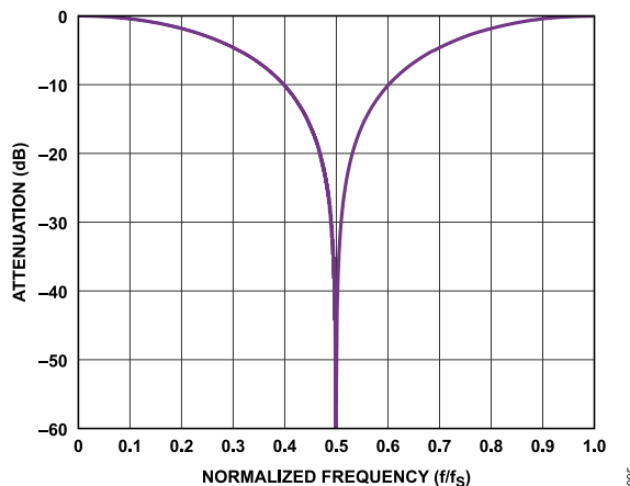
Figure 95. Sinc1 Filter Response, Decimate by 2
