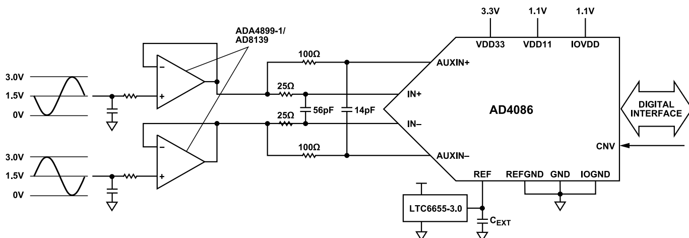
Figure 45. AD4086 Typical Applications Diagram, Single Op-Amp Drivers
