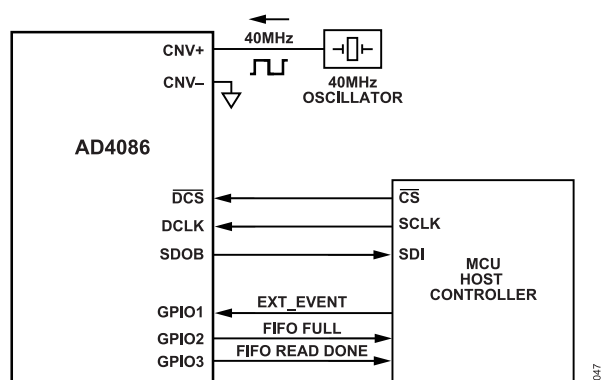
Figure 49. SPI Data Interface Clocking Example
