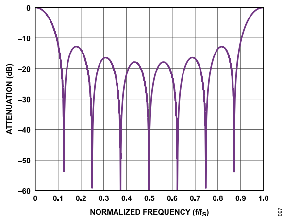
Figure 97. Sinc1 Filter Response, Decimate by 8
