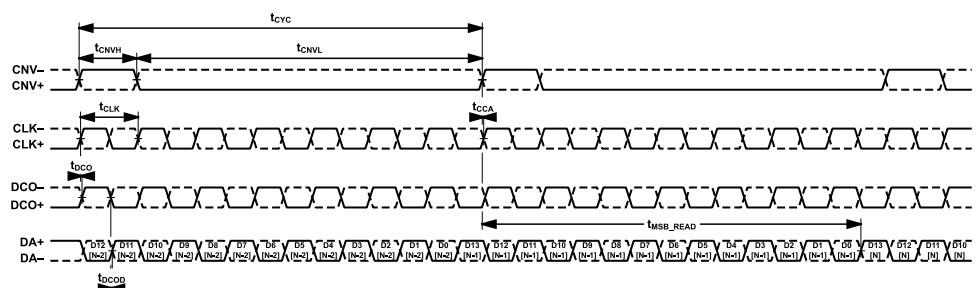
Figure 69. Continuous Conversion Timing, LVDS Data Interface, Single Data Lane, Echo Clock Mode
