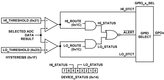
Figure 77. Internally Generated Event Detection Signal Path
