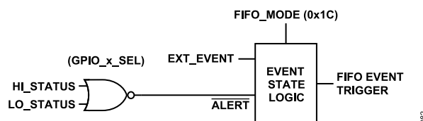
Figure 80. FIFO Event Detection Logic
