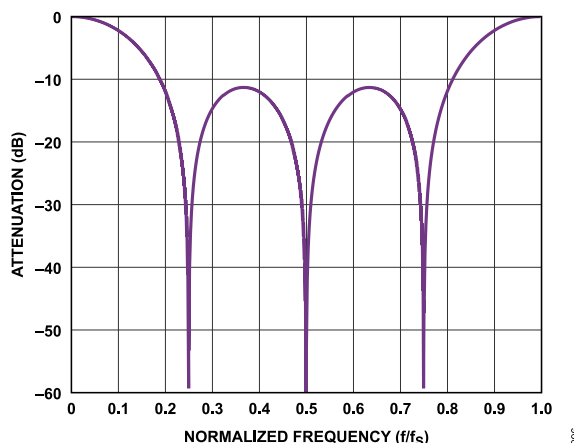
Figure 96. Sinc1 Filter Response, Decimate by 4
