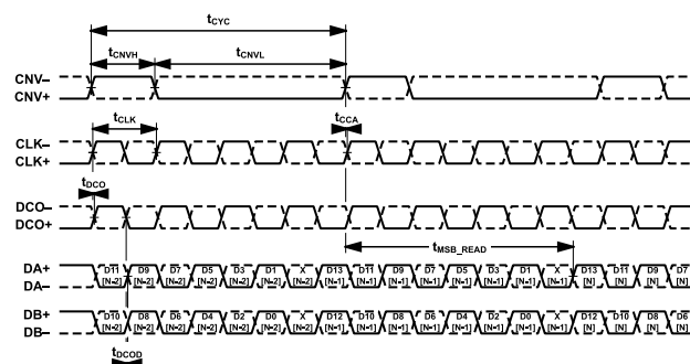
Figure 70. Continuous Conversion Timing, LVDS Data Interface, Dual Data Lane, Echo Clock Mode
