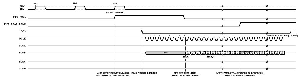
Figure 82. Asynchronous Capture Read Timing, Data FIFO Enabled, Single Data Lane
