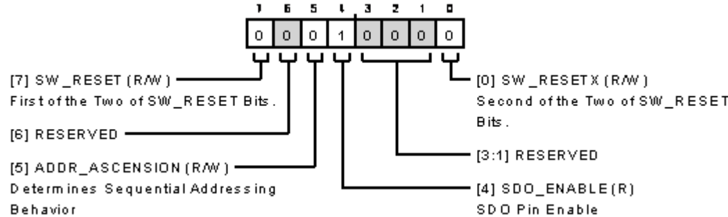
Figure 105. Interface Configuration A Settings
