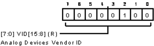
Figure 115. Vendor ID High Register
