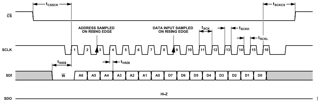
Figure 55. Configuration SPI Timing, Data Write Frame, 8-Bit Instruction Mode, Single 8-Bit Register
