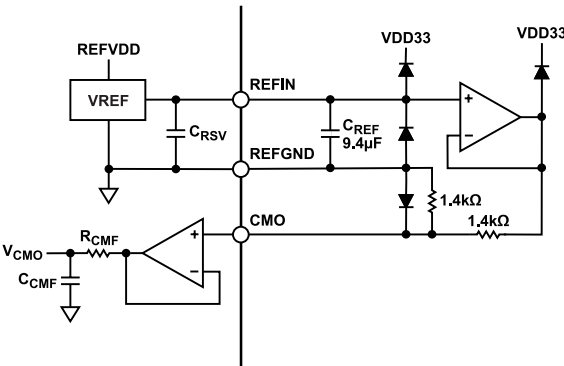
Figure 35. REFIN and CMO Internal Equivalent Circuit and Typical Application
