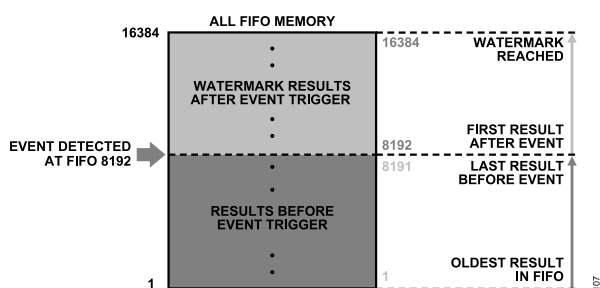
Figure 89. FIFO Event Capture Mode Read All FIFO Mode Example, Locating Event Position in FIFO
