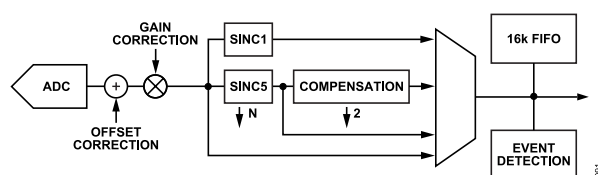
Figure 91. Digital Filter Selection Options
