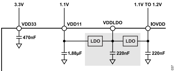
Figure 38. Externally Sourced Supply Configuration
