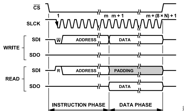
Figure 52. Generic SPI Configuration Frame, CRC Disabled
