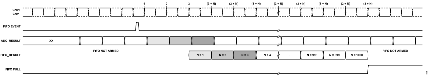
Figure 81. FIFO Data Capture Example, WATERMARK = 1000
