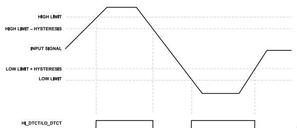
Figure 79. Threshold Detect Levels
