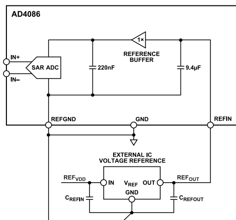
Figure 46. AD4086 General External Reference Design Functional Diagram
