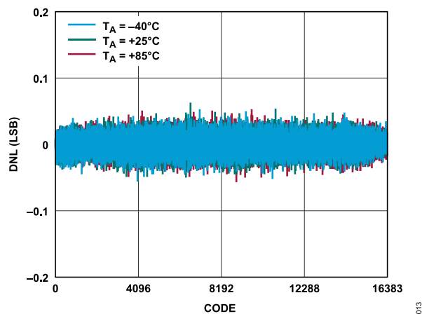
Figure 13. DNL vs. Code for Various Temperatures, 40MSPS
