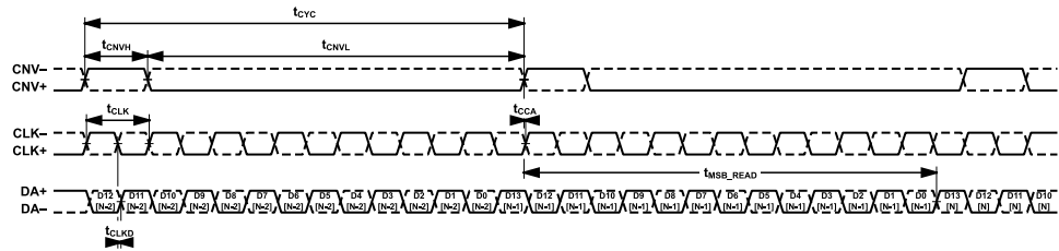
Figure 71. Continuous Conversion Timing, LVDS Data Interface, Single Data Lane, Self Clock Mode
