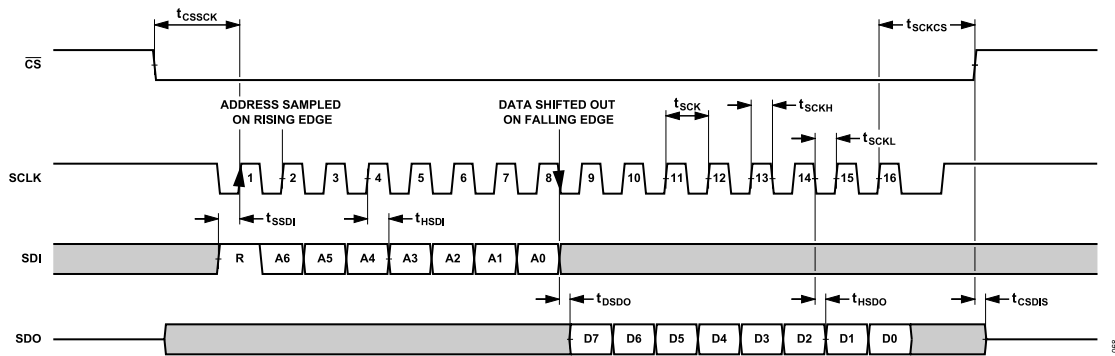
Figure 58. Configuration SPI Timing, Data Read Frame, 8-Bit Instruction Mode
