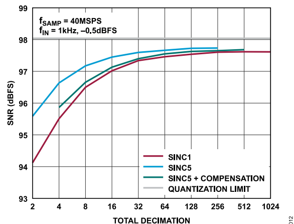
Figure 12. SNR vs. Total Decimation Factor
