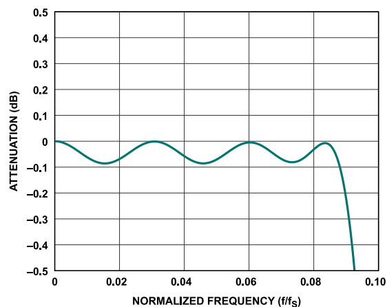
Figure 101. Sinc5 + Compensation Filter Response, Decimate by 2, Pass-Band Ripple
