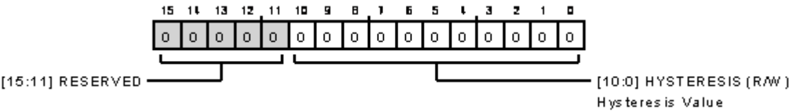
Figure 130. Event Detection Hysteresis Configuration Register
