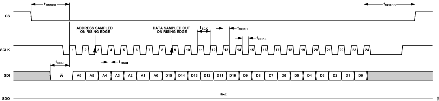
Figure 56. Configuration SPI Timing, Data Write Frame, 8-Bit Instruction Mode, Streaming Mode, Multibyte Register
