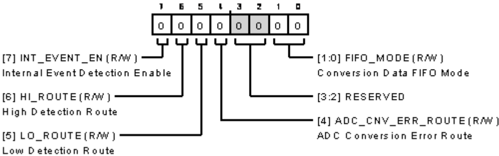
Figure 128. General Configuration Register
