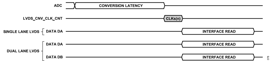
Figure 76. LVDS Data Transfer Latency
