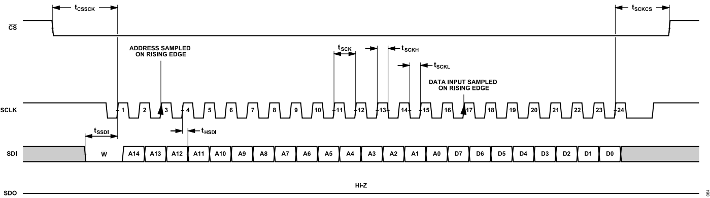
Figure 54. Configuration SPI Timing, Data Write Frame, 16-Bit Instruction Mode (Default)
