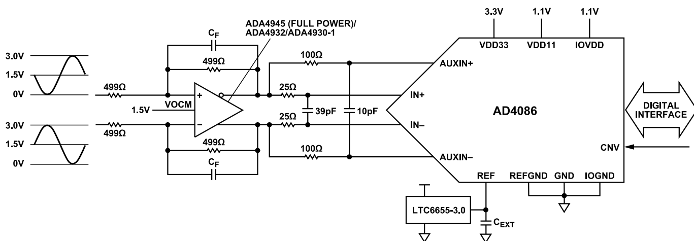
Figure 44. AD4086 Typical Applications Diagram, Fully Differential Amplifier
