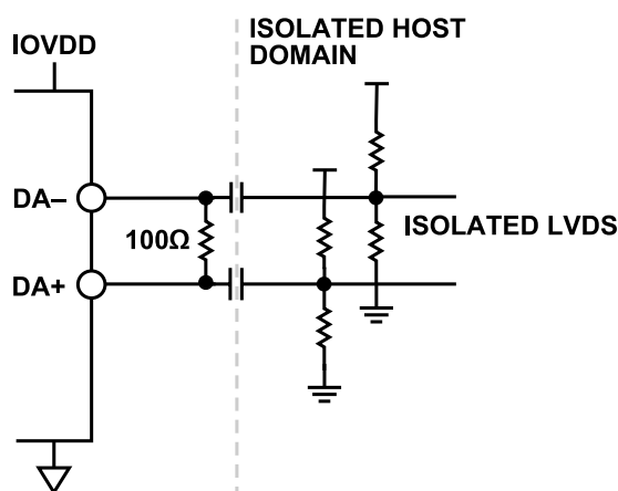
Figure 73. Isolated LVDS
