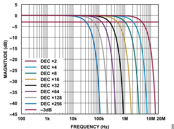
Figure 9. Sinc1 Filter Response, f_s = 40\text{MHz} (DEC \times Means Decimate By)
