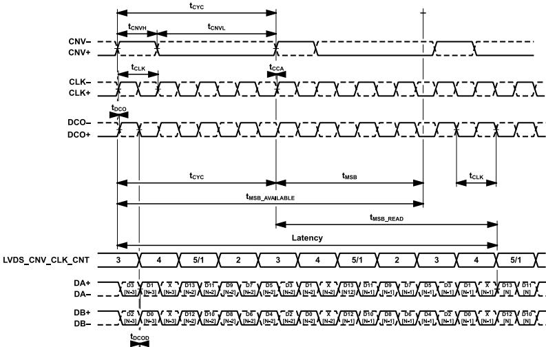
Figure 75. Dual Lane LVDS, Echo Clock Mode, LVDS_CNV_CLK_CNT Position Example
