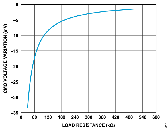
Figure 24. CMO Voltage Variation vs. Load Resistance
