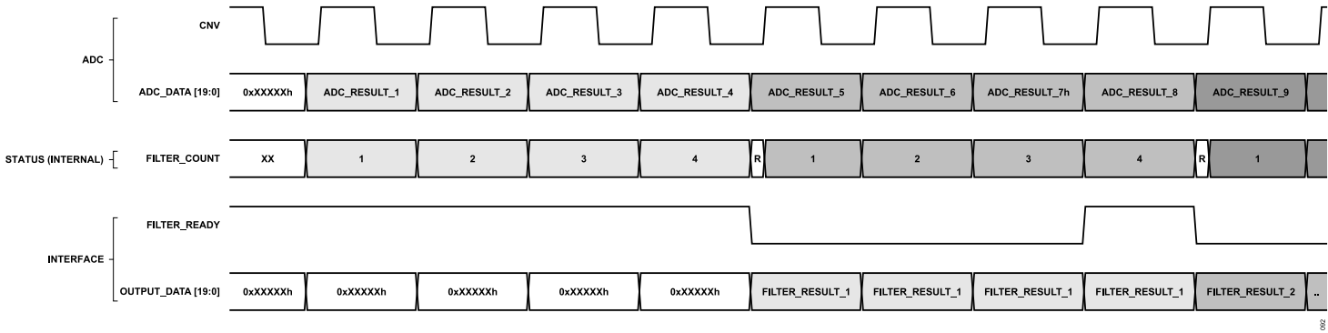
Figure 92. Digital Filter Decimate by 4 Frame Overview
