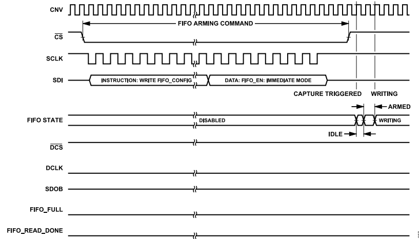
Figure 85. Immediate Trigger Mode Arming
