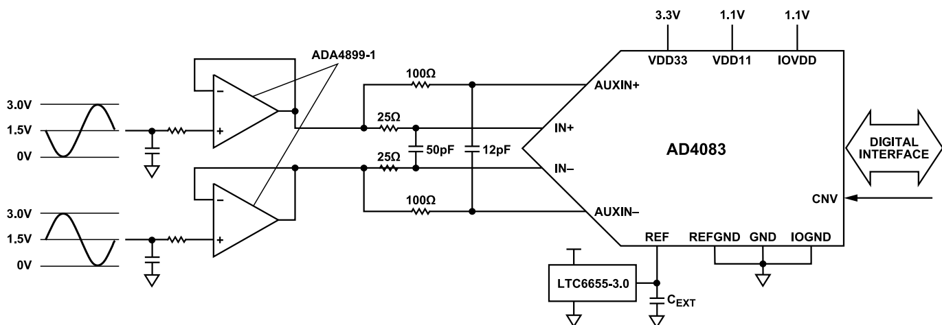
Figure 45. AD4083 Typical Applications Diagram, Single Op-Amp Drivers
