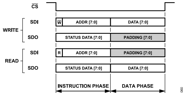
Figure 62. Short Instruction Mode, Data Status Enabled, CRC not Enabled
