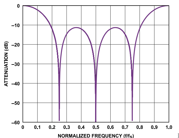
Figure 100. Sinc1 Filter Response, Decimate by 4
