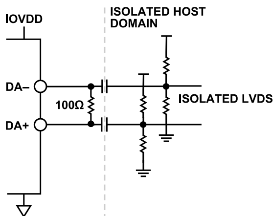
Figure 77. Isolated LVDS
