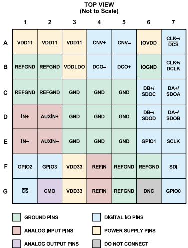
Figure 2. Pin Configuration
