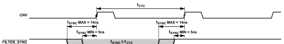
Figure 97. Filter Reset Timing
