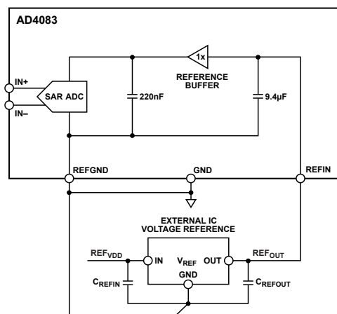
Figure 46. AD4083 General External Reference Design Functional Diagram
