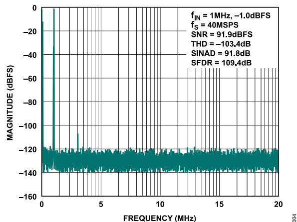
Figure 4. FFT 40MSPS, f_{IN} = 1\text{MHz} , -1.0\text{dBFS}
