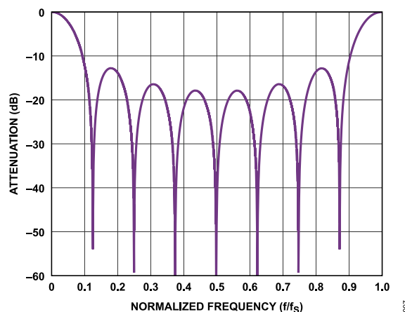
Figure 101. Sinc1 Filter Response, Decimate by 8
