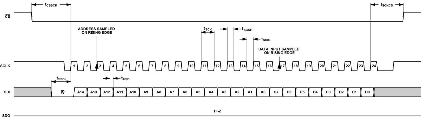
Figure 66. Configuration SPI Timing, Data Write Frame, 16-Bit Instruction Mode (Default)
