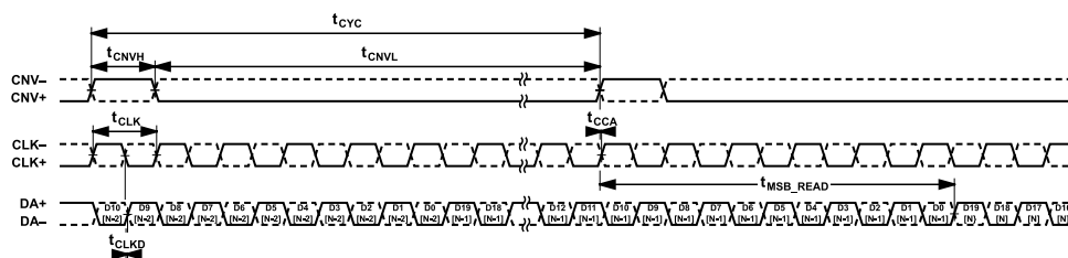
Figure 75. Continuous Conversion Timing, LVDS Data Interface, Single Data Lane, Self Clock Mode
