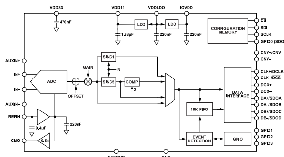
Figure 1. AD4083 Functional Block Diagram
