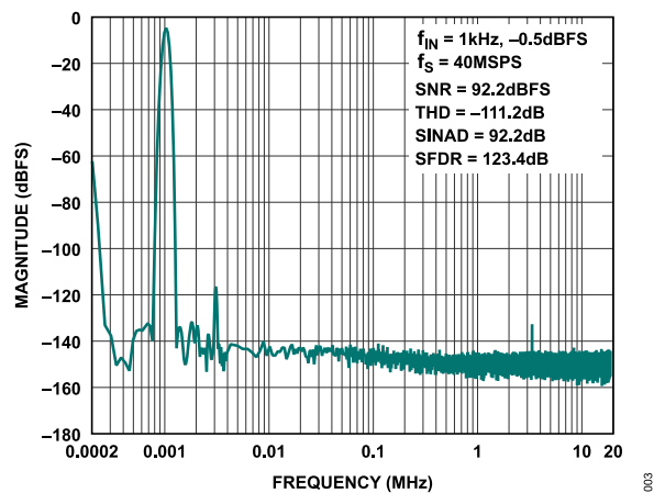
Figure 3. Fast Fourier Transform (FFT) 40MSPS, f_{IN} = 1\text{kHz} , -0.5\text{dBFS}
