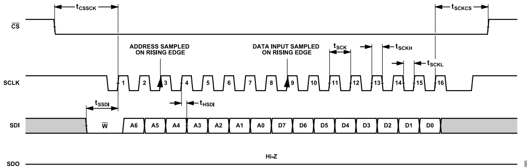
Figure 67. Configuration SPI Timing, Data Write Frame, 8-Bit Instruction Mode, Single 8-Bit Register
