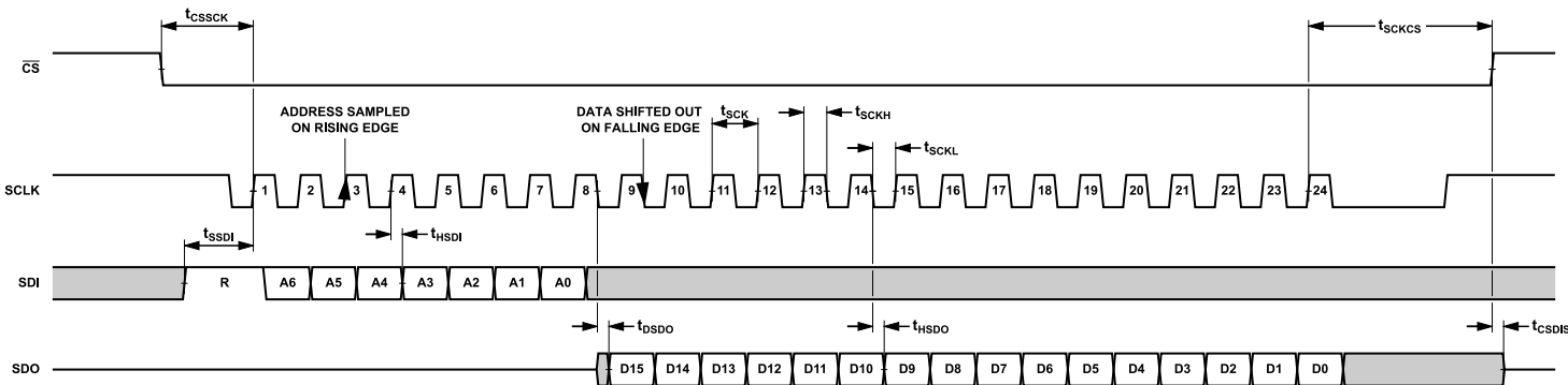
Figure 71. Configuration SPI Timing, Data Read Frame, 8-Bit Instruction Mode, Steaming Mode, Multibyte Register
