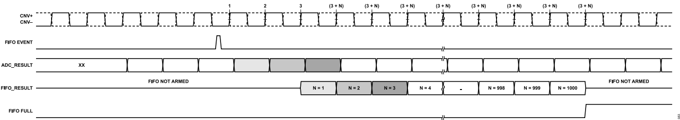
Figure 85. FIFO Data Capture Example, WATERMARK = 1000
