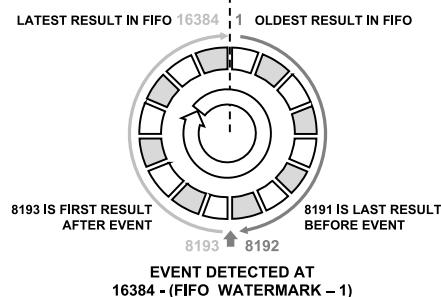
Figure 92. Event Capture Mode Read All FIFO Mode Example, FIFO Filling
