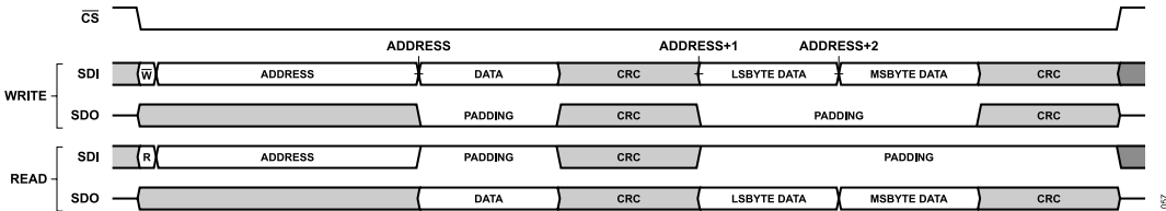
Figure 59. Streaming Mode Configuration with CRC Enabled, ADDR_ASCENSION = 1
