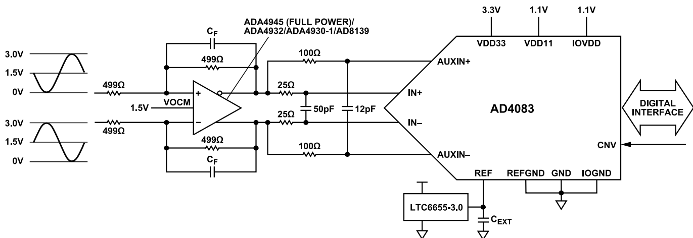
Figure 44. AD4083 Typical Applications Diagram, Fully Differential Amplifier
