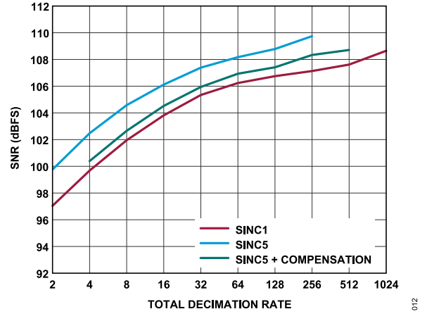
Figure 12. Combined SNR vs. Total Decimation for All Filters
