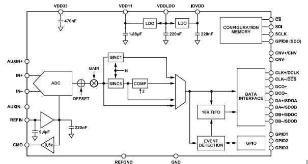
Figure 1. AD4082 Functional Block Diagram
