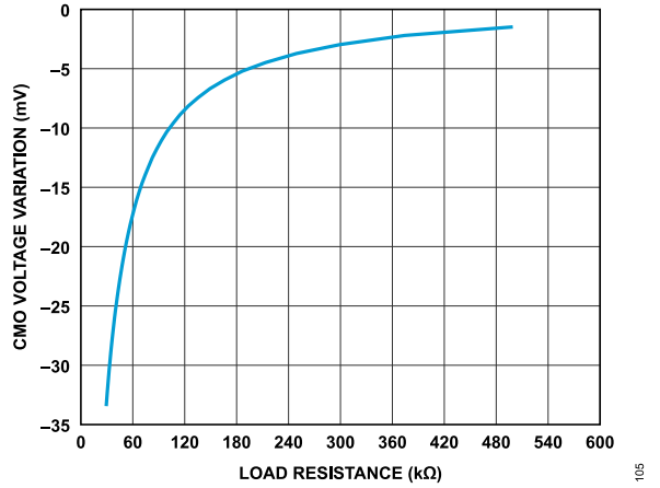
Figure 24. CMO Voltage Variation vs. Load Resistance
