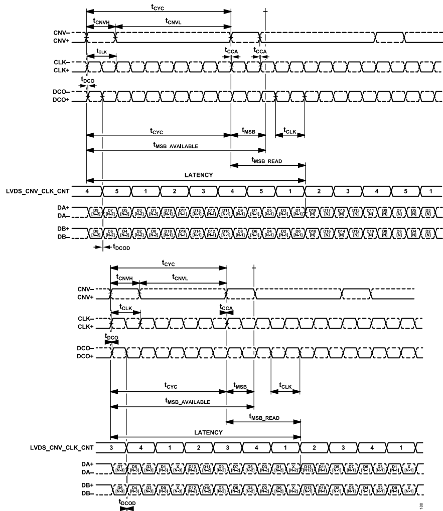
Figure 79. Dual Lane LVDS, Echo Clock Mode, LVDS_CNV_CLK_CNT Position Example
