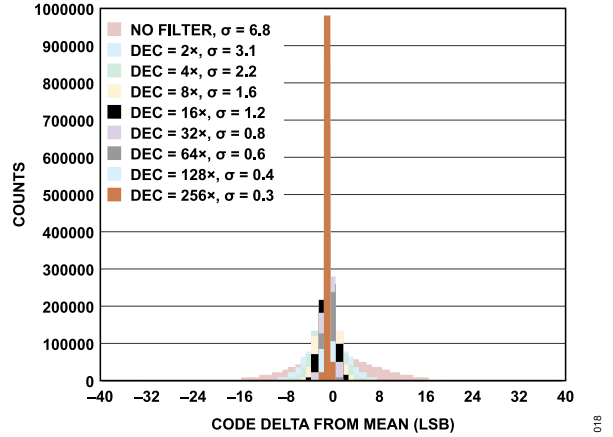
Figure 18. Histogram of Codes, Sinc5, No Filter, Decimate 2x, Decimate 4x ... Decimate 256x
