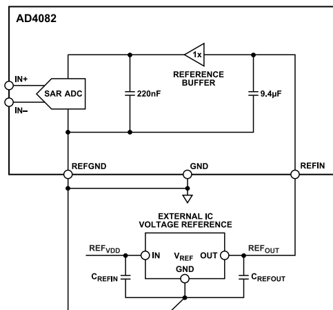
Figure 46. AD4082 General External Reference Design Functional Diagram
