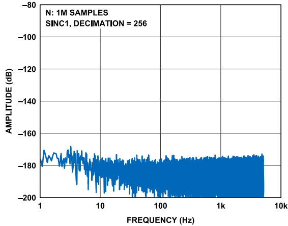
Figure 15. Noise Floor with Shorted Inputs
