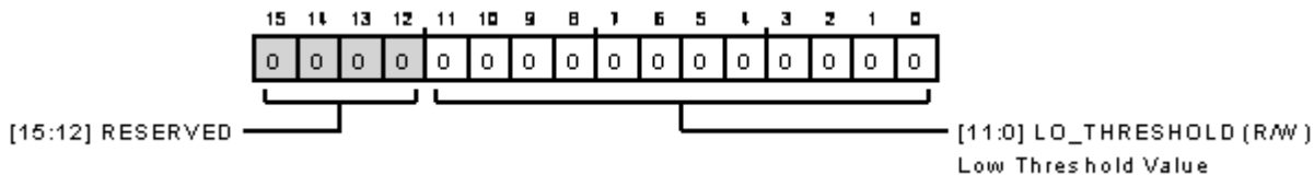
Figure 136. Event Detection Low Threshold Configuration Register
