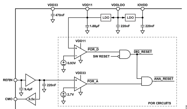
Figure 39. Simplified Diagram of POR Circuit
