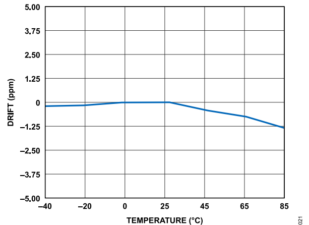
Figure 20. Offset Drift vs. Temperature
