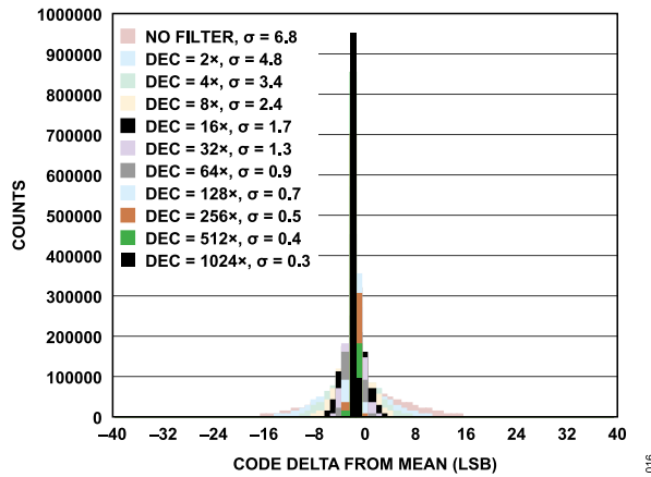
Figure 16. Histogram of Codes, Sinc1 Filter vs. Decimation Rate
