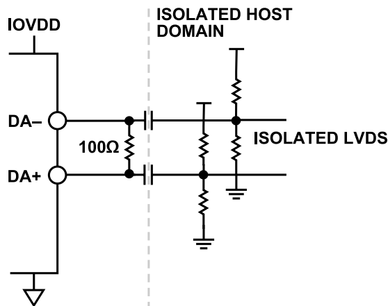
Figure 77. Isolated LVDS
