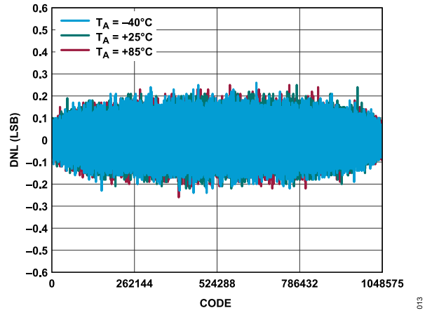
Figure 13. DNL vs. Temperature
