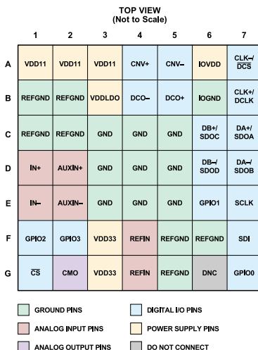
Figure 2. Pin Configuration
