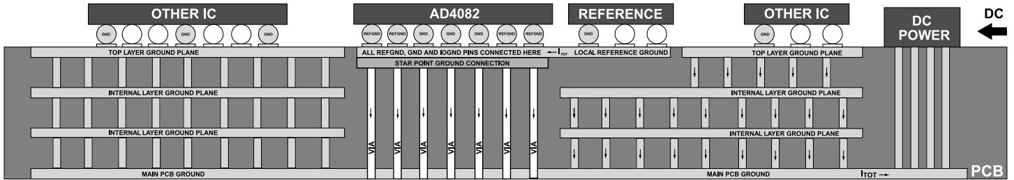
Figure 108. Recommended PCB Ground Planes Layout
