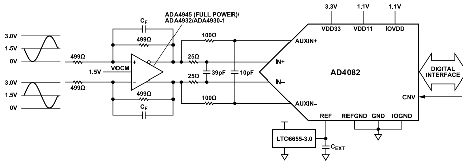
Figure 44. AD4082 Typical Applications Diagram, Fully Differential Amplifier
