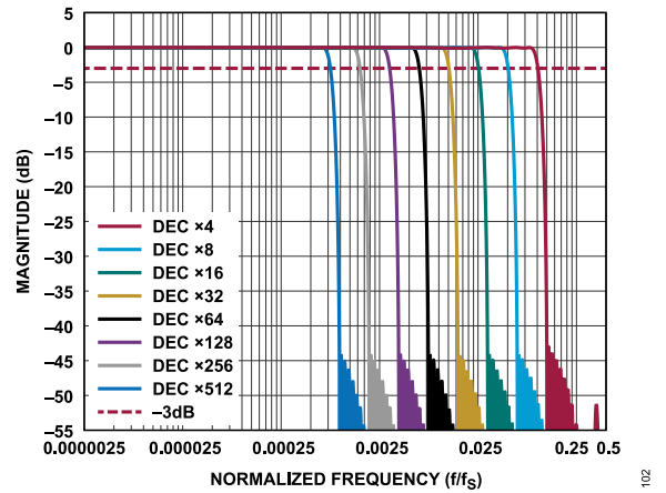
Figure 106. Sinc5 + Compensation Filter Response
