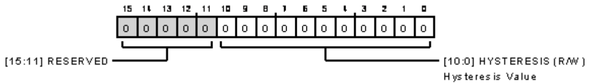
Figure 134. Event Detection Hysteresis Configuration Register
