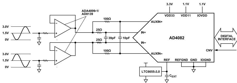
Figure 45. AD4082 Typical Applications Diagram, Single Op-Amp Drivers
