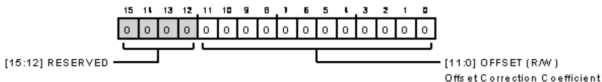
Figure 137. Offset Correction Register
