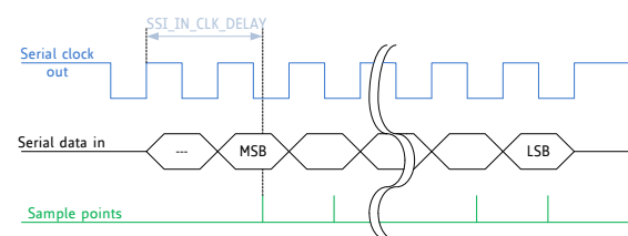
Figure 56: SSI: SSI_IN_CLK_DELAY > SER_CLK_IN_HIGH
