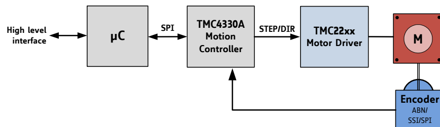
Figure 4: Hardware Set-up for Closed-loop Operation with TMC220x/222x
