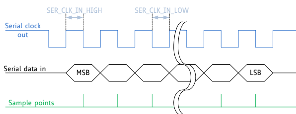
Figure 55: SSI: SSI_IN_CLK_DELAY =0
