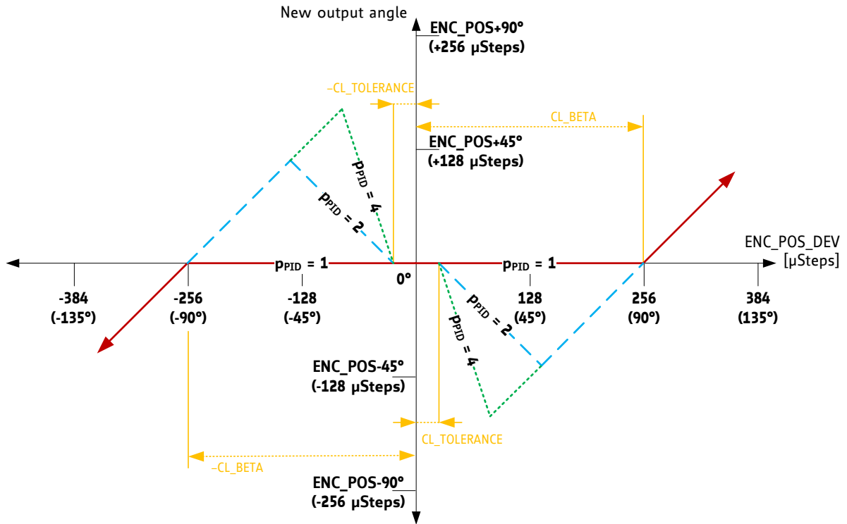
Figure 57: Calculation of the Output Angle with appropriate CL_DELTA_P
