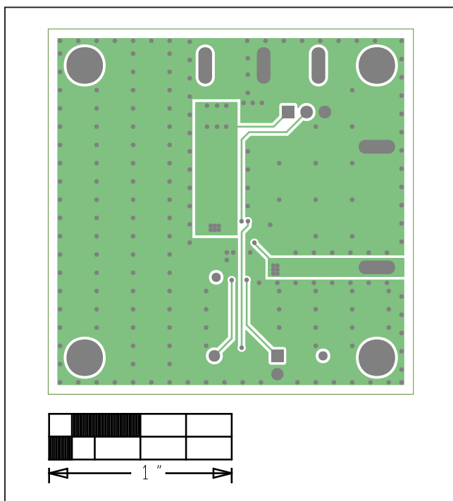
MAXM15463 EV Kit PCB Layout—Layer 3 Power
