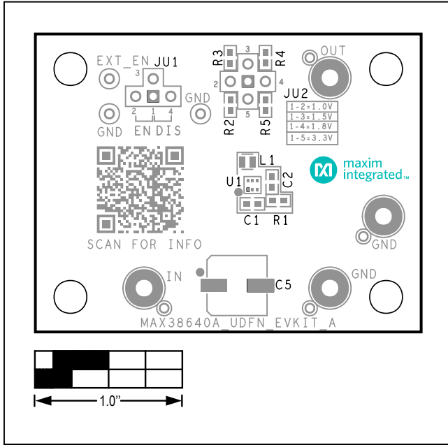
MAX38640A \mu DFN EV Kit—Top Silkscreen
