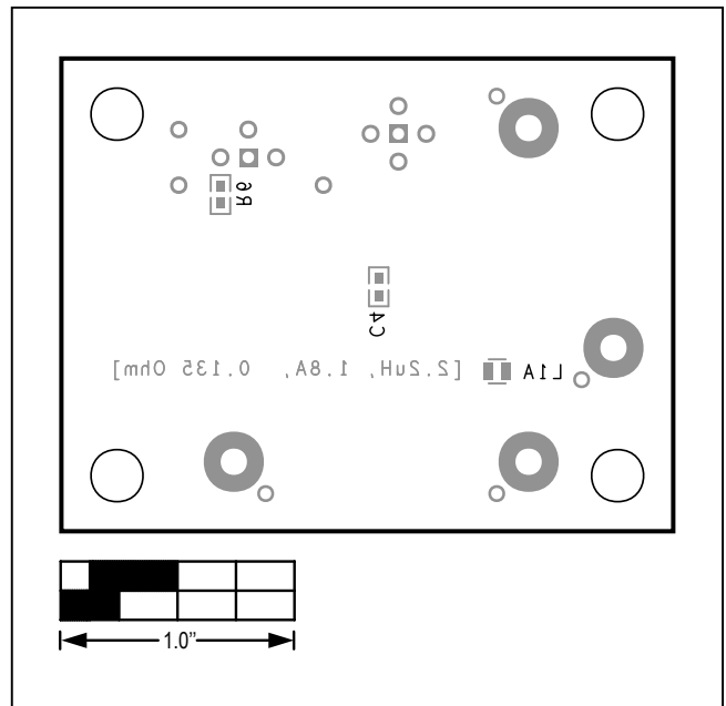
MAX38640A \mu DFN EV Kit—Bottom Silkscreen
