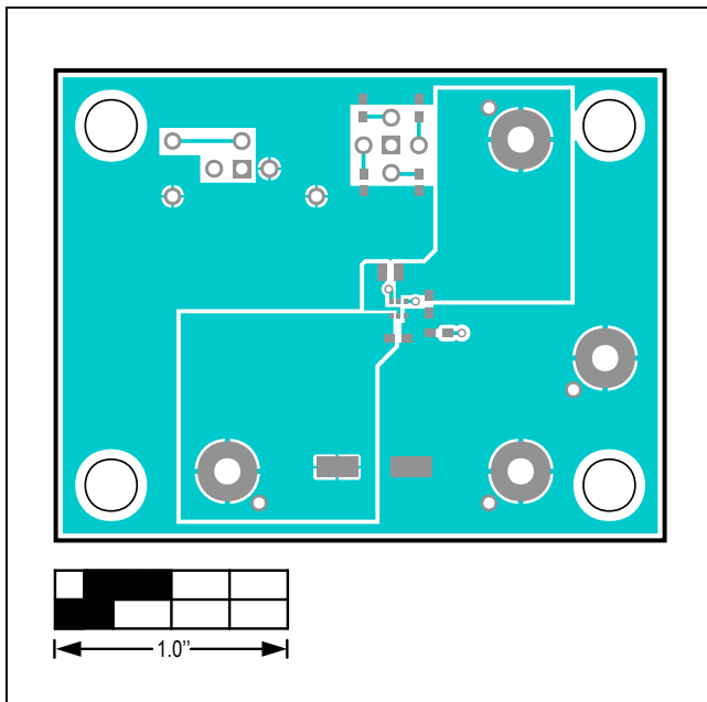
MAX38640A \mu DFN EV Kit—Top
