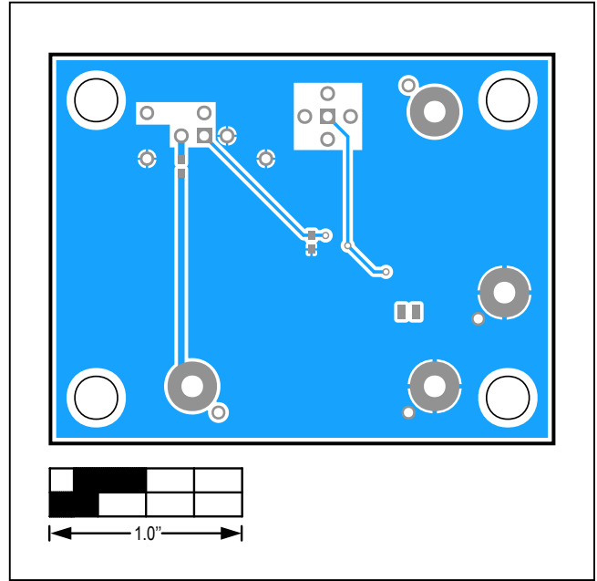
MAX38640A \mu DFN EV Kit—Bottom
