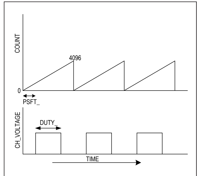
Figure 2. PWM Dimming
