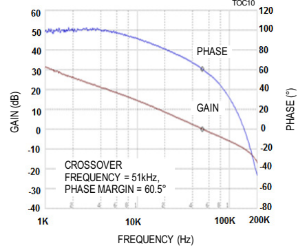
BODE PLOT 3.3V OUTPUT, 5A LOAD CURRENT
