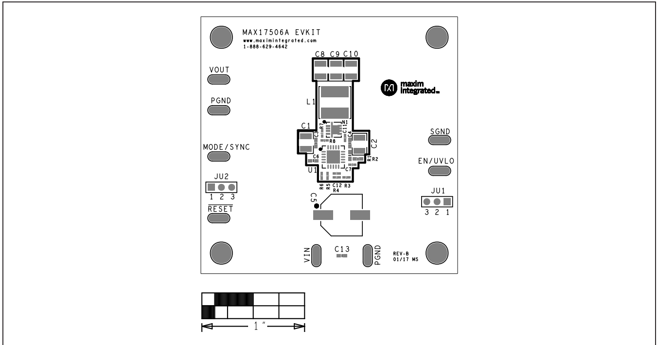
MAX17506 3.3V Output EV Kit PCB Layout—Silk Top
