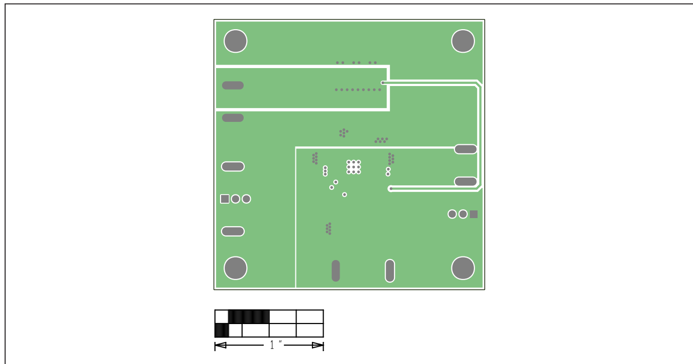
MAX17506 3.3V Output EV Kit PCB Layout—Layer 3 Power
