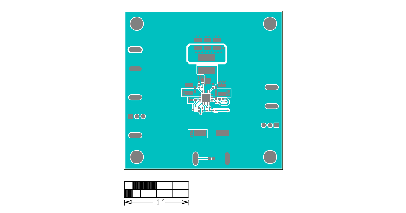
MAX17506 3.3V Output EV Kit PCB Layout—Top Layer
