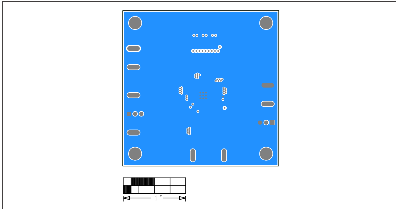
MAX17506 3.3V Output EV Kit PCB Layout—Bottom Layer
