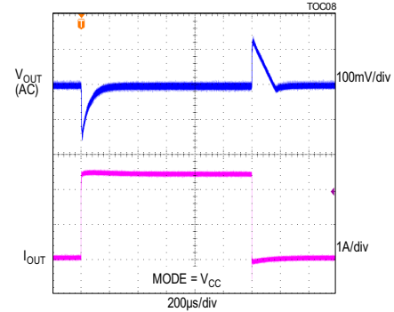
LOAD CURRENT STEPPED FROM 50mA TO 2.5A 3.3V OUTPUT, DCM MODE
