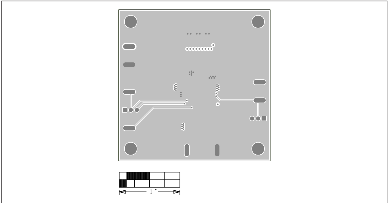
MAX17506 3.3V Output EV Kit PCB Layout—Layer 2 Ground
