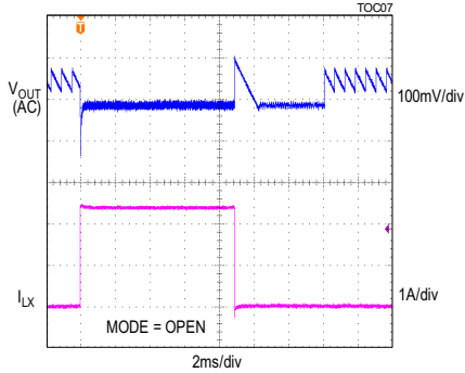
LOAD CURRENT STEPPED FROM 50mA TO 2.5A 3.3V OUTPUT, PFM MODE
