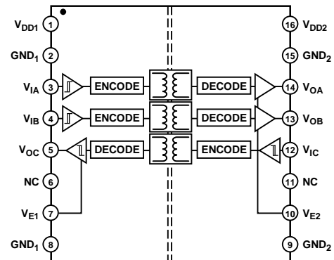
Figure 2. ADuM3301W
