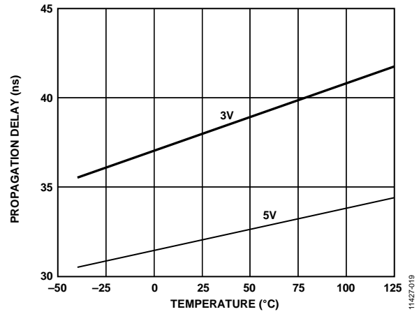
Figure 13. Propagation Delay vs. Temperature, B Grade for 5 V and 3.3 V Operation
