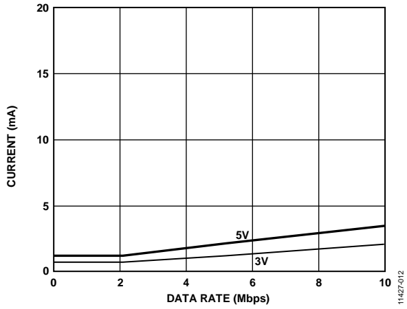
Figure 12. Typical ADuM3301W V_{DD2} Supply Current vs. Data Rate for 5 V and 3.3 V Operation
