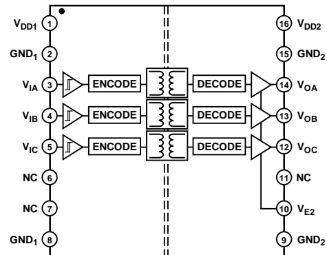
Figure 1. ADuM3300W
