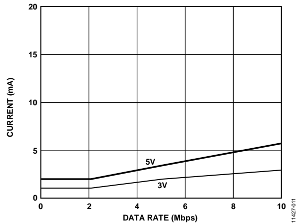
Figure 11. Typical ADuM3301W V_{DD1} Supply Current vs. Data Rate for 5 V and 3.3 V Operation
