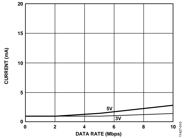
Figure 10. Typical ADuM3300W V_{DD2} Supply Current vs. Data Rate for 5 V and 3.3 V Operation
