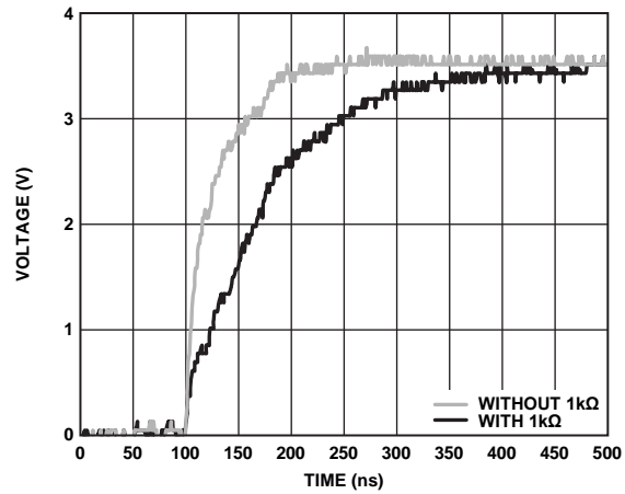
Figure 33. Using a Resistor on SEROUT
