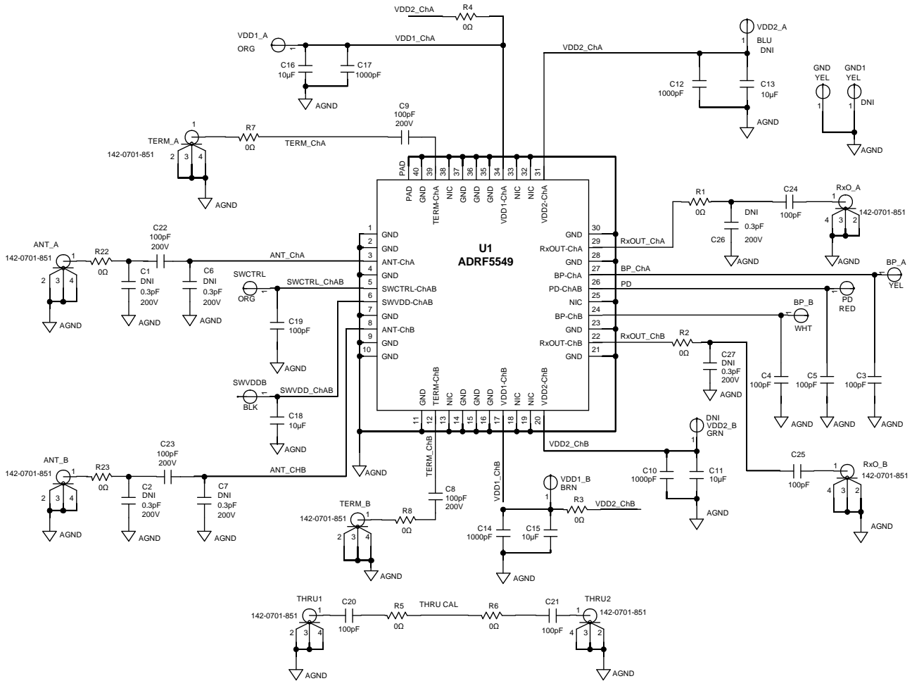
Figure 28. Typical Application Circuit
