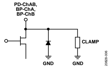
Figure 6. PD-ChAB and BP-Chx Interface Schematic
