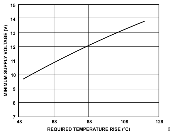
Figure 8. Minimum Supply Voltage vs. Required Temperature Rise
