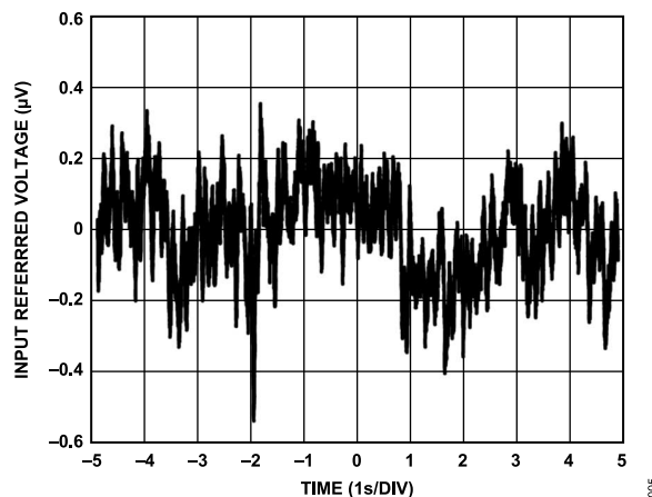
Figure 6. 0.1 Hz to 10 Hz Noise Peak to Peak, I_{CQ1} = 100 \mu A and I_{BZ1} = 5 mA
