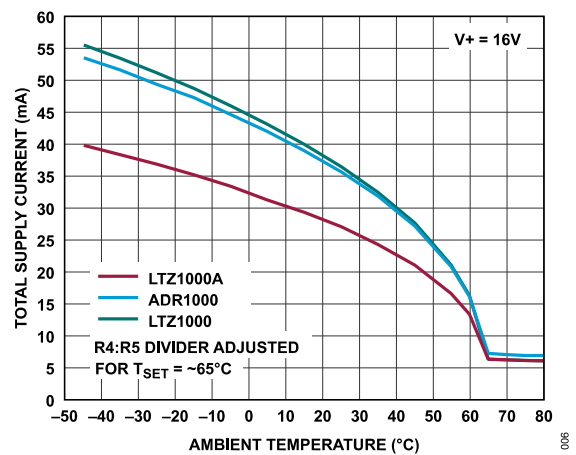
Figure 7. Total Supply Current vs. Ambient Temperature, ADR1000, LTZ1000, and LTZ1000A, Circuit of Figure 9 with R4:R5 Dividers Adjusted for T_{SET} \approx 65^\circ C
