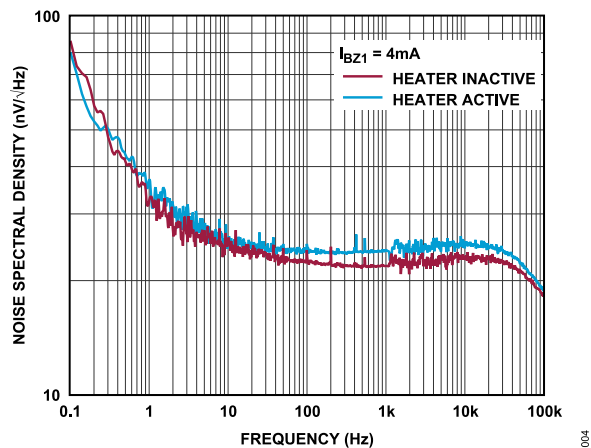
Figure 4. Noise Spectral Density vs. Frequency, Heater Active vs. Inactive, I_{BZ1} = 4 mA , I_{CQ1} = 100 \mu A
