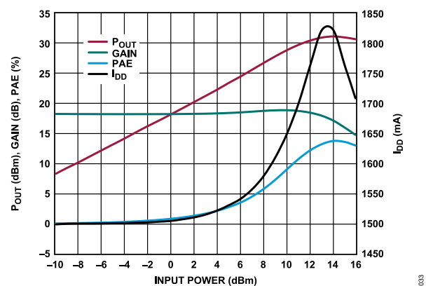
Figure 33. P_{OUT} , Gain, PAE, and Drain Current with RF Applied ( I_{DD} ) vs. Input Power, 22 GHz, V_{DD} = 5 V, I_{DQ} = 1500 mA
