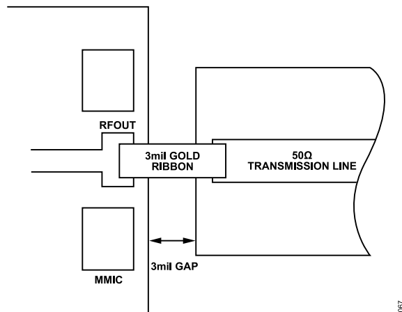
Figure 67. High Frequency Output Wideband Matching
