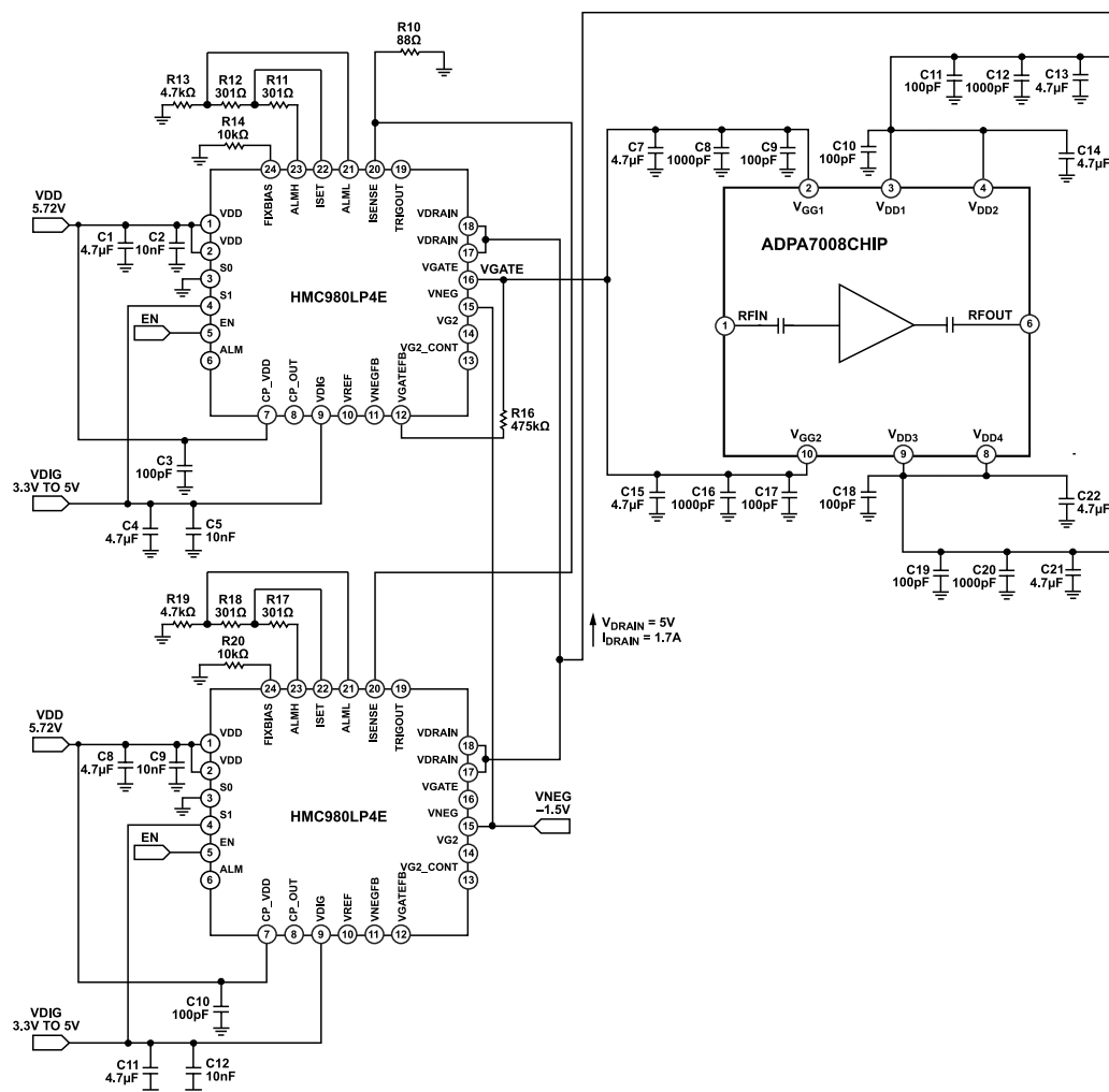
Figure 60. Application Circuit Using HMC980LP4E with ADPA7008CHIP (External Negative Voltage Source)
