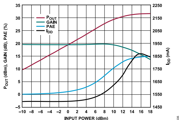
Figure 35. P_{OUT} , Gain, PAE, and I_{DD} vs. Input Power, 36 GHz, V_{DD} = 5 V, I_{DQ} = 1500 mA
