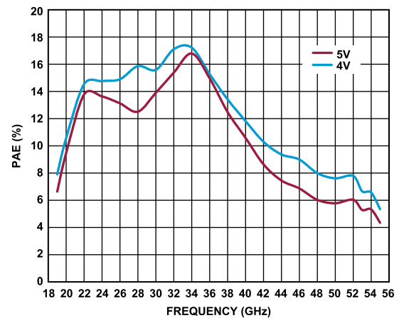
Figure 32. PAE vs. Frequency for Various Supply Voltages, I_{DQ} = 1500 mA, PAE at P_{SAT} (dBm)
