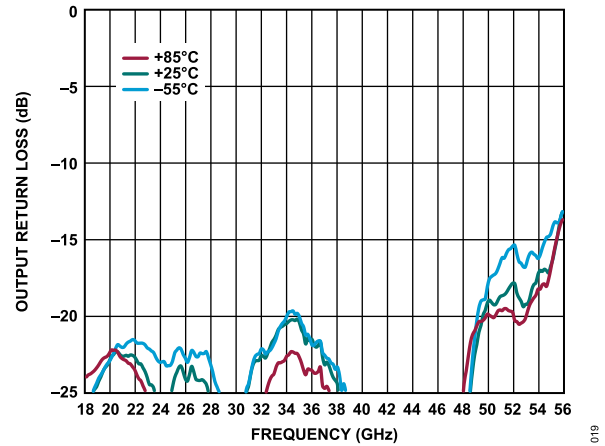
Figure 19. Output Return Loss vs. Frequency for Various Temperatures, V_{DD} = 5\text{ V} , I_{DQ} = 1500\text{ mA}
