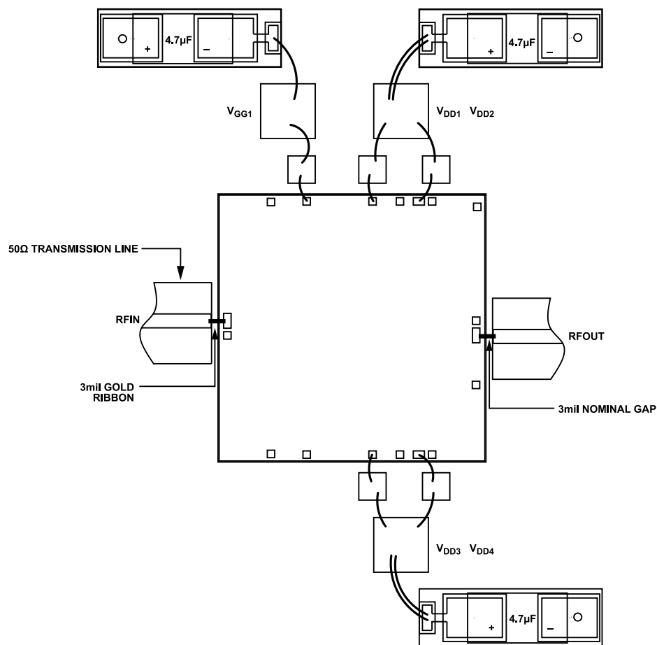
Figure 65. Assembly Diagram
