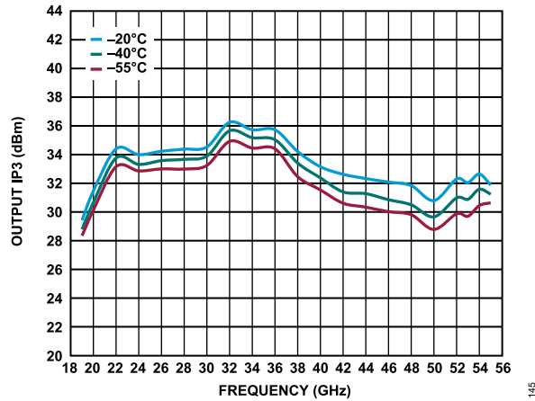
Figure 46. Output IP3 vs. Frequency at -20^{\circ}\text{C} , -40^{\circ}\text{C} , and -55^{\circ}\text{C} , P_{\text{OUT}} per Tone = 14 dBm, V_{\text{DD}} = 5\text{ V} , I_{\text{DQ}} = 1700\text{ mA}
