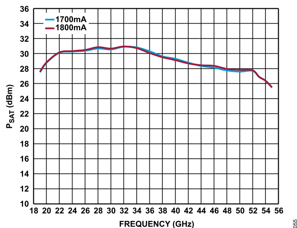
Figure 64. P_{SAT} vs. Frequency for Various Drain Currents, V_{DD} = 5\text{ V} , Data Measured with Constant I_{DD}
