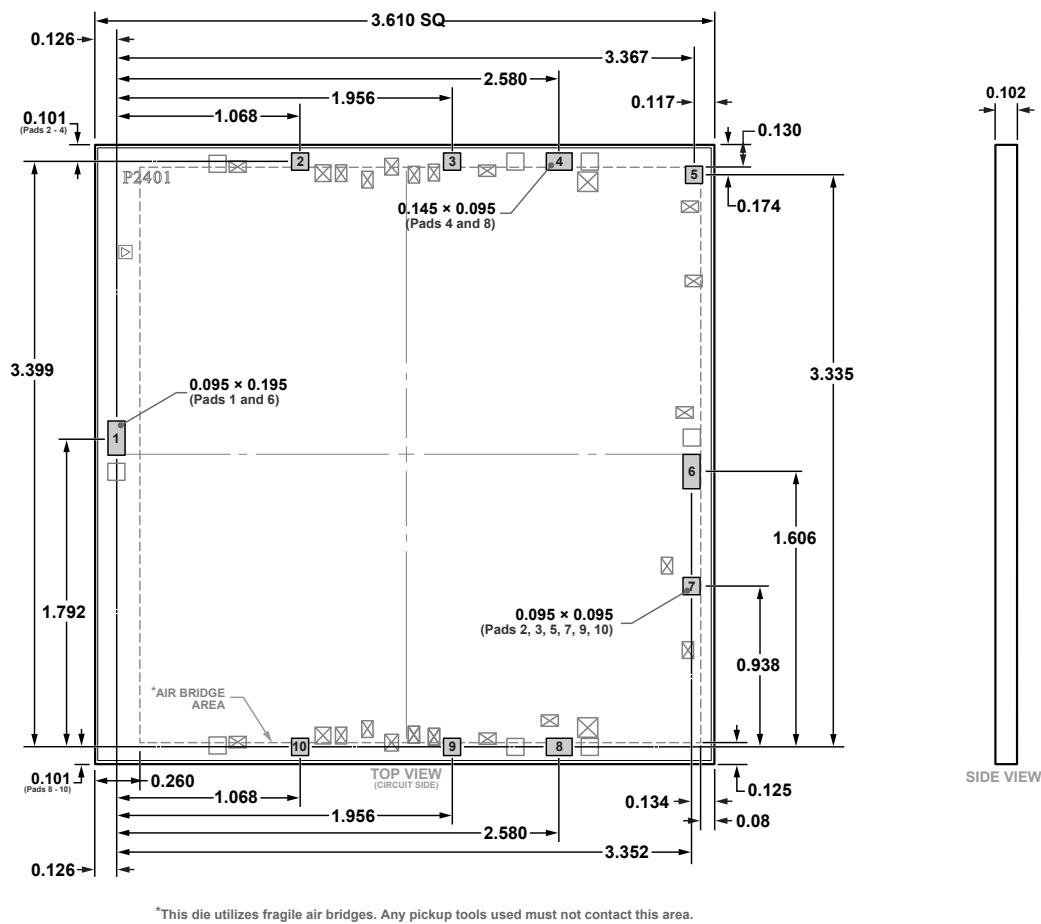
Figure 68. 10-Pad Bare Die [CHIP] (C-10-12) Dimensions shown in millimeters
