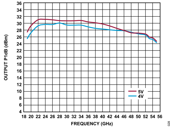
Figure 28. Output P1dB vs. Frequency for Various Supply Voltages, I_{DQ} = 1500 mA
