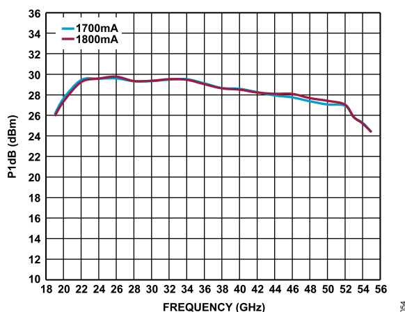
Figure 63. P1dB vs. Frequency for Various Drain Currents, V_{DD} = 5\text{ V} , Data Measured with Constant I_{DD}
