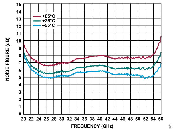
Figure 21. Noise Figure vs. Frequency for Various Temperatures, V_{DD} = 5\text{ V} , I_{DQ} = 1500\text{ mA}
