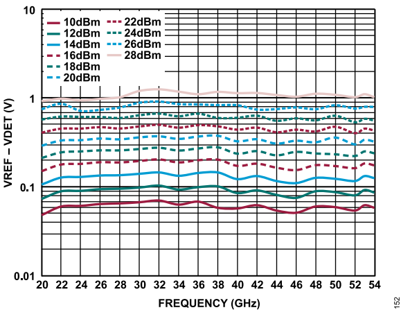
Figure 54. Detector Voltage ( V_{REF} - V_{DET} ) vs. Frequency for Various Output Powers
