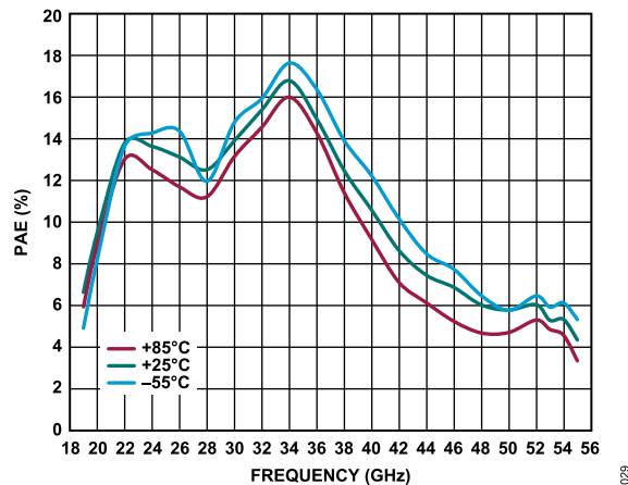
Figure 29. Power Added Efficiency (PAE) vs. Frequency for Various Temperatures, V_{DD} = 5 V, I_{DQ} = 1500 mA, PAE at P_{SAT} (dBm)
