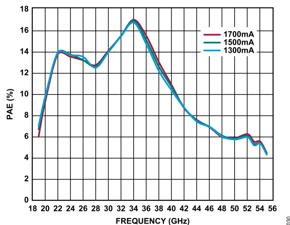
Figure 30. PAE vs. Frequency for Various Supply Currents, V_{DD} = 5 V, PAE at P_{SAT} (dBm)
