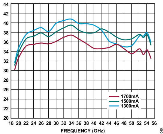
Figure 47. Output IP3 vs. Frequency for Various Supply Currents, P_{\text{OUT}} per Tone = 14 dBm, V_{\text{DD}} = 5\text{ V}
