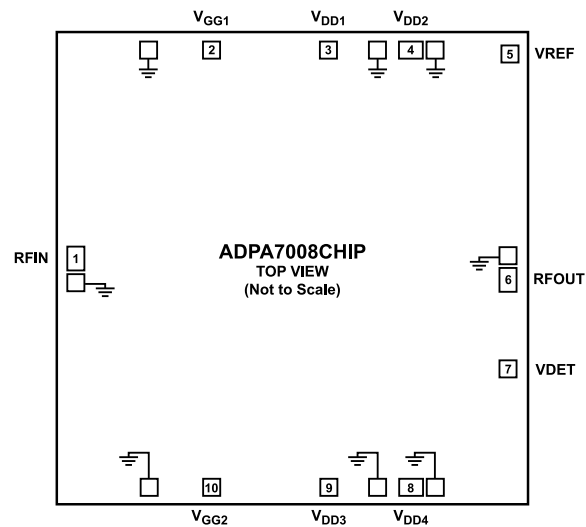
Figure 2. Pin Configuration
