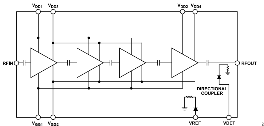
Figure 55. ADPA7008CHIP Architecture
