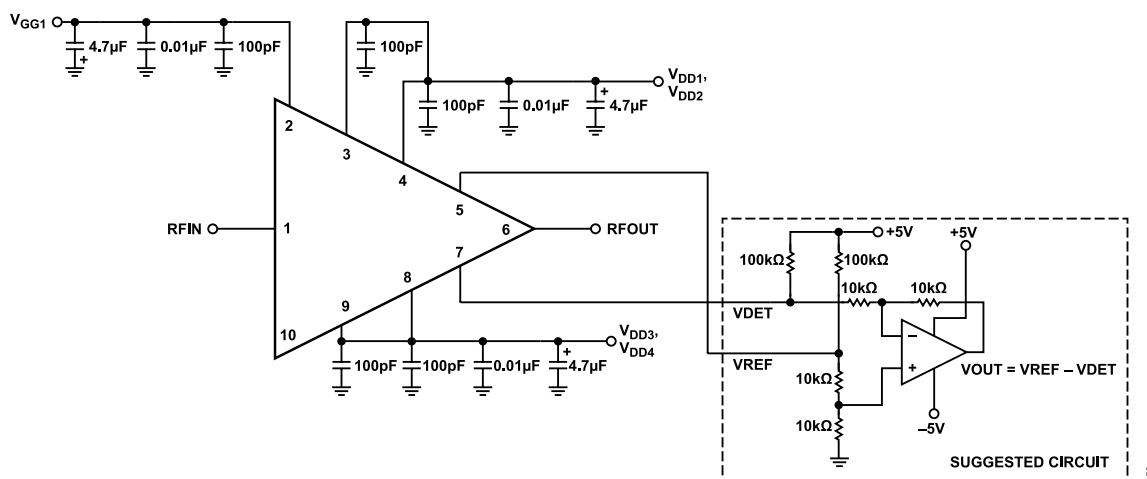
Figure 56. Primary Application Circuit
