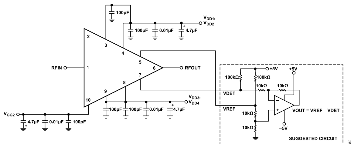
Figure 57. Alternate Application Circuit
