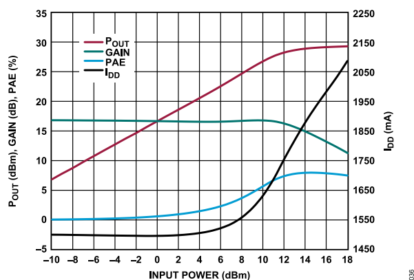
Figure 36. P_{OUT} , Gain, PAE, and I_{DD} vs. Input Power, 44 GHz, V_{DD} = 5 V, I_{DQ} = 1500 mA
