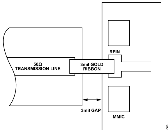
Figure 66. High Frequency Input Wideband Matching
