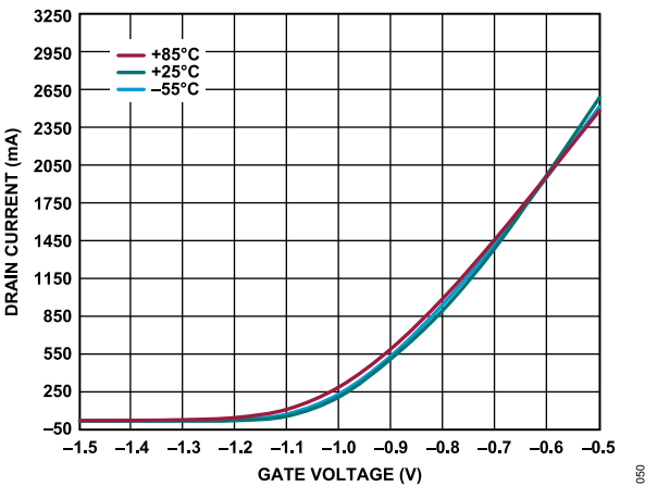
Figure 52. Drain Current vs. Gate Voltage for Various Temperatures, V_{DD} = 5\text{ V} , I_{DQ} = 1500\text{ mA}
