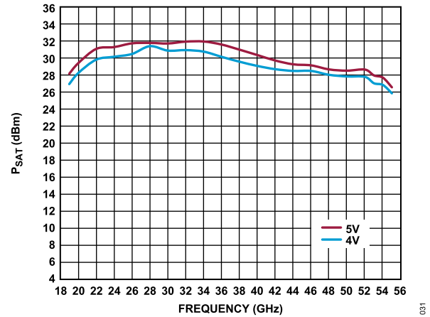
Figure 31. P_{SAT} vs. Frequency for Various Voltages, I_{DQ} = 1500 mA
