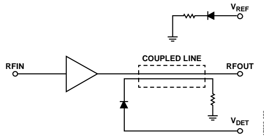
Figure 56. Power Detector Circuit
