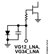
Figure 6. VG12_LNA and VG34_LNA Interface Schematic
