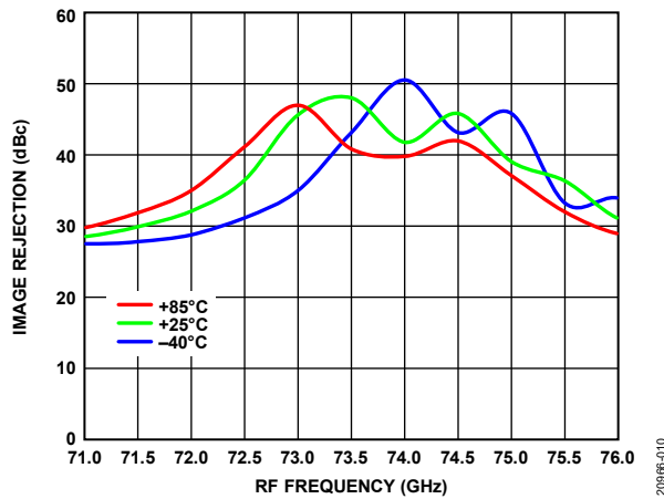
Figure 10. Image Rejection vs. RF Frequency over Temperature
