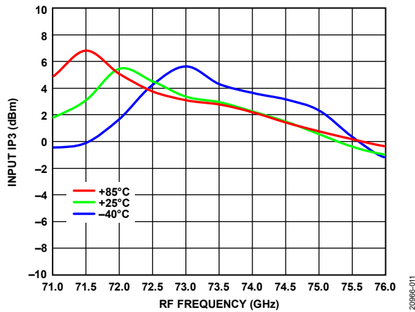
Figure 11. Input IP3 vs. RF Frequency over Temperature
