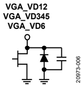
Figure 6. VGA_VD12, VGA_VD345, and VGA_VD6 Interface Schematic
