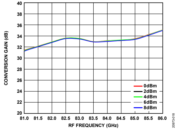
Figure 18. Maximum Conversion Gain vs. RF Frequency over LO Power, IF Input Power = -20 dBm
