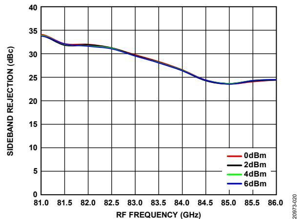
Figure 20. Sideband Rejection vs. RF Frequency over LO Power, Gain = 23.5 dB
