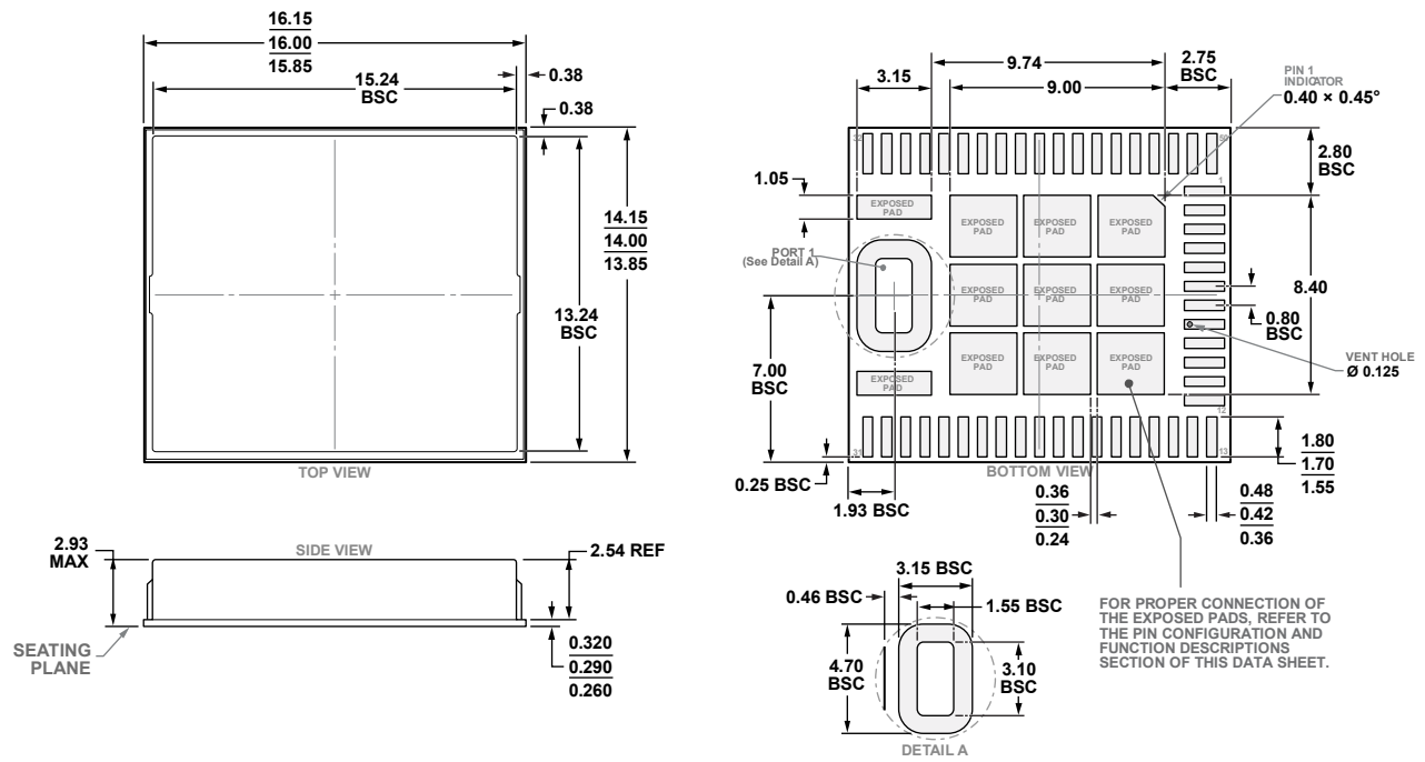
Figure 87. 50-Terminal Chip Array Small Outline No Lead Cavity [LGA_CAV] 16.00 mm × 14.00 mm Body and 2.93 mm Package Height (CE-50-2) Dimensions shown in millimeters
