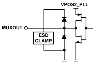
Figure 9. MUXOUT Interface Schematic
