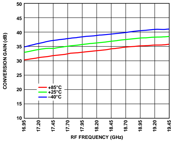
Figure 40. Conversion Gain vs. RF Frequency at Various Temperatures
