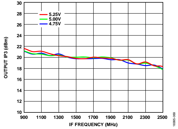
Figure 71. Output IP3 vs. IF Frequency at Various Supply Voltages, T A = 25°C
