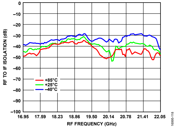
Figure 120. RF to IF Leakage vs. RF Frequency at Various Temperatures for Low-Side Injection LO, IF = 900 MHz
