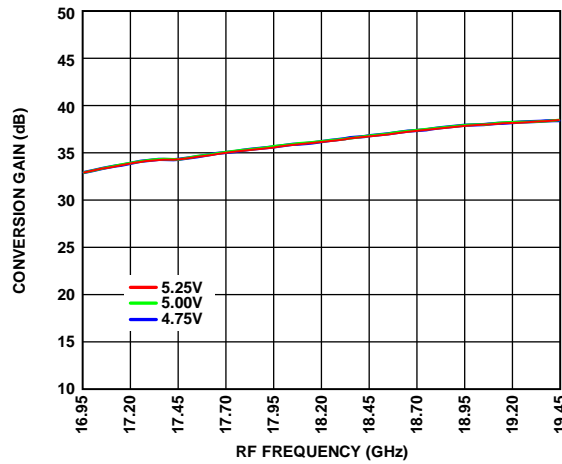
Figure 43. Conversion Gain vs. RF Frequency at Various Supply Voltages, T_A = 25^\circ\text{C}
