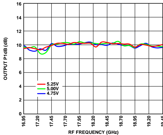
Figure 45. Output P1dB vs. RF Frequency at Various Supply Voltages, T_A = 25^\circ\text{C}
