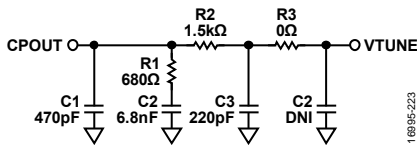
Figure 124. Recommended Loop Filter Schematic
