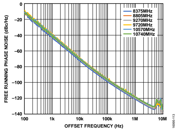
Figure 115. Free Running Phase Noise vs. Offset Frequency at Various VCO Frequencies, T_A = 25^\circ\text{C}
