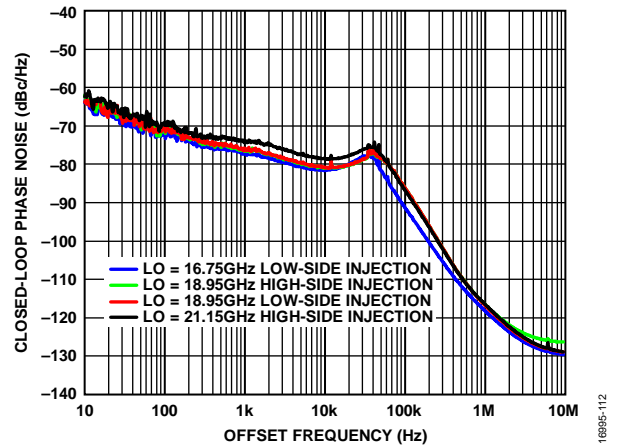
Figure 114. Closed-Loop Phase Noise vs. Offset Frequency at Various LO Frequencies, T_A = 25^\circ\text{C}
