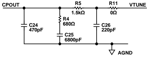
Figure 131. Recommended Integer Mode Loop Filter Schematic
