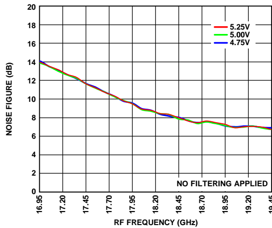
Figure 44. Noise Figure vs. RF Frequency at Various Supply Voltages, T_A = 25^\circ\text{C}
