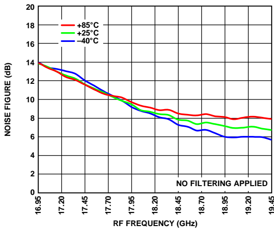
Figure 41. Noise Figure vs. RF Frequency at Various Temperatures
