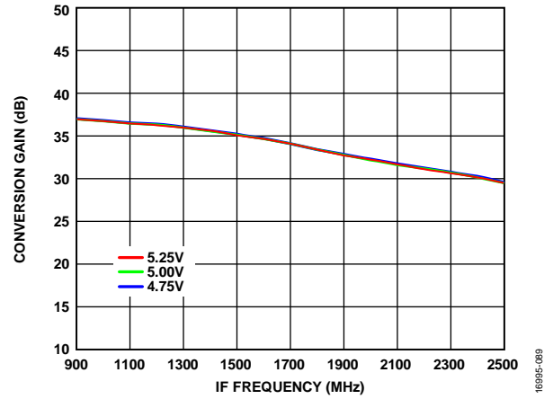
Figure 91. Conversion Gain vs. IF Frequency at Various Supply Voltages, T_A = 25^\circ\text{C}
