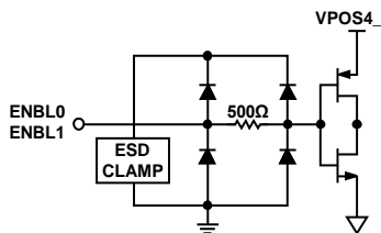
Figure 10. ENBL0 and ENBL1 Interface Schematic
