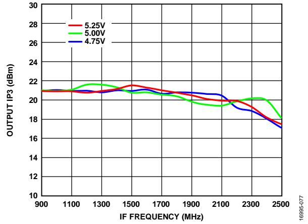
Figure 79. Output IP3 vs. IF Frequency at Various Supply Voltages, T A = 25°C
