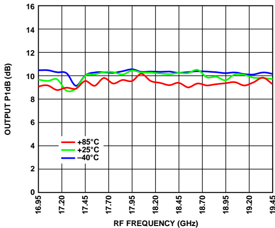
Figure 42. Output P1dB vs. RF Frequency at Various Temperatures
