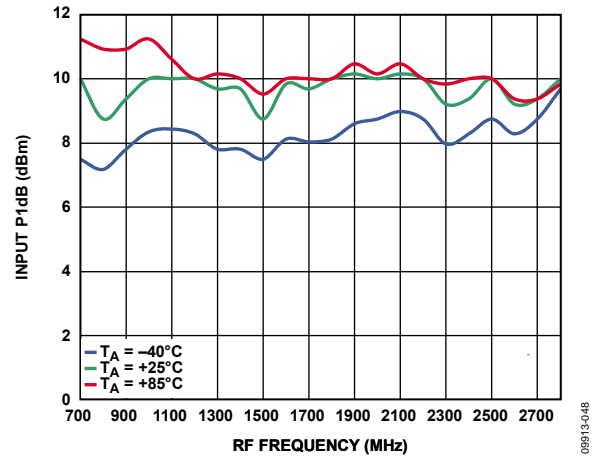
Figure 57. Input P1dB vs. RF Frequency at 3.6 V
