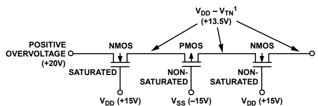
Figure 22. Positive Overvoltage on the Channel Protector
