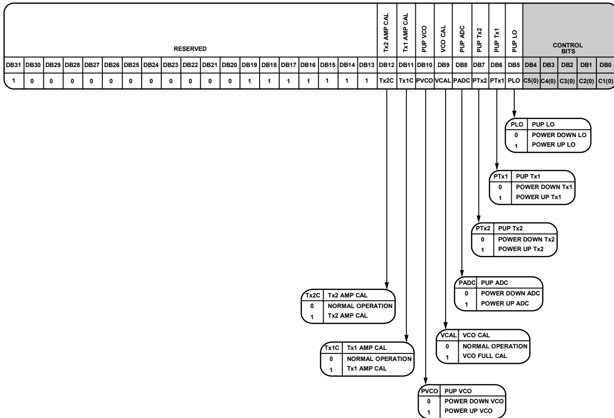
Figure 24. Register 0 (R0)
