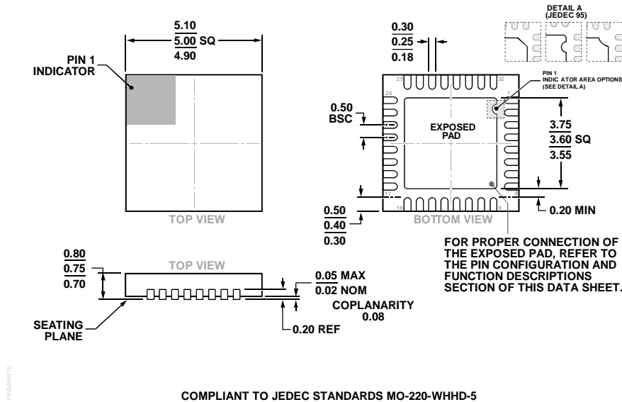
COMPLIANT TO JEDEC STANDARDS MO-220-WHHD-5 Figure 54. 32-Lead Lead Frame Chip Scale Package [LFCSP] 5 mm × 5 mm Body and 0.75 mm Package Height (CP-32-12)
