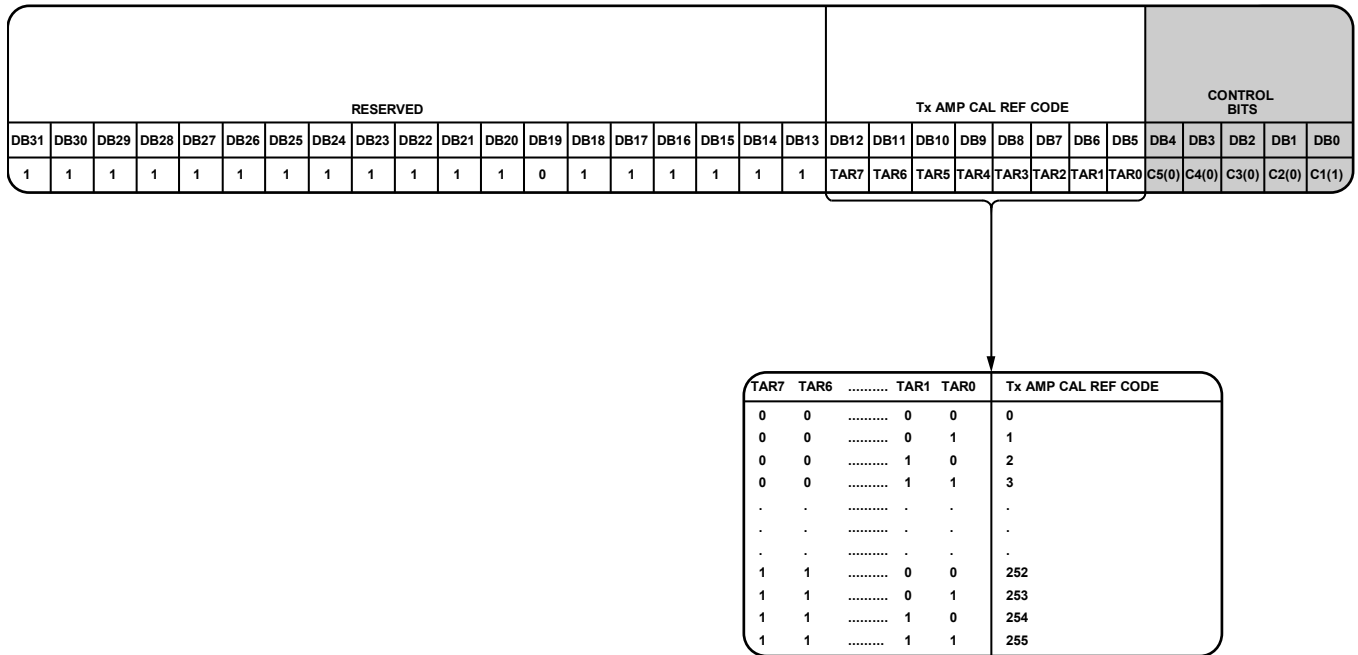
Figure 25. Register 1 (R1)
