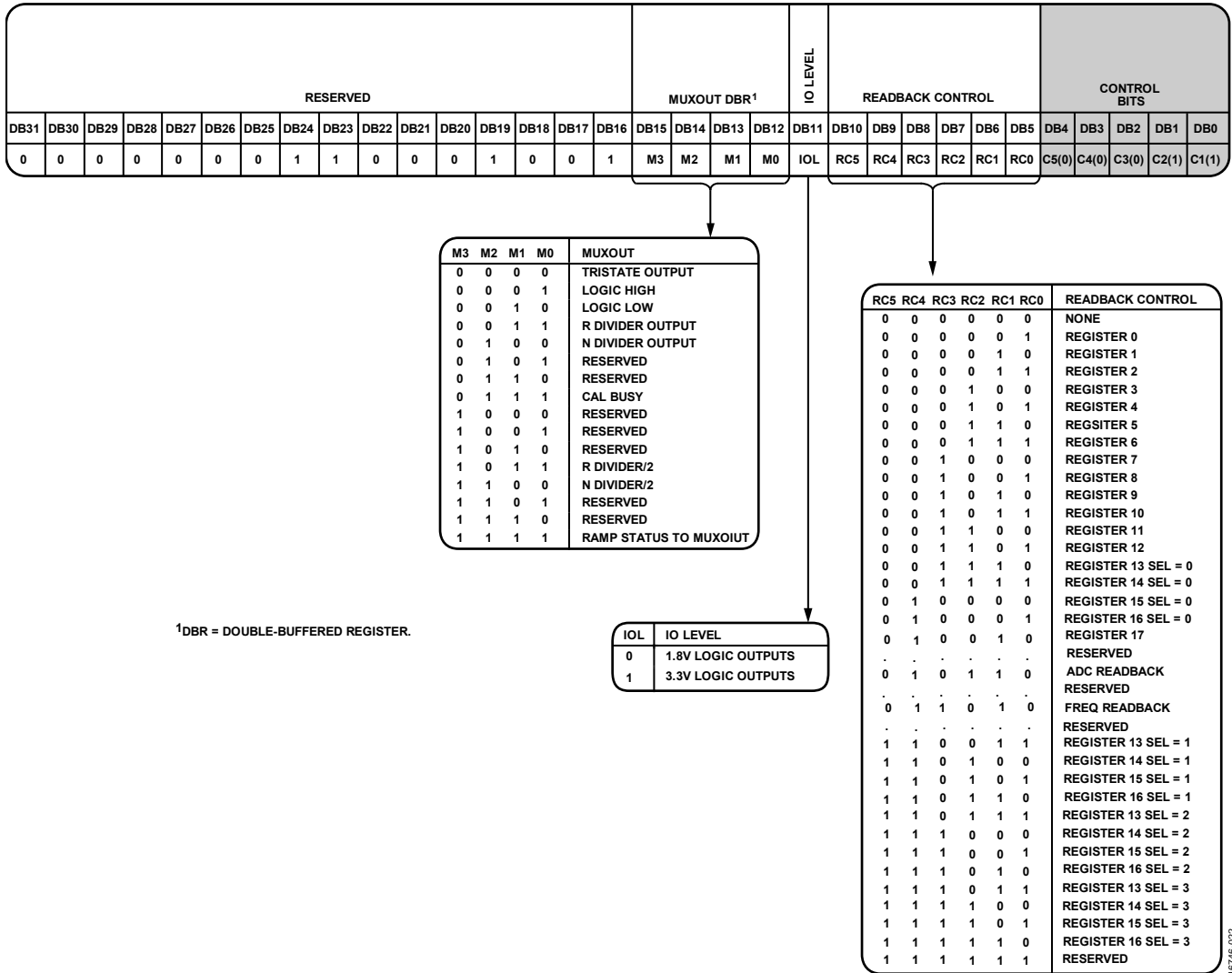
Figure 27. Register 3 (R3)
