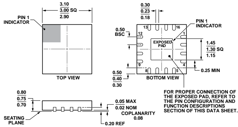
Figure 68. 16-Lead Lead Frame Chip Scale Package [LFCSP] 3 mm × 3 mm Body and 0.75 mm Package Height (CP-16-21) Dimensions shown in millimeters
