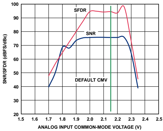
Figure 18. SNR/SFDR vs. Analog Input Common-Mode Voltage, A_{IN} = 100 \text{ MHz} , 2.5 V p-p FS
