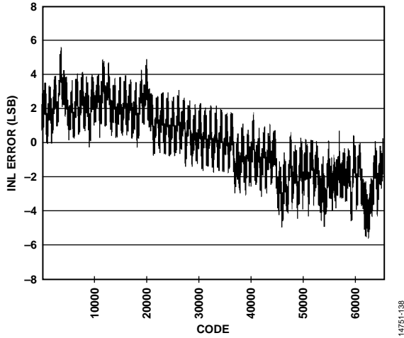
Figure 16. INL, f_{IN} = 4.3 \text{ MHz} , 2.5 V p-p FS
