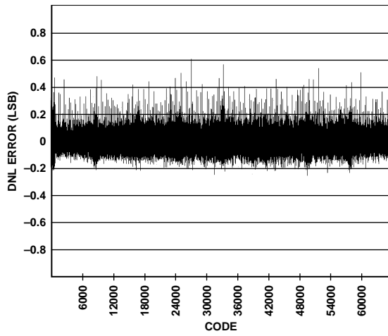
Figure 17. DNL, f_{IN} = 4.3 \text{ MHz} , 2.5 V p-p FS
