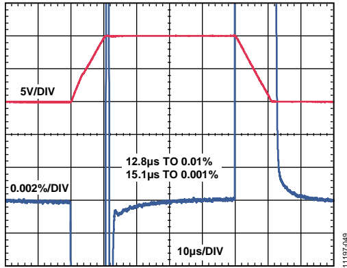
Figure 47. Large Signal Pulse Response and Settling Time ( G = 10 ), 10 V Step, V_s = \pm 15\text{ V} , R_L = 2\text{ k}\Omega , C_L = 100\text{ pF}
