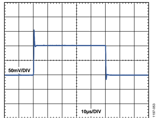
Figure 51. Small Signal Pulse Response ( G = 1 ), R_L = 2\text{ k}\Omega , C_L = 100\text{ pF}
