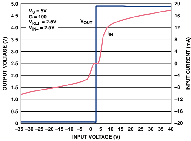
Figure 17. Input Overvoltage Performance; G = 100 , V_S = 5V
