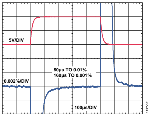
Figure 49. Large Signal Pulse Response and Settling Time ( G = 1000 ), 10 V Step, V_s = \pm 15\text{ V} , R_L = 2\text{ k}\Omega , C_L = 100\text{ pF}
