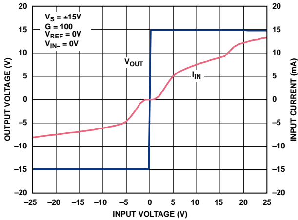
Figure 18. Input Overvoltage Performance; G = 100 , V_S = \pm 15V
