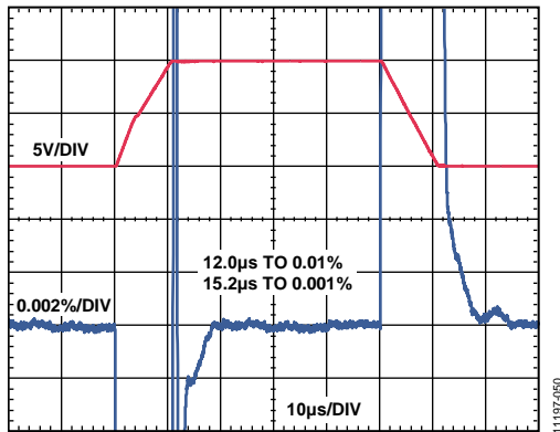
Figure 48. Large Signal Pulse Response and Settling Time ( G = 100 ), 10 V Step, V_s = \pm 15\text{ V} , R_L = 2\text{ k}\Omega , C_L = 100\text{ pF}
