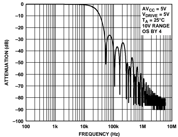
Figure 55. Digital Filter Response for OS x 4
