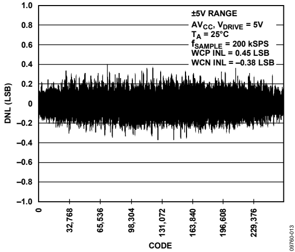
Figure 14. Typical DNL, ±5V Range
