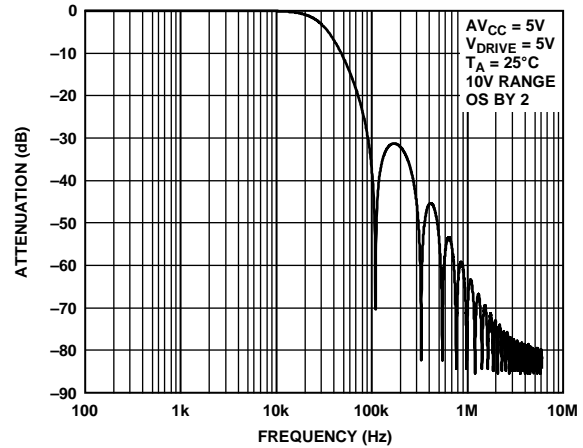
Figure 54. Digital Filter Response for OS x 2
