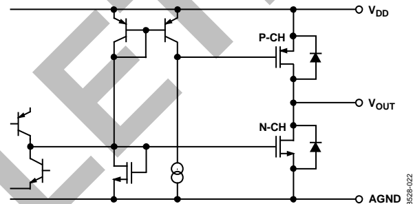
Figure 19. Equivalent Analog Output Circuit
