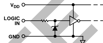
Figure 21. Equivalent Digital Input ESD Protection
