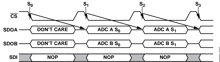
Figure 37. Reading Conversion Results for 2-Wire Mode
