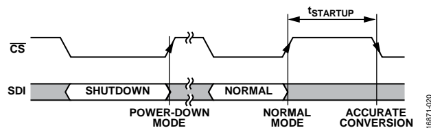
Figure 35. Shutdown Mode Operation
