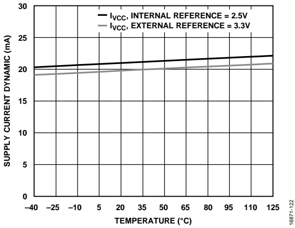
Figure 22. Supply Current Dynamic vs. Temperature
