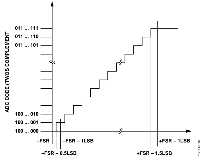
Figure 30. ADC Ideal Transfer Function (FSR = Full-Scale Range)
