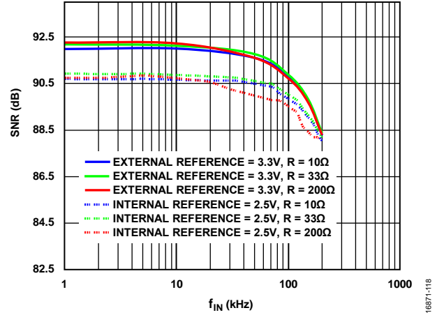
Figure 18. SNR vs. f_{IN}
