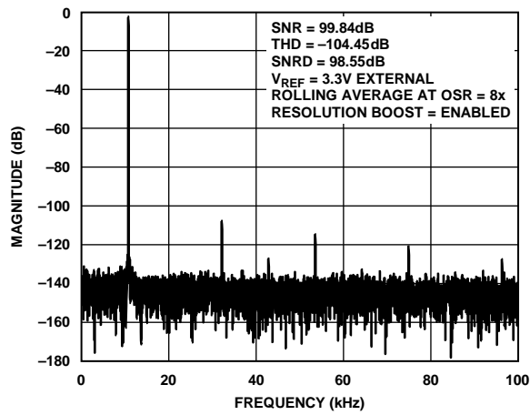
Figure 11. FFT with Oversampling
