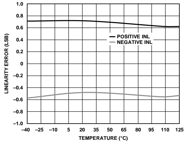
Figure 14. Linearity Error vs. Temperature
