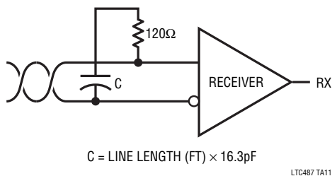
Figure 10. AC-Coupled Termination
