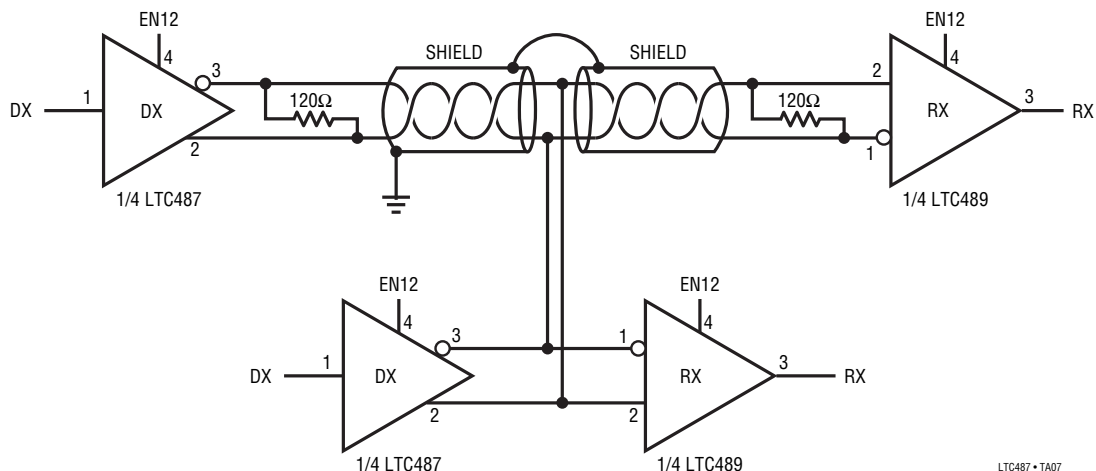
Figure 6. Typical Connection
