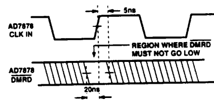
Figure 1. \overline{DMRD} Asynchronous Timing Constraint
