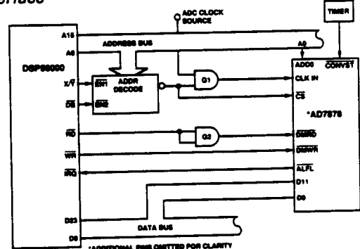
Figure 5. DSP56000-AD7878 Asynchronous Clock Interface
