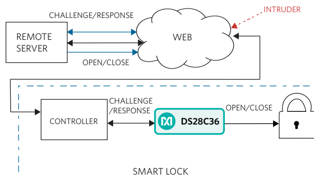
Figure 2. Secure remote lock opening/closing using the DS28C36
