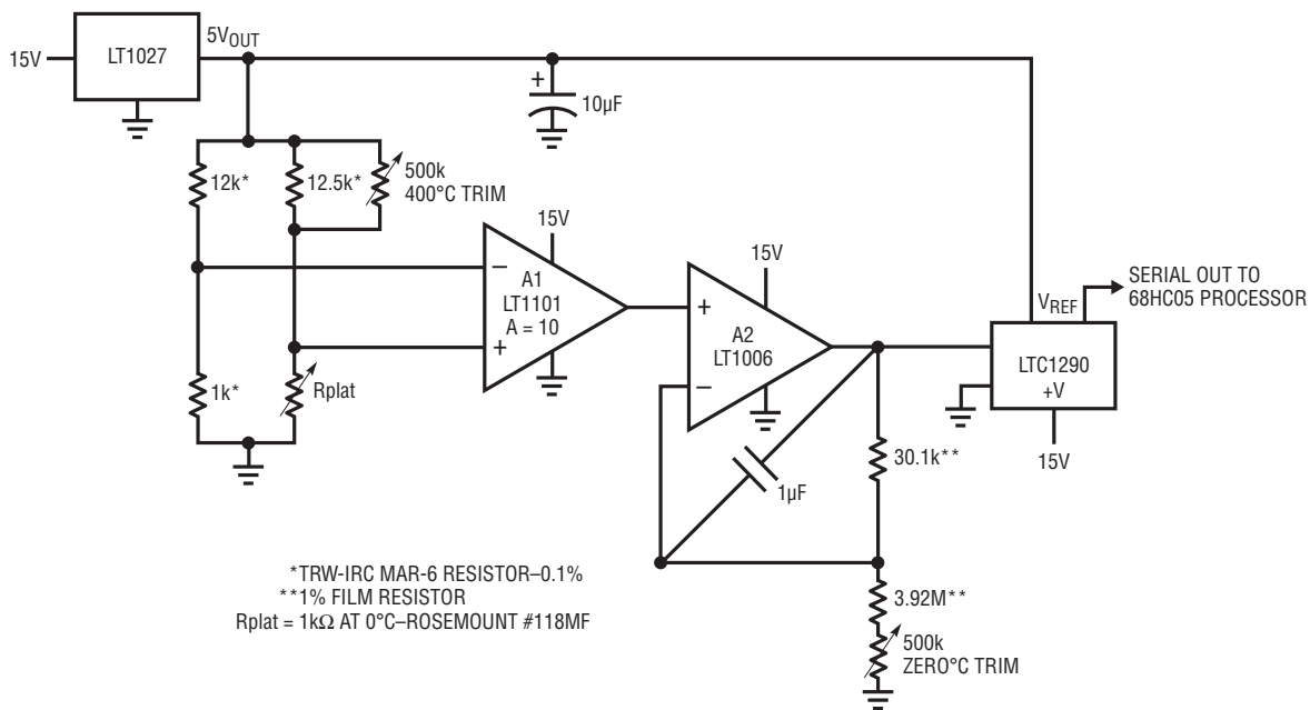
Figure 2. Digitally Linearized Platinum RTD Signal Conditioner
