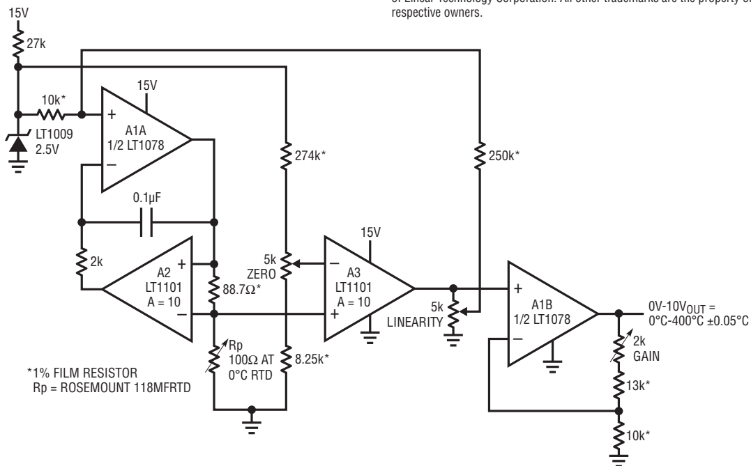
Figure 1. Linearized Platinum RTD Bridge. Feedback to Bridge from A3 Linearizes the Circuit
