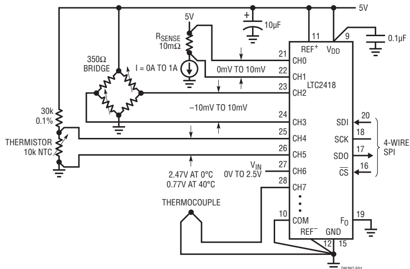
Figure 1. Multiple Measurements with the LTC2418
