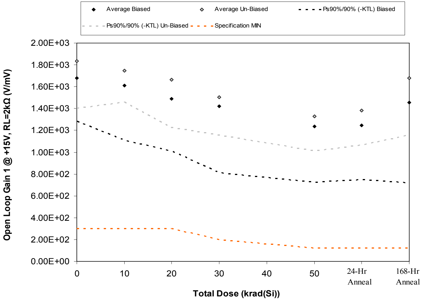
Figure 5.49. Plot of Open Loop Gain 1 @ +15V, RL=2kΩ (V/mV) versus total dose. The solid diamonds are the average of the measured data points for the samples irradiated under electrical bias while the shaded diamonds are the average of the measured data points for the samples irradiated with all pins tied to ground. The black lines (solid and/or dashed) are the average of the data points after application of the KTL statistics on the samples irradiated under electrical bias while the gray lines (solid and/or dashed) are the average of the data points after application of the KTL statistics on the samples irradiated in the unbiased condition. The red dotted line(s) are the pre- and/or post-irradiation minimum and/or maximum specification value as defined in the datasheet and/or test plan.
