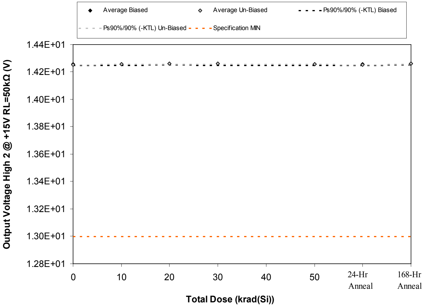
Figure 5.52. Plot of Output Voltage High 2 @ +15V RL=50kΩ (V) versus total dose. The solid diamonds are the average of the measured data points for the samples irradiated under electrical bias while the shaded diamonds are the average of the measured data points for the samples irradiated with all pins tied to ground. The black lines (solid and/or dashed) are the average of the data points after application of the KTL statistics on the samples irradiated under electrical bias while the gray lines (solid and/or dashed) are the average of the data points after application of the KTL statistics on the samples irradiated in the unbiased condition. The red dotted line(s) are the pre- and/or post-irradiation minimum and/or maximum specification value as defined in the datasheet and/or test plan.
