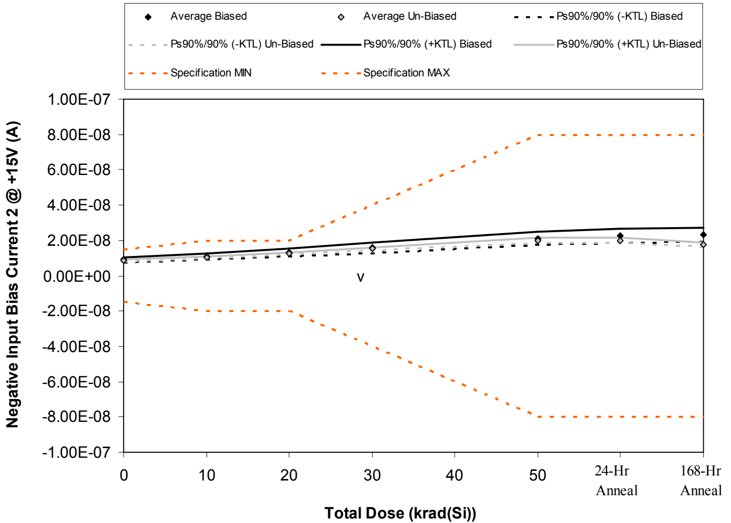
Figure 5.42. Plot of Negative Input Bias Current 2 @ +15V (A) versus total dose. The solid diamonds are the average of the measured data points for the samples irradiated under electrical bias while the shaded diamonds are the average of the measured data points for the samples irradiated with all pins tied to ground. The black lines (solid and/or dashed) are the average of the data points after application of the KTL statistics on the samples irradiated under electrical bias while the gray lines (solid and/or dashed) are the average of the data points after application of the KTL statistics on the samples irradiated in the unbiased condition. The red dotted line(s) are the pre- and/or post-irradiation minimum and/or maximum specification value as defined in the datasheet and/or test plan.
