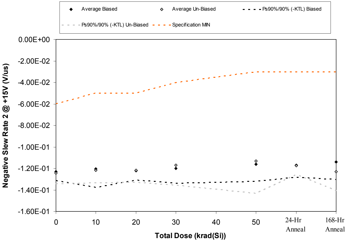
Figure 5.62. Plot of Negative Slew Rate 2 @ +15V (V/us) versus total dose. The solid diamonds are the average of the measured data points for the samples irradiated under electrical bias while the shaded diamonds are the average of the measured data points for the samples irradiated with all pins tied to ground. The black lines (solid and/or dashed) are the average of the data points after application of the KTL statistics on the samples irradiated under electrical bias while the gray lines (solid and/or dashed) are the average of the data points after application of the KTL statistics on the samples irradiated in the unbiased condition. The red dotted line(s) are the pre- and/or post-irradiation minimum and/or maximum specification value as defined in the datasheet and/or test plan.
