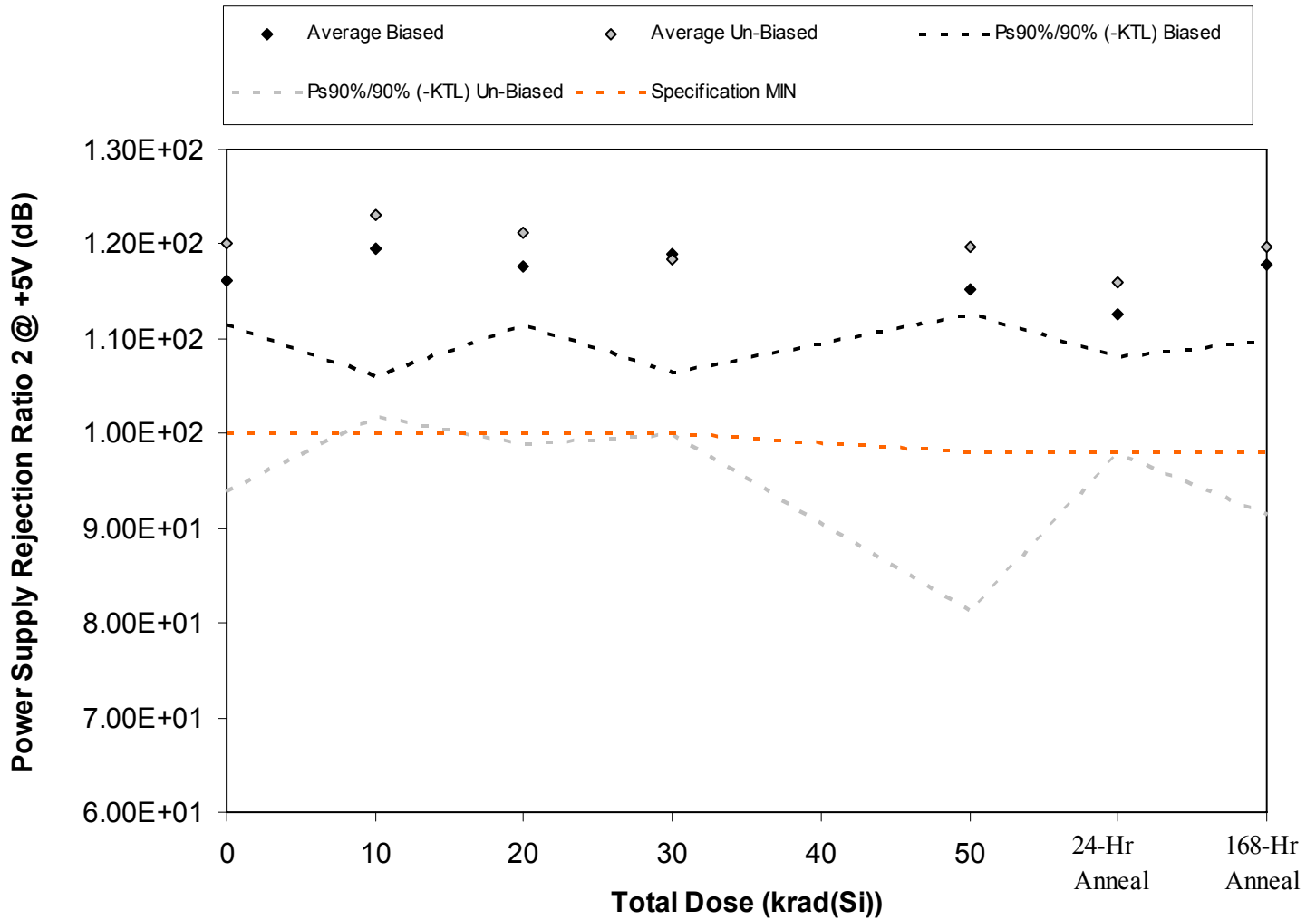
Figure 5.14. Plot of Power Supply Rejection Ratio 2 @ +5V (dB) versus total dose. The solid diamonds are the average of the measured data points for the samples irradiated under electrical bias while the shaded diamonds are the average of the measured data points for the samples irradiated with all pins tied to ground. The black lines (solid and/or dashed) are the average of the data points after application of the KTL statistics on the samples irradiated under electrical bias while the gray lines (solid and/or dashed) are the average of the data points after application of the KTL statistics on the samples irradiated in the unbiased condition. The red dotted line(s) are the pre- and/or post-irradiation minimum and/or maximum specification value as defined in the datasheet and/or test plan.
