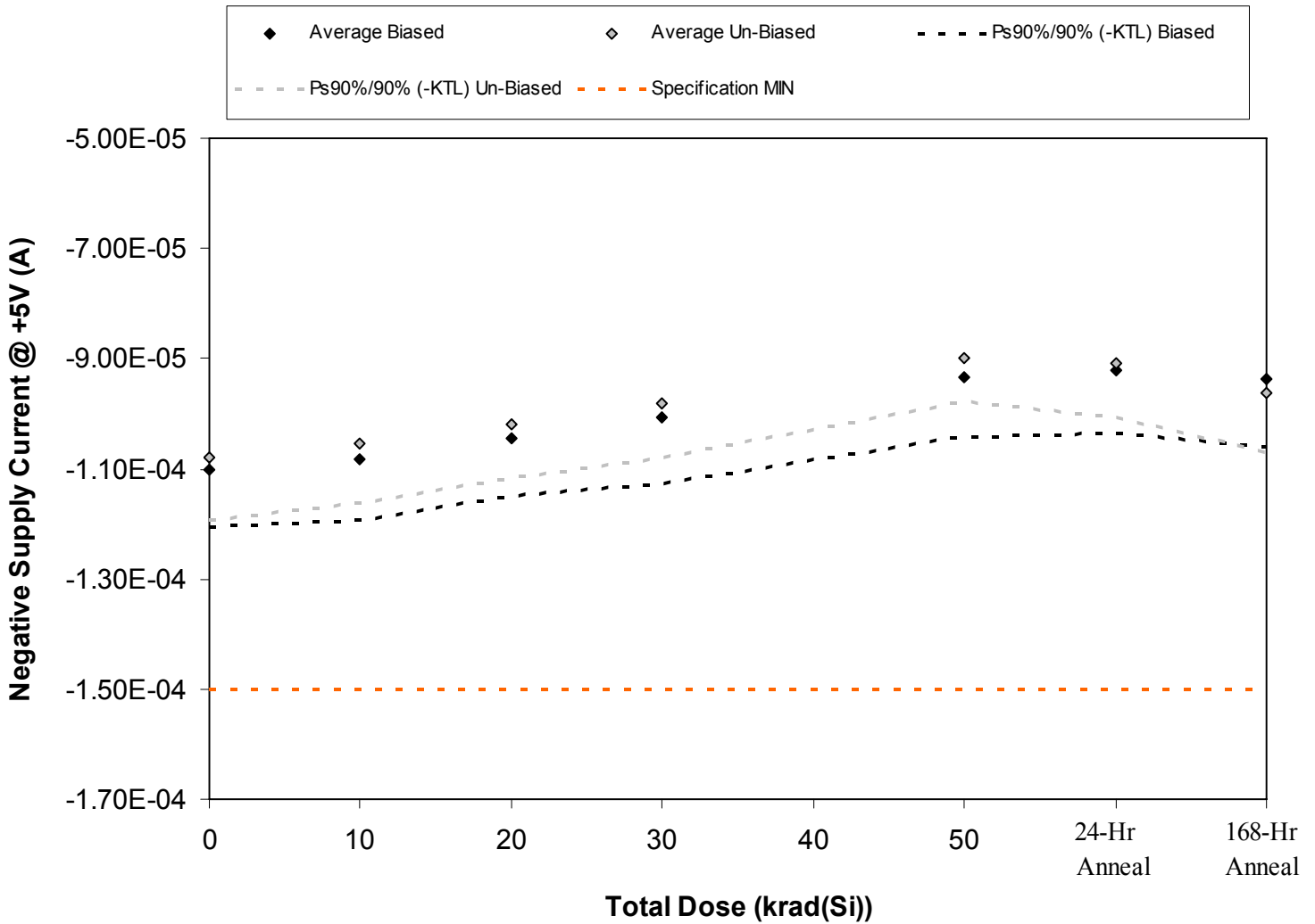
Figure 5.2. Plot of Negative Supply Current @ +5V (A) versus total dose. The solid diamonds are the average of the measured data points for the samples irradiated under electrical bias while the shaded diamonds are the average of the measured data points for the samples irradiated with all pins tied to ground. The black lines (solid and/or dashed) are the average of the data points after application of the KTL statistics on the samples irradiated under electrical bias while the gray lines (solid and/or dashed) are the average of the data points after application of the KTL statistics on the samples irradiated in the unbiased condition. The red dotted line(s) are the pre- and/or post-irradiation minimum and/or maximum specification value as defined in the datasheet and/or test plan.
