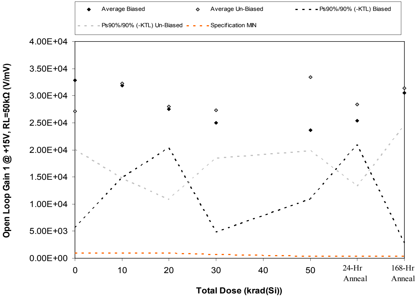
Figure 5.47. Plot of Open Loop Gain 1 @ +15V, RL=50kΩ (V/mV) versus total dose. The solid diamonds are the average of the measured data points for the samples irradiated under electrical bias while the shaded diamonds are the average of the measured data points for the samples irradiated with all pins tied to ground. The black lines (solid and/or dashed) are the average of the data points after application of the KTL statistics on the samples irradiated under electrical bias while the gray lines (solid and/or dashed) are the average of the data points after application of the KTL statistics on the samples irradiated in the unbiased condition. The red dotted line(s) are the pre- and/or post-irradiation minimum and/or maximum specification value as defined in the datasheet and/or test plan.
