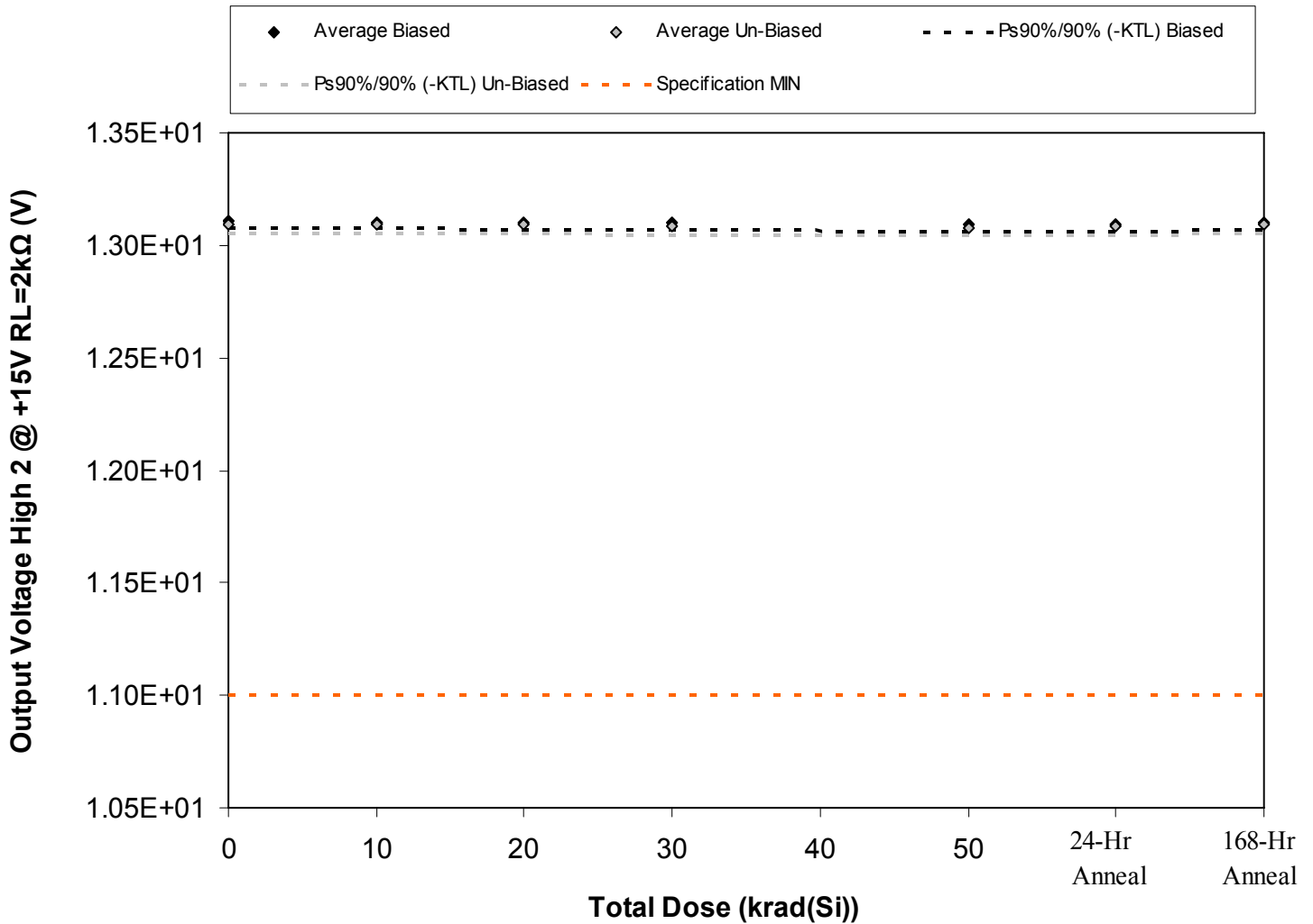
Figure 5.54. Plot of Output Voltage High 2 @ +15V RL=2kΩ (V) versus total dose. The solid diamonds are the average of the measured data points for the samples irradiated under electrical bias while the shaded diamonds are the average of the measured data points for the samples irradiated with all pins tied to ground. The black lines (solid and/or dashed) are the average of the data points after application of the KTL statistics on the samples irradiated under electrical bias while the gray lines (solid and/or dashed) are the average of the data points after application of the KTL statistics on the samples irradiated in the unbiased condition. The red dotted line(s) are the pre- and/or post-irradiation minimum and/or maximum specification value as defined in the datasheet and/or test plan.
