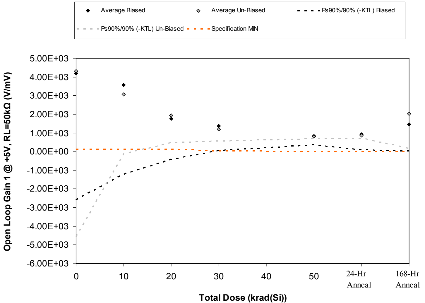
Figure 5.17. Plot of Open Loop Gain 1 @ +5V, RL=50kΩ (V/mV) versus total dose. The solid diamonds are the average of the measured data points for the samples irradiated under electrical bias while the shaded diamonds are the average of the measured data points for the samples irradiated with all pins tied to ground. The black lines (solid and/or dashed) are the average of the data points after application of the KTL statistics on the samples irradiated under electrical bias while the gray lines (solid and/or dashed) are the average of the data points after application of the KTL statistics on the samples irradiated in the unbiased condition. The red dotted line(s) are the pre- and/or post-irradiation minimum and/or maximum specification value as defined in the datasheet and/or test plan.
