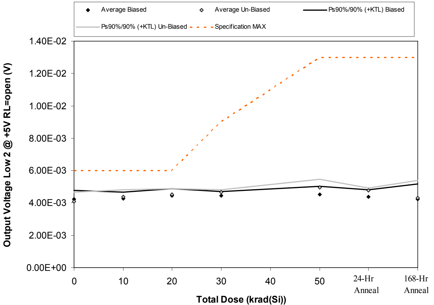
Figure 5.20. Plot of Output Voltage Low 2 @ +5V RL=open (V) versus total dose. The solid diamonds are the average of the measured data points for the samples irradiated under electrical bias while the shaded diamonds are the average of the measured data points for the samples irradiated with all pins tied to ground. The black lines (solid and/or dashed) are the average of the data points after application of the KTL statistics on the samples irradiated under electrical bias while the gray lines (solid and/or dashed) are the average of the data points after application of the KTL statistics on the samples irradiated in the unbiased condition. The red dotted line(s) are the pre- and/or post-irradiation minimum and/or maximum specification value as defined in the datasheet and/or test plan.
