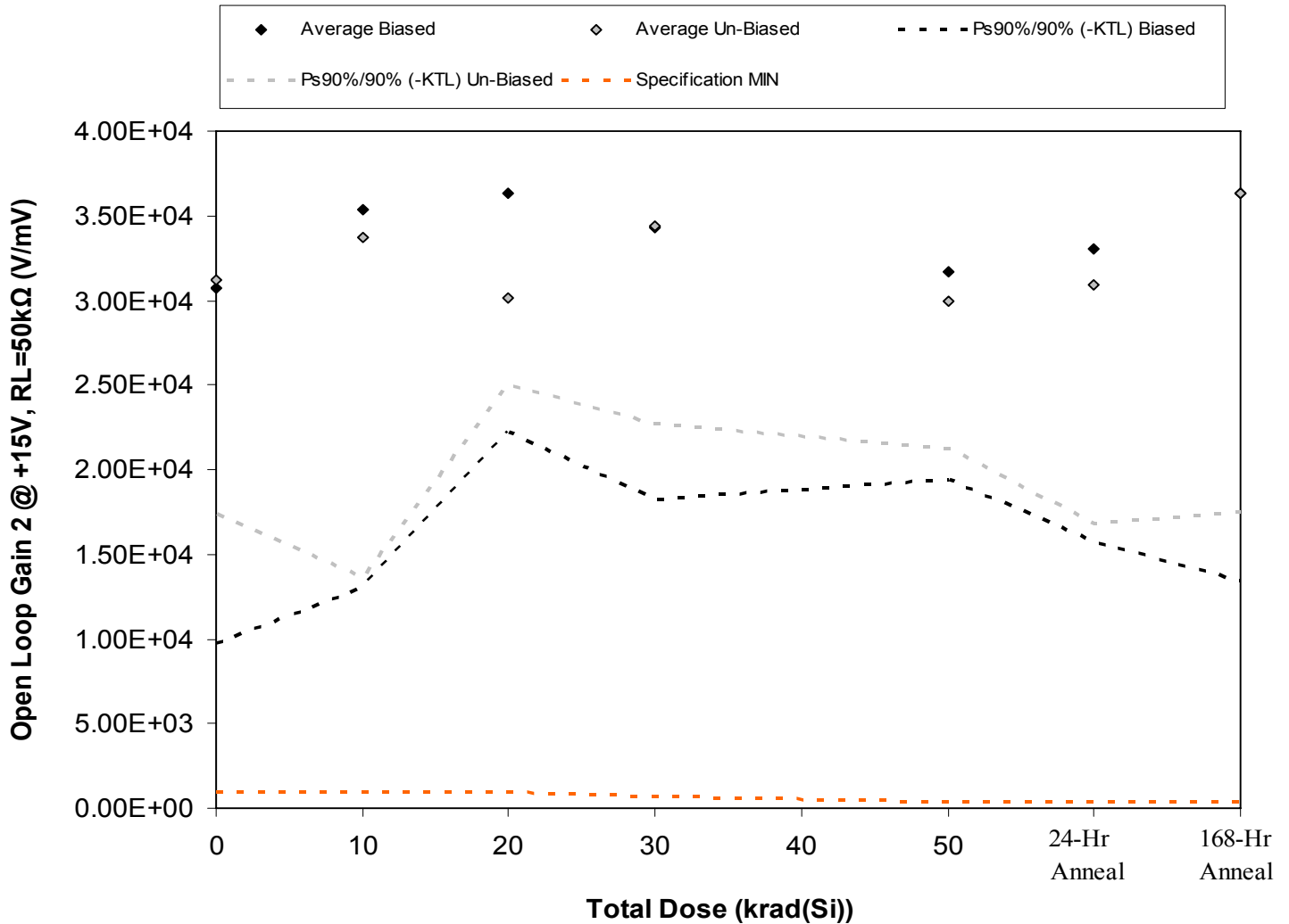
Figure 5.48. Plot of Open Loop Gain 2 @ +15V, RL=50kΩ (V/mV) versus total dose. The solid diamonds are the average of the measured data points for the samples irradiated under electrical bias while the shaded diamonds are the average of the measured data points for the samples irradiated with all pins tied to ground. The black lines (solid and/or dashed) are the average of the data points after application of the KTL statistics on the samples irradiated under electrical bias while the gray lines (solid and/or dashed) are the average of the data points after application of the KTL statistics on the samples irradiated in the unbiased condition. The red dotted line(s) are the pre- and/or post-irradiation minimum and/or maximum specification value as defined in the datasheet and/or test plan.
