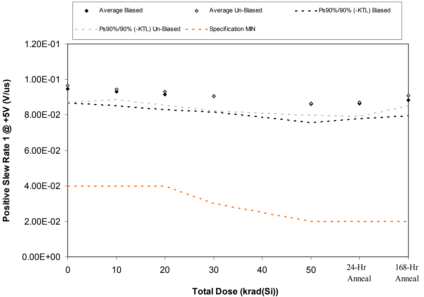
Figure 5.29. Plot of Positive Slew Rate 1 @ +5V (V/us) versus total dose. The solid diamonds are the average of the measured data points for the samples irradiated under electrical bias while the shaded diamonds are the average of the measured data points for the samples irradiated with all pins tied to ground. The black lines (solid and/or dashed) are the average of the data points after application of the KTL statistics on the samples irradiated under electrical bias while the gray lines (solid and/or dashed) are the average of the data points after application of the KTL statistics on the samples irradiated in the unbiased condition. The red dotted line(s) are the pre- and/or post-irradiation minimum and/or maximum specification value as defined in the datasheet and/or test plan.
