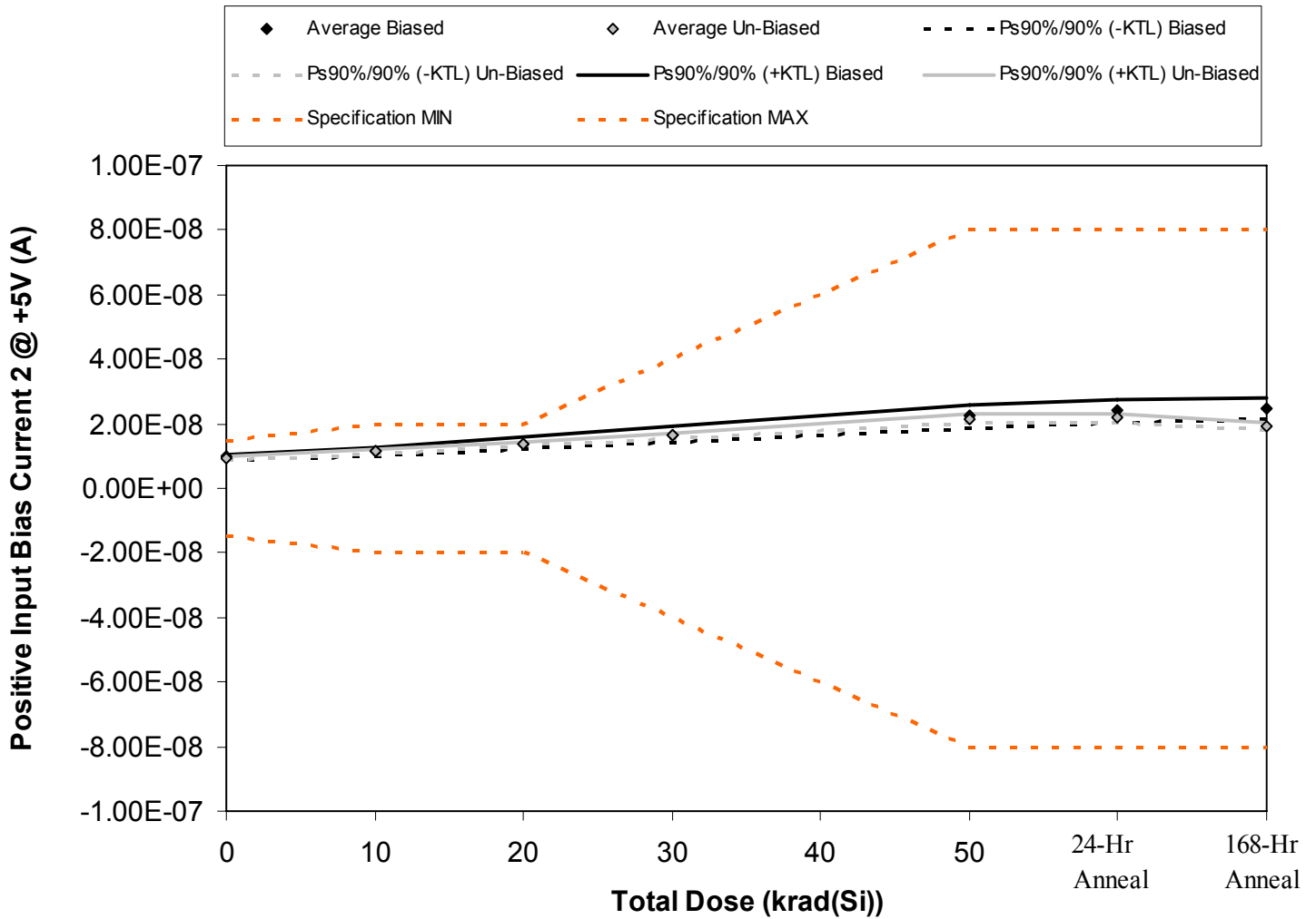
Figure 5.8. Plot of Positive Input Bias Current 2 @ +5V (A) versus total dose. The solid diamonds are the average of the measured data points for the samples irradiated under electrical bias while the shaded diamonds are the average of the measured data points for the samples irradiated with all pins tied to ground. The black lines (solid and/or dashed) are the average of the data points after application of the KTL statistics on the samples irradiated under electrical bias while the gray lines (solid and/or dashed) are the average of the data points after application of the KTL statistics on the samples irradiated in the unbiased condition. The red dotted line(s) are the pre- and/or post-irradiation minimum and/or maximum specification value as defined in the datasheet and/or test plan.
