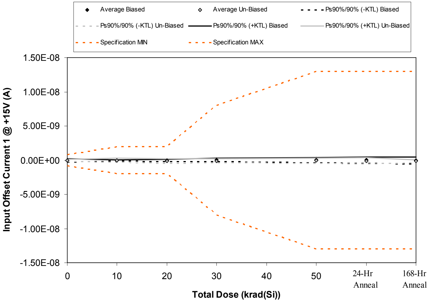
Figure 5.37. Plot of Input Offset Current 1 @ +15V (A) versus total dose. The solid diamonds are the average of the measured data points for the samples irradiated under electrical bias while the shaded diamonds are the average of the measured data points for the samples irradiated with all pins tied to ground. The black lines (solid and/or dashed) are the average of the data points after application of the KTL statistics on the samples irradiated under electrical bias while the gray lines (solid and/or dashed) are the average of the data points after application of the KTL statistics on the samples irradiated in the unbiased condition. The red dotted line(s) are the pre- and/or post-irradiation minimum and/or maximum specification value as defined in the datasheet and/or test plan.
