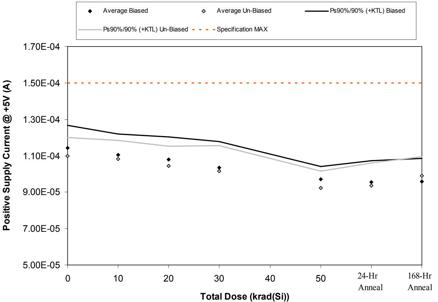
Figure 5.1. Plot of Positive Supply Current @ +5V (A) versus total dose. The solid diamonds are the average of the measured data points for the samples irradiated under electrical bias while the shaded diamonds are the average of the measured data points for the samples irradiated with all pins tied to ground. The black lines (solid and/or dashed) are the average of the data points after application of the KTL statistics on the samples irradiated under electrical bias while the gray lines (solid and/or dashed) are the average of the data points after application of the KTL statistics on the samples irradiated in the unbiased condition. The red dotted line(s) are the pre- and/or post-irradiation minimum and/or maximum specification value as defined in the datasheet and/or test plan.
