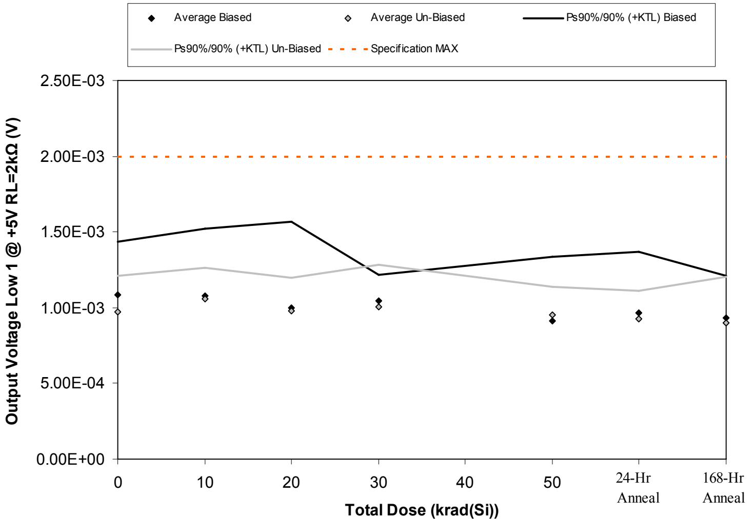
Figure 5.21. Plot of Output Voltage Low 1 @ +5V RL=2kΩ (V) versus total dose. The solid diamonds are the average of the measured data points for the samples irradiated under electrical bias while the shaded diamonds are the average of the measured data points for the samples irradiated with all pins tied to ground. The black lines (solid and/or dashed) are the average of the data points after application of the KTL statistics on the samples irradiated under electrical bias while the gray lines (solid and/or dashed) are the average of the data points after application of the KTL statistics on the samples irradiated in the unbiased condition. The red dotted line(s) are the pre- and/or post-irradiation minimum and/or maximum specification value as defined in the datasheet and/or test plan.
