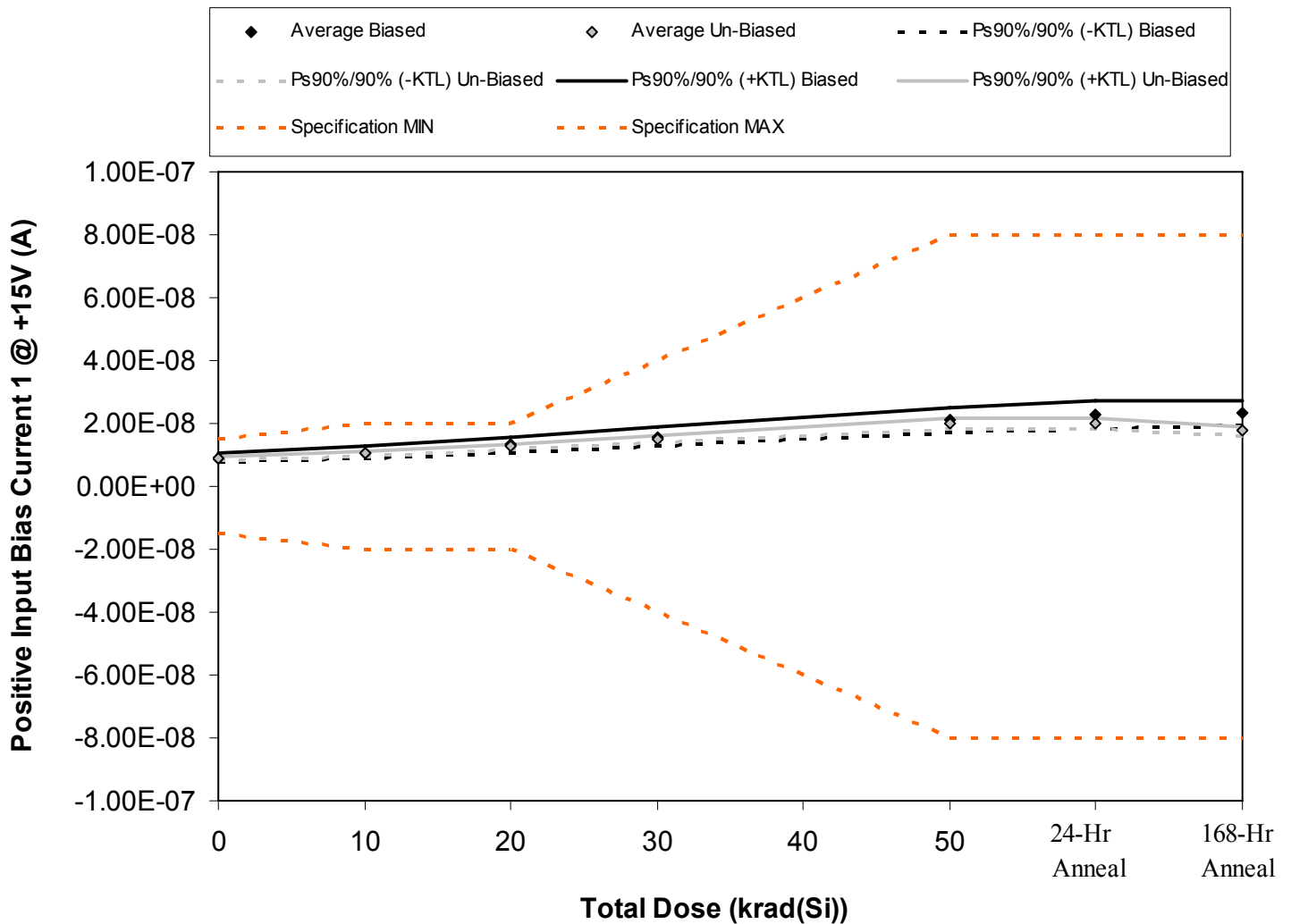
Figure 5.39. Plot of Positive Input Bias Current 1 @ +15V (A) versus total dose. The solid diamonds are the average of the measured data points for the samples irradiated under electrical bias while the shaded diamonds are the average of the measured data points for the samples irradiated with all pins tied to ground. The black lines (solid and/or dashed) are the average of the data points after application of the KTL statistics on the samples irradiated under electrical bias while the gray lines (solid and/or dashed) are the average of the data points after application of the KTL statistics on the samples irradiated in the unbiased condition. The red dotted line(s) are the pre- and/or post-irradiation minimum and/or maximum specification value as defined in the datasheet and/or test plan.
