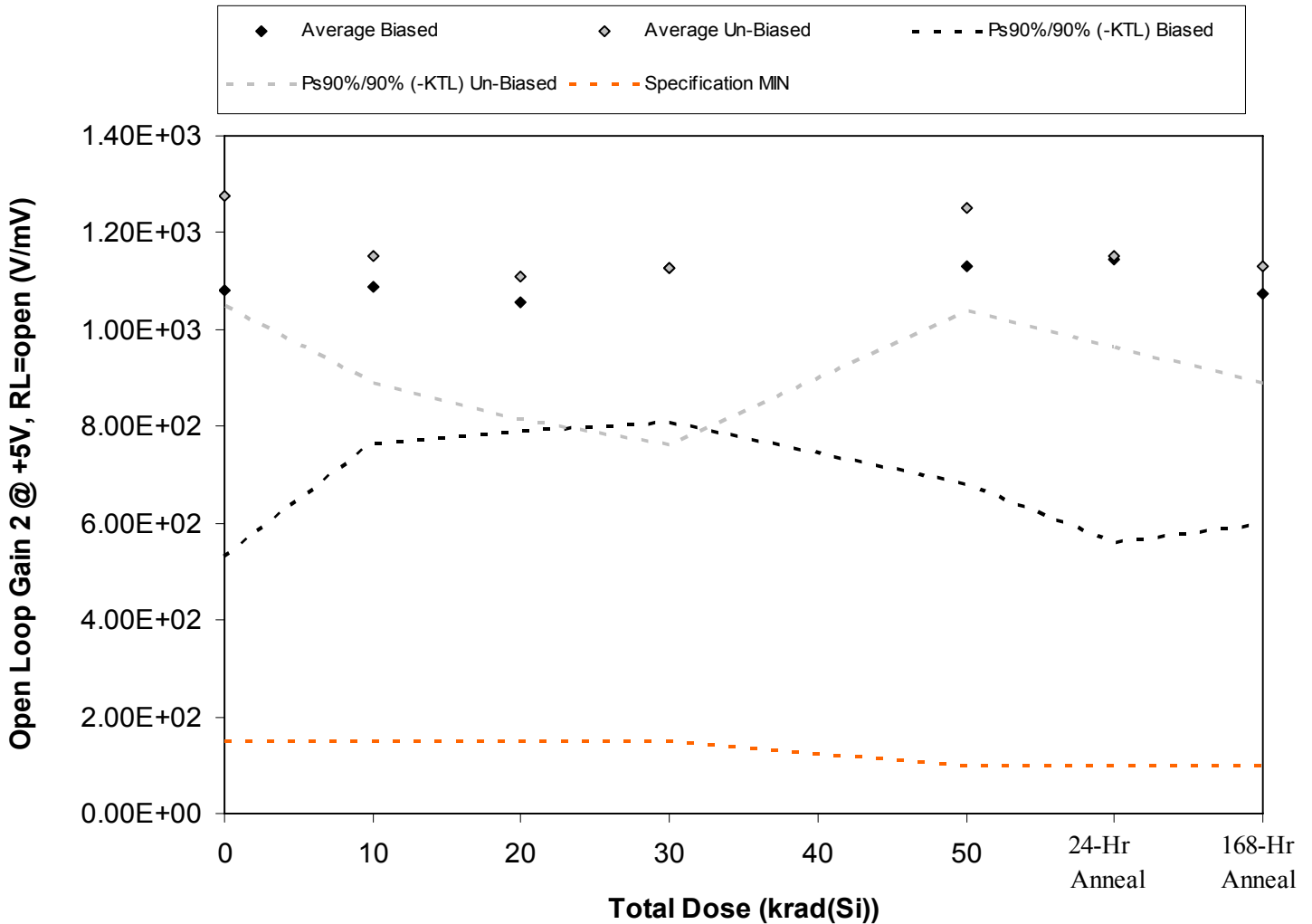
Figure 5.16. Plot of Open Loop Gain 2 @ +5V, RL=open (V/mV) versus total dose. The solid diamonds are the average of the measured data points for the samples irradiated under electrical bias while the shaded diamonds are the average of the measured data points for the samples irradiated with all pins tied to ground. The black lines (solid and/or dashed) are the average of the data points after application of the KTL statistics on the samples irradiated under electrical bias while the gray lines (solid and/or dashed) are the average of the data points after application of the KTL statistics on the samples irradiated in the unbiased condition. The red dotted line(s) are the pre- and/or post-irradiation minimum and/or maximum specification value as defined in the datasheet and/or test plan.
