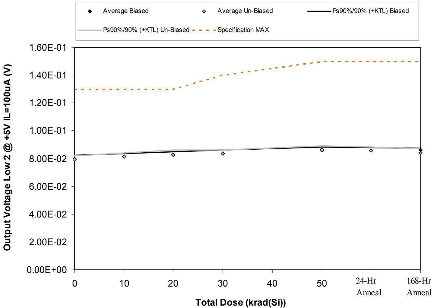
Figure 5.24. Plot of Output Voltage Low 2 @ +5V IL=100uA (V) versus total dose. The solid diamonds are the average of the measured data points for the samples irradiated under electrical bias while the shaded diamonds are the average of the measured data points for the samples irradiated with all pins tied to ground. The black lines (solid and/or dashed) are the average of the data points after application of the KTL statistics on the samples irradiated under electrical bias while the gray lines (solid and/or dashed) are the average of the data points after application of the KTL statistics on the samples irradiated in the unbiased condition. The red dotted line(s) are the pre- and/or post-irradiation minimum and/or maximum specification value as defined in the datasheet and/or test plan.
