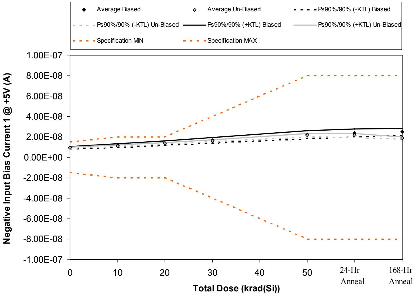
Figure 5.9. Plot of Negative Input Bias Current 1 @ +5V (A) versus total dose. The solid diamonds are the average of the measured data points for the samples irradiated under electrical bias while the shaded diamonds are the average of the measured data points for the samples irradiated with all pins tied to ground. The black lines (solid and/or dashed) are the average of the data points after application of the KTL statistics on the samples irradiated under electrical bias while the gray lines (solid and/or dashed) are the average of the data points after application of the KTL statistics on the samples irradiated in the unbiased condition. The red dotted line(s) are the pre- and/or post-irradiation minimum and/or maximum specification value as defined in the datasheet and/or test plan.
