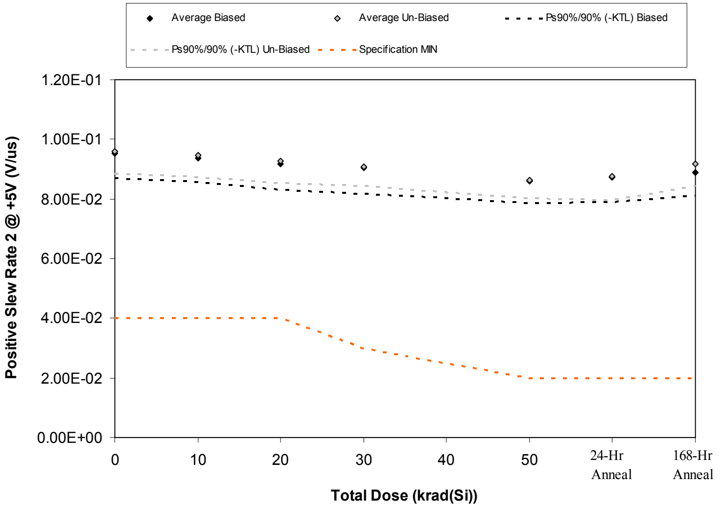
Figure 5.30. Plot of Positive Slew Rate 2 @ +5V (V/us) versus total dose. The solid diamonds are the average of the measured data points for the samples irradiated under electrical bias while the shaded diamonds are the average of the measured data points for the samples irradiated with all pins tied to ground. The black lines (solid and/or dashed) are the average of the data points after application of the KTL statistics on the samples irradiated under electrical bias while the gray lines (solid and/or dashed) are the average of the data points after application of the KTL statistics on the samples irradiated in the unbiased condition. The red dotted line(s) are the pre- and/or post-irradiation minimum and/or maximum specification value as defined in the datasheet and/or test plan.
