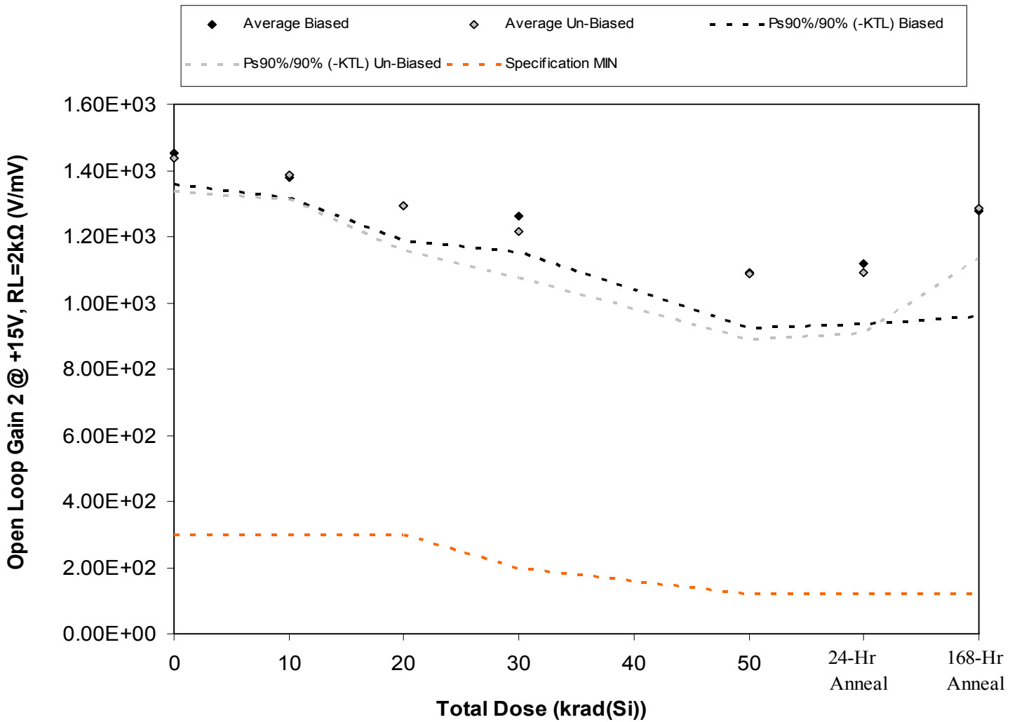
Figure 5.50. Plot of Open Loop Gain 2 @ +15V, RL=2kΩ (V/mV) versus total dose. The solid diamonds are the average of the measured data points for the samples irradiated under electrical bias while the shaded diamonds are the average of the measured data points for the samples irradiated with all pins tied to ground. The black lines (solid and/or dashed) are the average of the data points after application of the KTL statistics on the samples irradiated under electrical bias while the gray lines (solid and/or dashed) are the average of the data points after application of the KTL statistics on the samples irradiated in the unbiased condition. The red dotted line(s) are the pre- and/or post-irradiation minimum and/or maximum specification value as defined in the datasheet and/or test plan.
