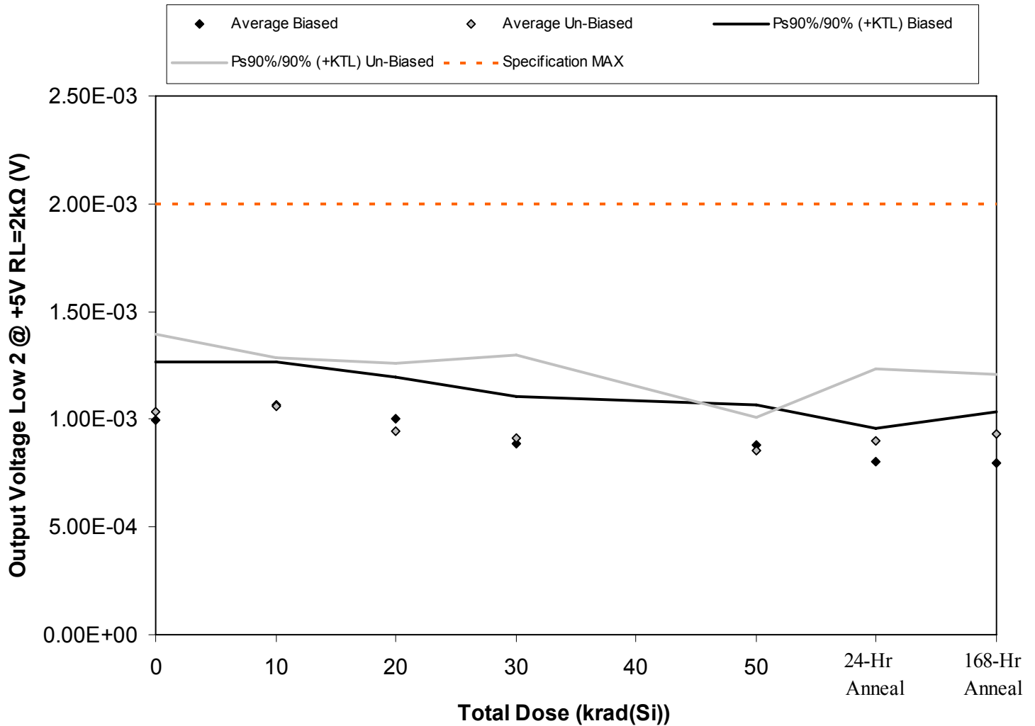
Figure 5.22. Plot of Output Voltage Low 2 @ +5V RL=2kΩ (V) versus total dose. The solid diamonds are the average of the measured data points for the samples irradiated under electrical bias while the shaded diamonds are the average of the measured data points for the samples irradiated with all pins tied to ground. The black lines (solid and/or dashed) are the average of the data points after application of the KTL statistics on the samples irradiated under electrical bias while the gray lines (solid and/or dashed) are the average of the data points after application of the KTL statistics on the samples irradiated in the unbiased condition. The red dotted line(s) are the pre- and/or post-irradiation minimum and/or maximum specification value as defined in the datasheet and/or test plan.
