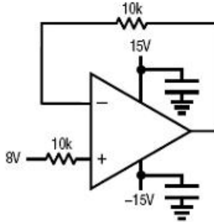
Figure B.1. Irradiation bias drawing for the units to be irradiated under electrical bias. This figure was extracted from LINEAR TECHNOLOGY CORPORATION RH1078M Datasheet.
