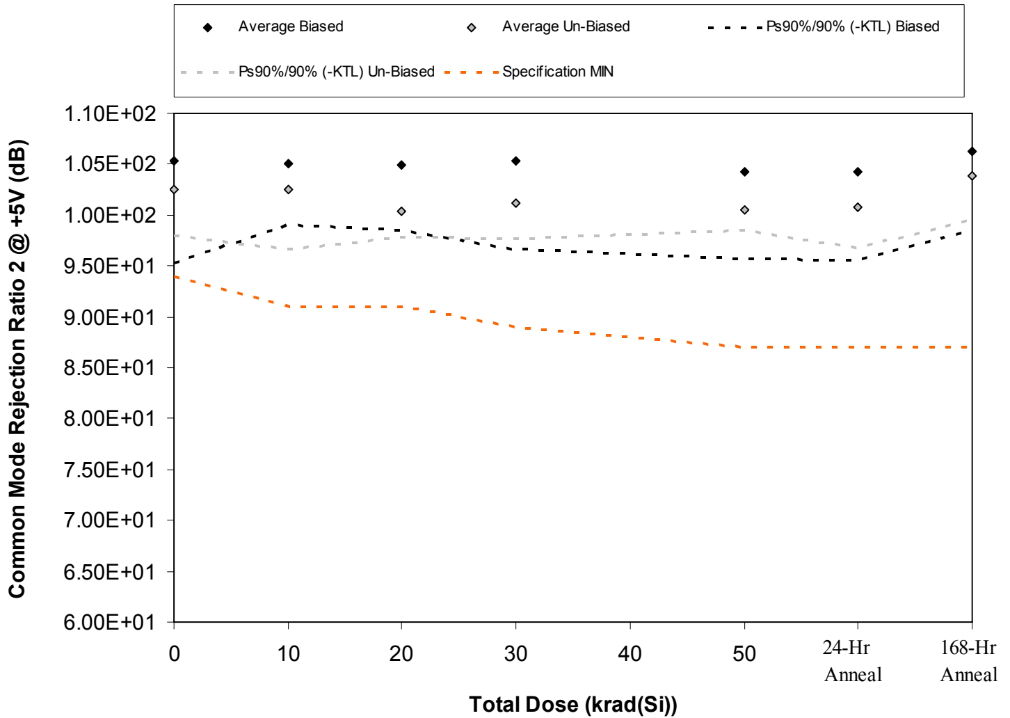
Figure 5.12. Plot of Common Mode Rejection Ratio 2 @ +5V (dB) versus total dose. The solid diamonds are the average of the measured data points for the samples irradiated under electrical bias while the shaded diamonds are the average of the measured data points for the samples irradiated with all pins tied to ground. The black lines (solid and/or dashed) are the average of the data points after application of the KTL statistics on the samples irradiated under electrical bias while the gray lines (solid and/or dashed) are the average of the data points after application of the KTL statistics on the samples irradiated in the unbiased condition. The red dotted line(s) are the pre- and/or post-irradiation minimum and/or maximum specification value as defined in the datasheet and/or test plan.
