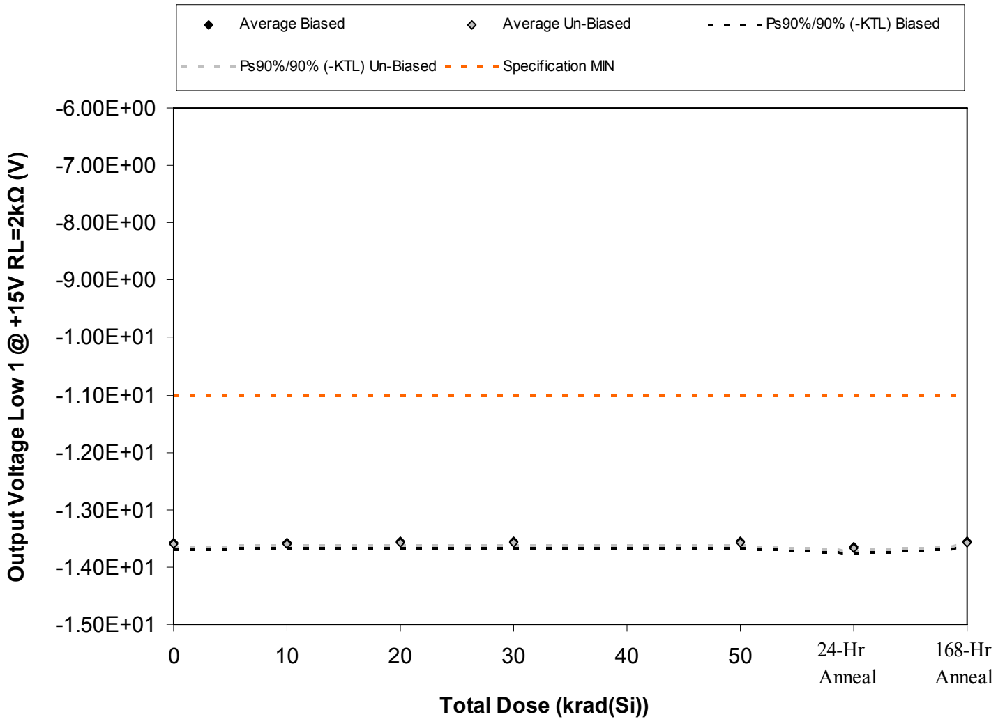
Figure 5.57. Plot of Output Voltage Low 1 @ +15V RL=2kΩ (V) versus total dose. The solid diamonds are the average of the measured data points for the samples irradiated under electrical bias while the shaded diamonds are the average of the measured data points for the samples irradiated with all pins tied to ground. The black lines (solid and/or dashed) are the average of the data points after application of the KTL statistics on the samples irradiated under electrical bias while the gray lines (solid and/or dashed) are the average of the data points after application of the KTL statistics on the samples irradiated in the unbiased condition. The red dotted line(s) are the pre- and/or post-irradiation minimum and/or maximum specification value as defined in the datasheet and/or test plan.
