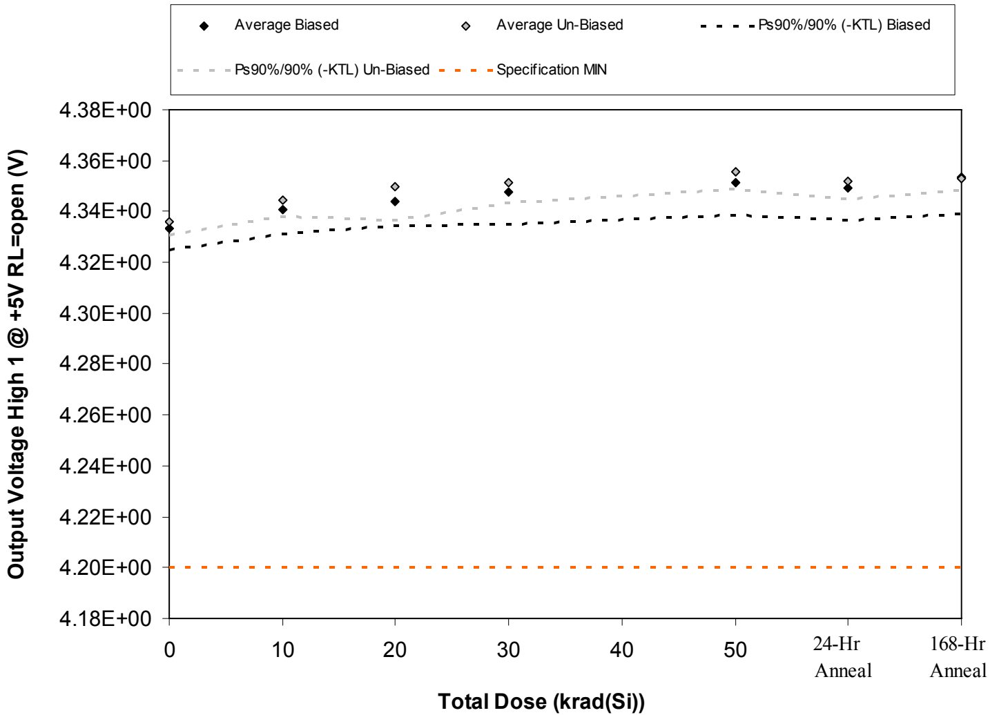
Figure 5.25. Plot of Output Voltage High 1 @ +5V RL=open (V) versus total dose. The solid diamonds are the average of the measured data points for the samples irradiated under electrical bias while the shaded diamonds are the average of the measured data points for the samples irradiated with all pins tied to ground. The black lines (solid and/or dashed) are the average of the data points after application of the KTL statistics on the samples irradiated under electrical bias while the gray lines (solid and/or dashed) are the average of the data points after application of the KTL statistics on the samples irradiated in the unbiased condition. The red dotted line(s) are the pre- and/or post-irradiation minimum and/or maximum specification value as defined in the datasheet and/or test plan.
