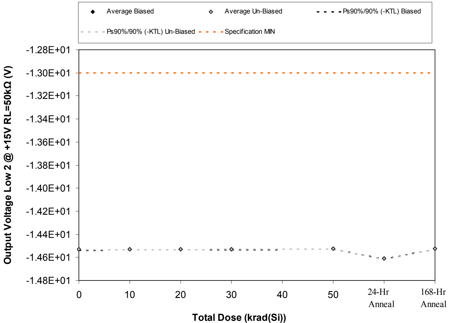
Figure 5.56. Plot of Output Voltage Low 2 @ +15V RL=50kΩ (V) versus total dose. The solid diamonds are the average of the measured data points for the samples irradiated under electrical bias while the shaded diamonds are the average of the measured data points for the samples irradiated with all pins tied to ground. The black lines (solid and/or dashed) are the average of the data points after application of the KTL statistics on the samples irradiated under electrical bias while the gray lines (solid and/or dashed) are the average of the data points after application of the KTL statistics on the samples irradiated in the unbiased condition. The red dotted line(s) are the pre- and/or post-irradiation minimum and/or maximum specification value as defined in the datasheet and/or test plan.
