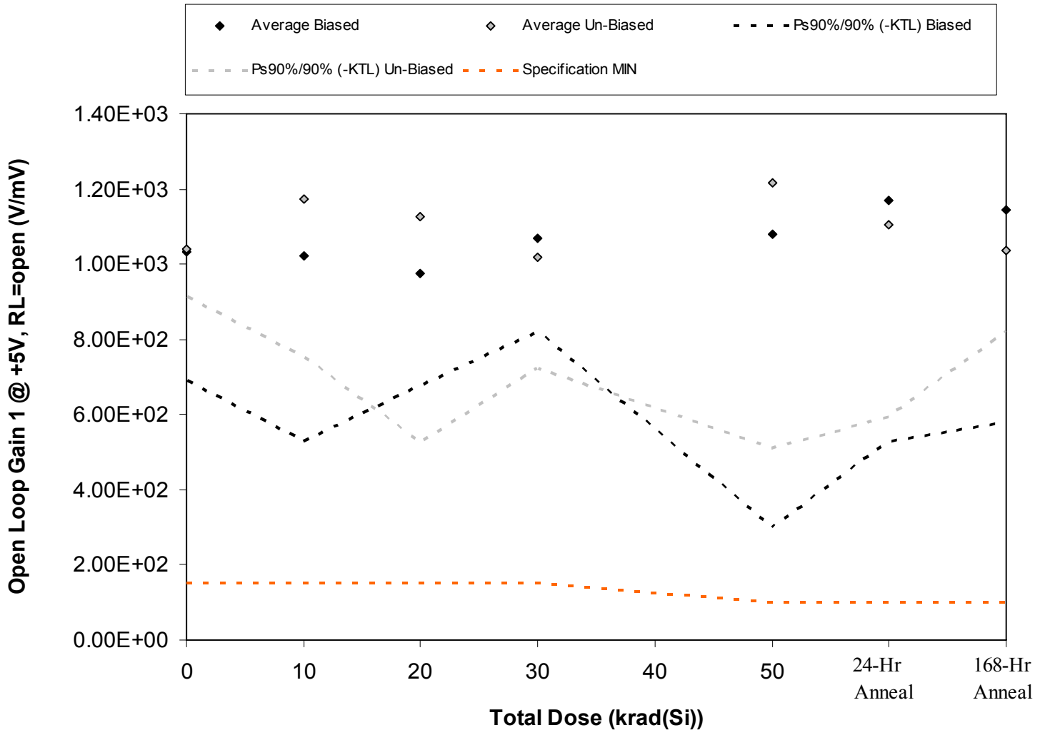
Figure 5.15. Plot of Open Loop Gain 1 @ +5V, RL=open (V/mV) versus total dose. The solid diamonds are the average of the measured data points for the samples irradiated under electrical bias while the shaded diamonds are the average of the measured data points for the samples irradiated with all pins tied to ground. The black lines (solid and/or dashed) are the average of the data points after application of the KTL statistics on the samples irradiated under electrical bias while the gray lines (solid and/or dashed) are the average of the data points after application of the KTL statistics on the samples irradiated in the unbiased condition. The red dotted line(s) are the pre- and/or post-irradiation minimum and/or maximum specification value as defined in the datasheet and/or test plan.
