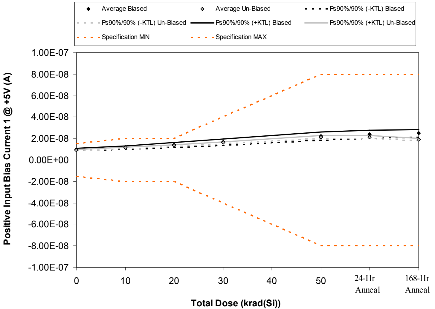
Figure 5.7. Plot of Positive Input Bias Current 1 @ +5V (A) versus total dose. The solid diamonds are the average of the measured data points for the samples irradiated under electrical bias while the shaded diamonds are the average of the measured data points for the samples irradiated with all pins tied to ground. The black lines (solid and/or dashed) are the average of the data points after application of the KTL statistics on the samples irradiated under electrical bias while the gray lines (solid and/or dashed) are the average of the data points after application of the KTL statistics on the samples irradiated in the unbiased condition. The red dotted line(s) are the pre- and/or post-irradiation minimum and/or maximum specification value as defined in the datasheet and/or test plan.
