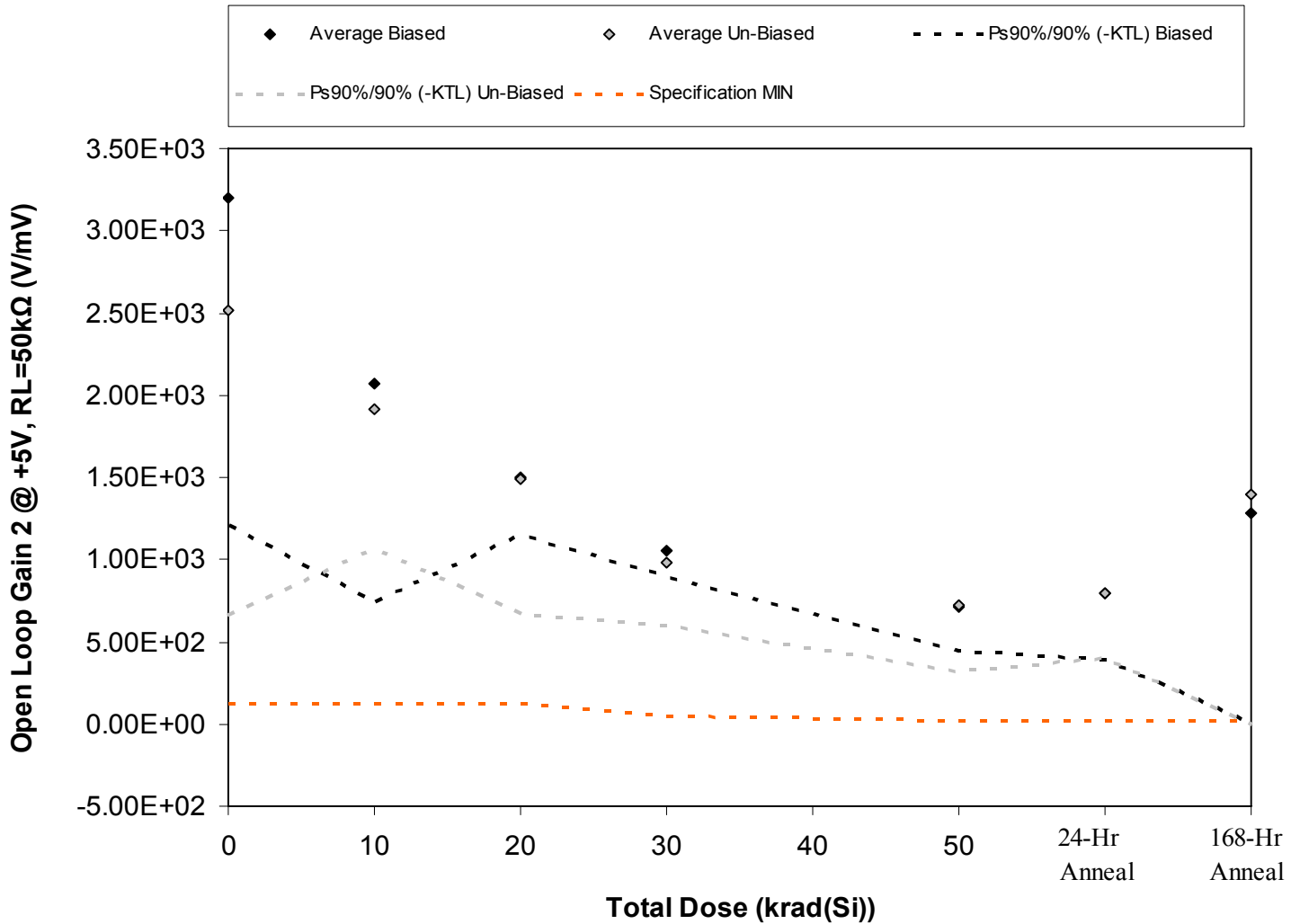
Figure 5.18. Plot of Open Loop Gain 2 @ +5V, RL=50kΩ (V/mV) versus total dose. The solid diamonds are the average of the measured data points for the samples irradiated under electrical bias while the shaded diamonds are the average of the measured data points for the samples irradiated with all pins tied to ground. The black lines (solid and/or dashed) are the average of the data points after application of the KTL statistics on the samples irradiated under electrical bias while the gray lines (solid and/or dashed) are the average of the data points after application of the KTL statistics on the samples irradiated in the unbiased condition. The red dotted line(s) are the pre- and/or post-irradiation minimum and/or maximum specification value as defined in the datasheet and/or test plan.
