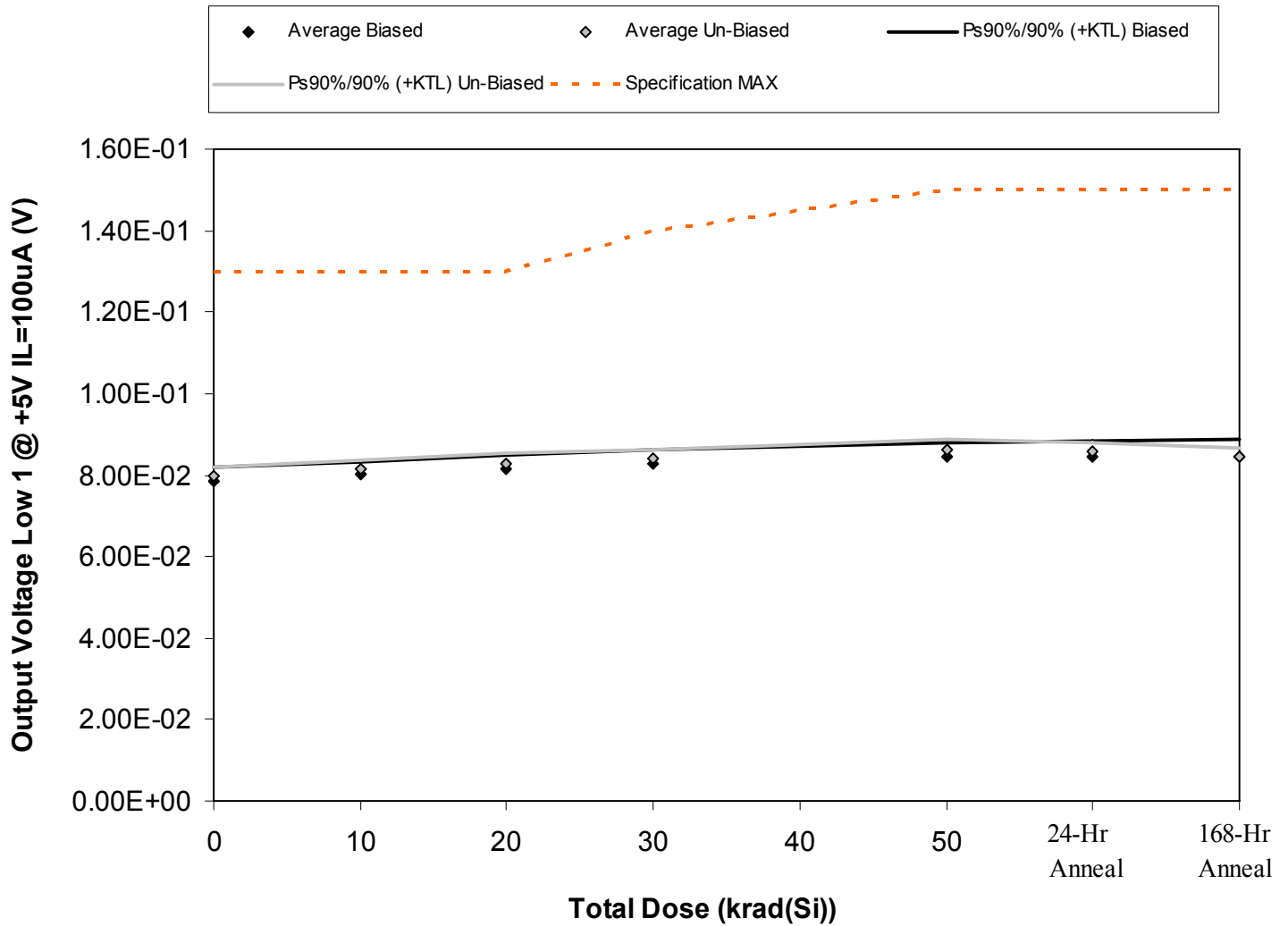
Figure 5.23. Plot of Output Voltage Low 1 @ +5V IL=100uA (V) versus total dose. The solid diamonds are the average of the measured data points for the samples irradiated under electrical bias while the shaded diamonds are the average of the measured data points for the samples irradiated with all pins tied to ground. The black lines (solid and/or dashed) are the average of the data points after application of the KTL statistics on the samples irradiated under electrical bias while the gray lines (solid and/or dashed) are the average of the data points after application of the KTL statistics on the samples irradiated in the unbiased condition. The red dotted line(s) are the pre- and/or post-irradiation minimum and/or maximum specification value as defined in the datasheet and/or test plan.
