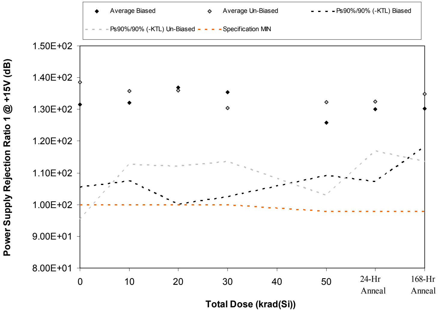
Figure 5.45. Plot of Power Supply Rejection Ratio 1 @ +15V (dB) versus total dose. The solid diamonds are the average of the measured data points for the samples irradiated under electrical bias while the shaded diamonds are the average of the measured data points for the samples irradiated with all pins tied to ground. The black lines (solid and/or dashed) are the average of the data points after application of the KTL statistics on the samples irradiated under electrical bias while the gray lines (solid and/or dashed) are the average of the data points after application of the KTL statistics on the samples irradiated in the unbiased condition. The red dotted line(s) are the pre- and/or post-irradiation minimum and/or maximum specification value as defined in the datasheet and/or test plan.
