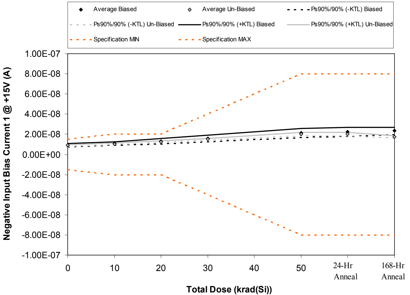
Figure 5.41. Plot of Negative Input Bias Current 1 @ +15V (A) versus total dose. The solid diamonds are the average of the measured data points for the samples irradiated under electrical bias while the shaded diamonds are the average of the measured data points for the samples irradiated with all pins tied to ground. The black lines (solid and/or dashed) are the average of the data points after application of the KTL statistics on the samples irradiated under electrical bias while the gray lines (solid and/or dashed) are the average of the data points after application of the KTL statistics on the samples irradiated in the unbiased condition. The red dotted line(s) are the pre- and/or post-irradiation minimum and/or maximum specification value as defined in the datasheet and/or test plan.
