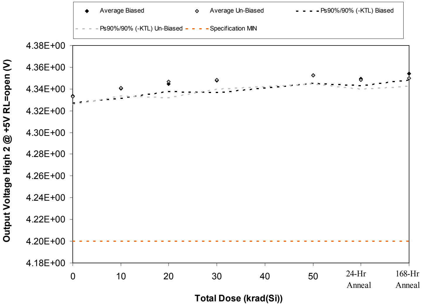
Figure 5.26. Plot of Output Voltage High 2 @ +5V RL=open (V) versus total dose. The solid diamonds are the average of the measured data points for the samples irradiated under electrical bias while the shaded diamonds are the average of the measured data points for the samples irradiated with all pins tied to ground. The black lines (solid and/or dashed) are the average of the data points after application of the KTL statistics on the samples irradiated under electrical bias while the gray lines (solid and/or dashed) are the average of the data points after application of the KTL statistics on the samples irradiated in the unbiased condition. The red dotted line(s) are the pre- and/or post-irradiation minimum and/or maximum specification value as defined in the datasheet and/or test plan.
