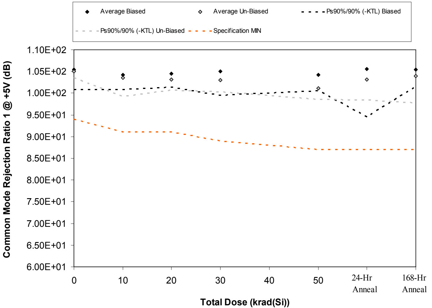
Figure 5.11. Plot of Common Mode Rejection Ratio 1 @ +5V (dB) versus total dose. The solid diamonds are the average of the measured data points for the samples irradiated under electrical bias while the shaded diamonds are the average of the measured data points for the samples irradiated with all pins tied to ground. The black lines (solid and/or dashed) are the average of the data points after application of the KTL statistics on the samples irradiated under electrical bias while the gray lines (solid and/or dashed) are the average of the data points after application of the KTL statistics on the samples irradiated in the unbiased condition. The red dotted line(s) are the pre- and/or post-irradiation minimum and/or maximum specification value as defined in the datasheet and/or test plan.
