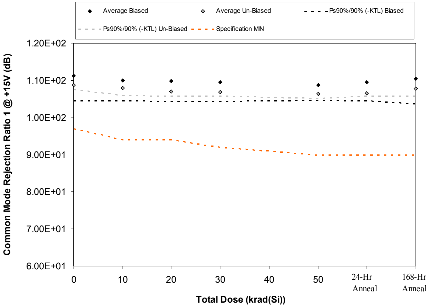
Figure 5.43. Plot of Common Mode Rejection Ratio 1 @ +15V (dB) versus total dose. The solid diamonds are the average of the measured data points for the samples irradiated under electrical bias while the shaded diamonds are the average of the measured data points for the samples irradiated with all pins tied to ground. The black lines (solid and/or dashed) are the average of the data points after application of the KTL statistics on the samples irradiated under electrical bias while the gray lines (solid and/or dashed) are the average of the data points after application of the KTL statistics on the samples irradiated in the unbiased condition. The red dotted line(s) are the pre- and/or post-irradiation minimum and/or maximum specification value as defined in the datasheet and/or test plan.
