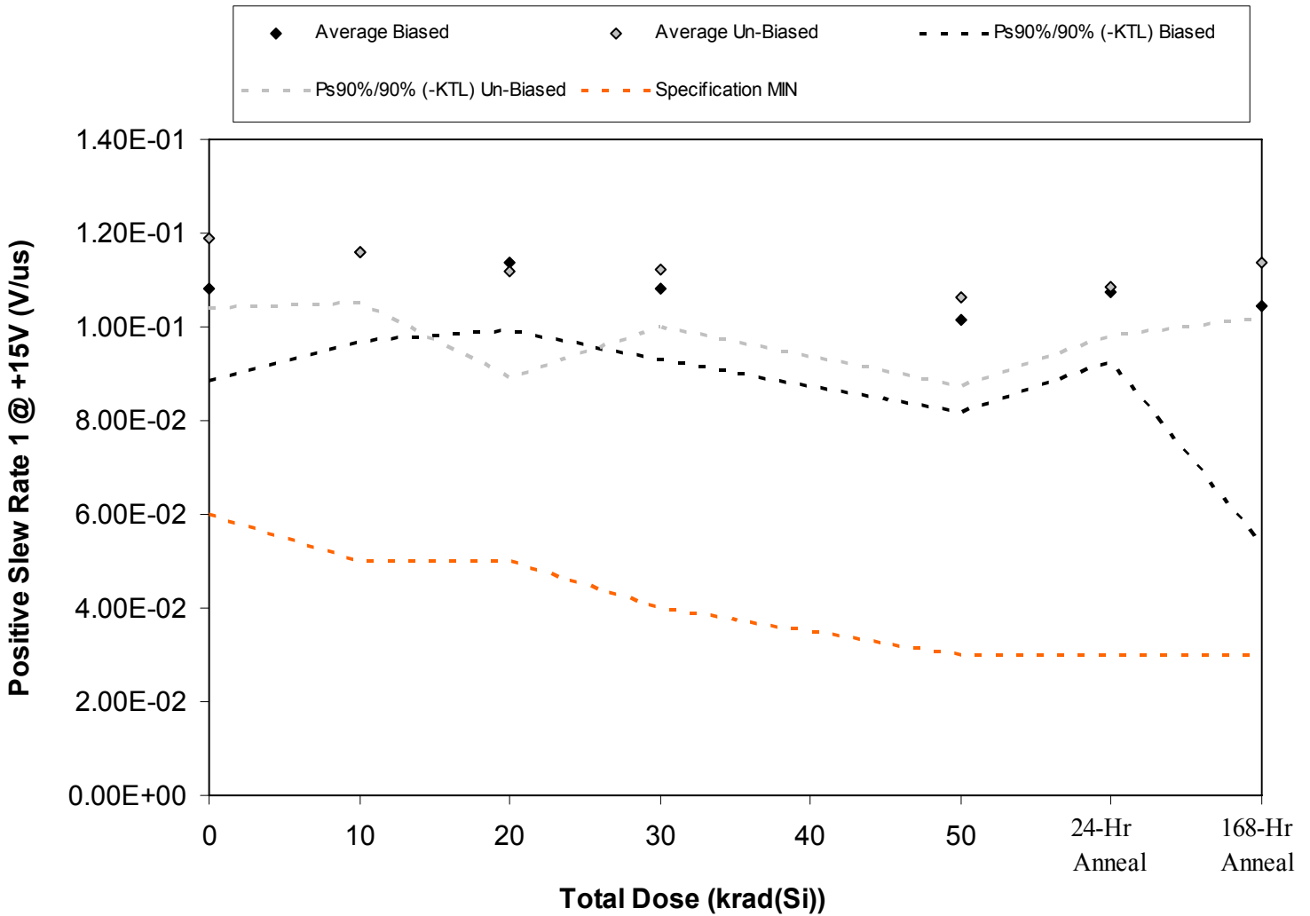
Figure 5.59. Plot of Positive Slew Rate 1 @ +15V (V/us) versus total dose. The solid diamonds are the average of the measured data points for the samples irradiated under electrical bias while the shaded diamonds are the average of the measured data points for the samples irradiated with all pins tied to ground. The black lines (solid and/or dashed) are the average of the data points after application of the KTL statistics on the samples irradiated under electrical bias while the gray lines (solid and/or dashed) are the average of the data points after application of the KTL statistics on the samples irradiated in the unbiased condition. The red dotted line(s) are the pre- and/or post-irradiation minimum and/or maximum specification value as defined in the datasheet and/or test plan.
