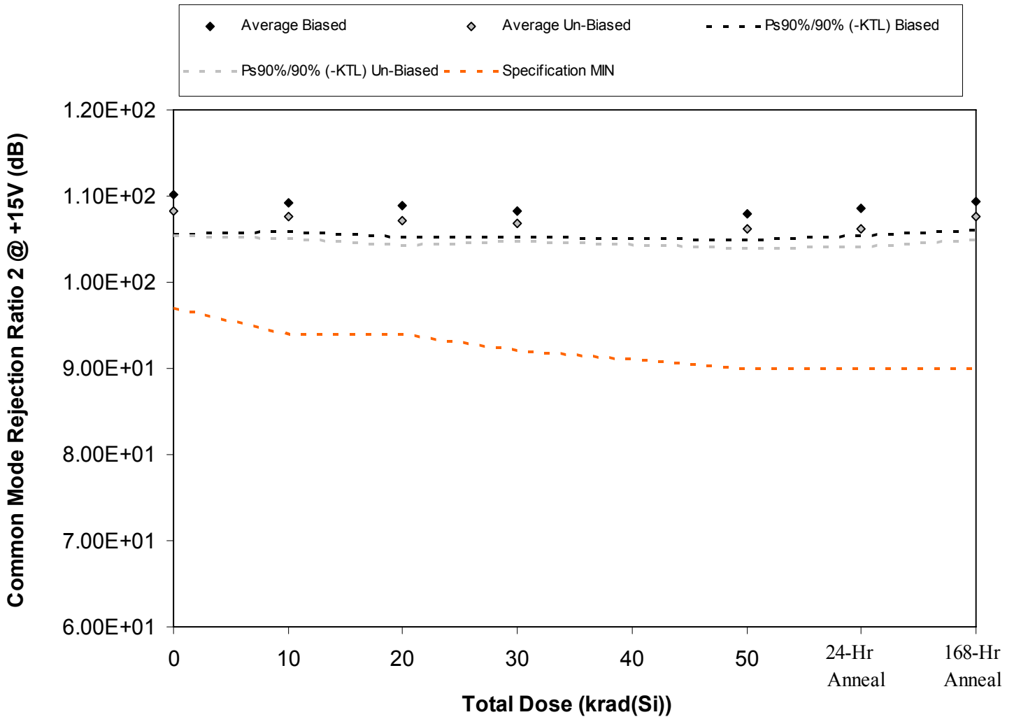
Figure 5.44. Plot of Common Mode Rejection Ratio 2 @ +15V (dB) versus total dose. The solid diamonds are the average of the measured data points for the samples irradiated under electrical bias while the shaded diamonds are the average of the measured data points for the samples irradiated with all pins tied to ground. The black lines (solid and/or dashed) are the average of the data points after application of the KTL statistics on the samples irradiated under electrical bias while the gray lines (solid and/or dashed) are the average of the data points after application of the KTL statistics on the samples irradiated in the unbiased condition. The red dotted line(s) are the pre- and/or post-irradiation minimum and/or maximum specification value as defined in the datasheet and/or test plan.
