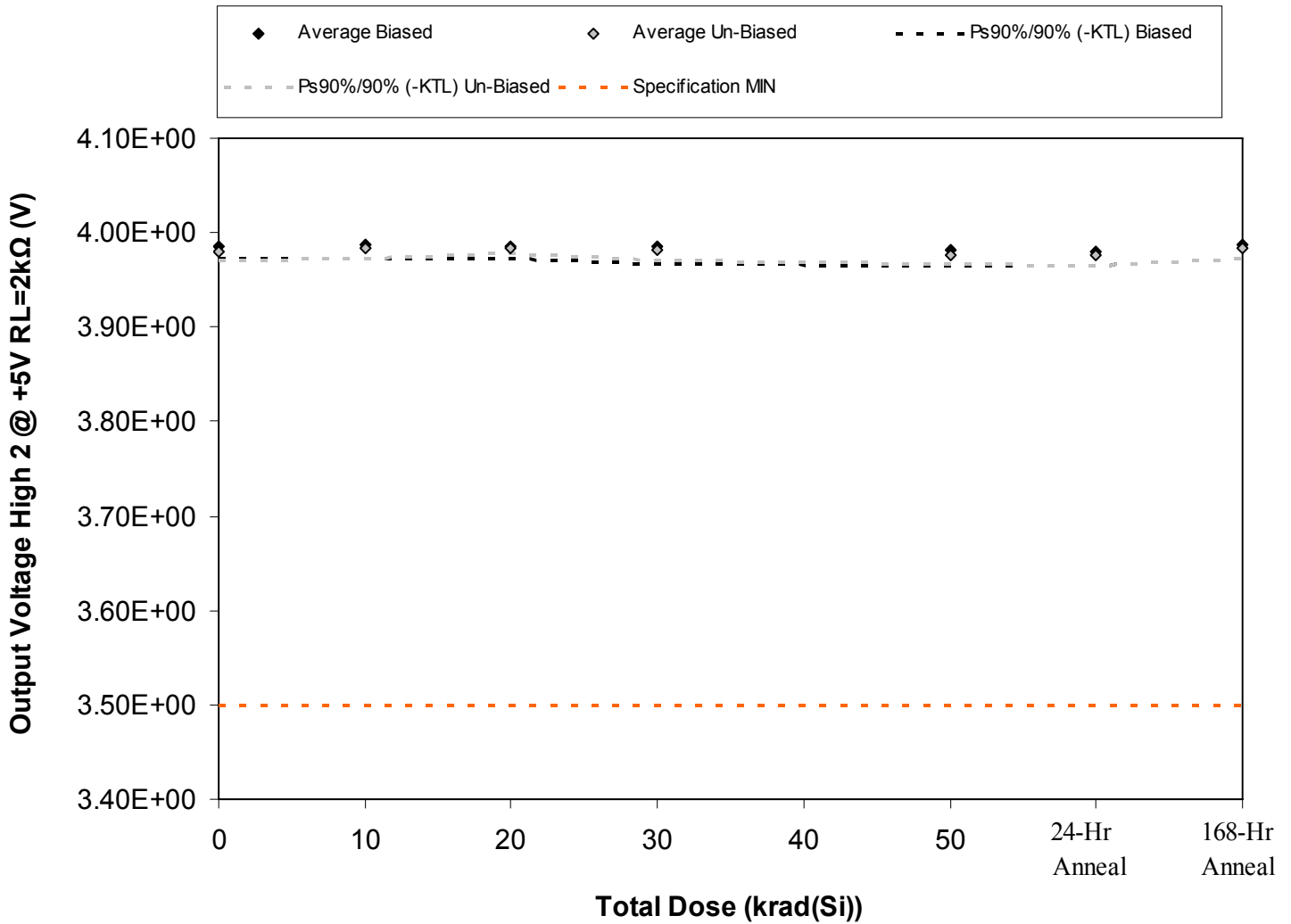
Figure 5.28. Plot of Output Voltage High 2 @ +5V RL=2kΩ (V) versus total dose. The solid diamonds are the average of the measured data points for the samples irradiated under electrical bias while the shaded diamonds are the average of the measured data points for the samples irradiated with all pins tied to ground. The black lines (solid and/or dashed) are the average of the data points after application of the KTL statistics on the samples irradiated under electrical bias while the gray lines (solid and/or dashed) are the average of the data points after application of the KTL statistics on the samples irradiated in the unbiased condition. The red dotted line(s) are the pre- and/or post-irradiation minimum and/or maximum specification value as defined in the datasheet and/or test plan.
