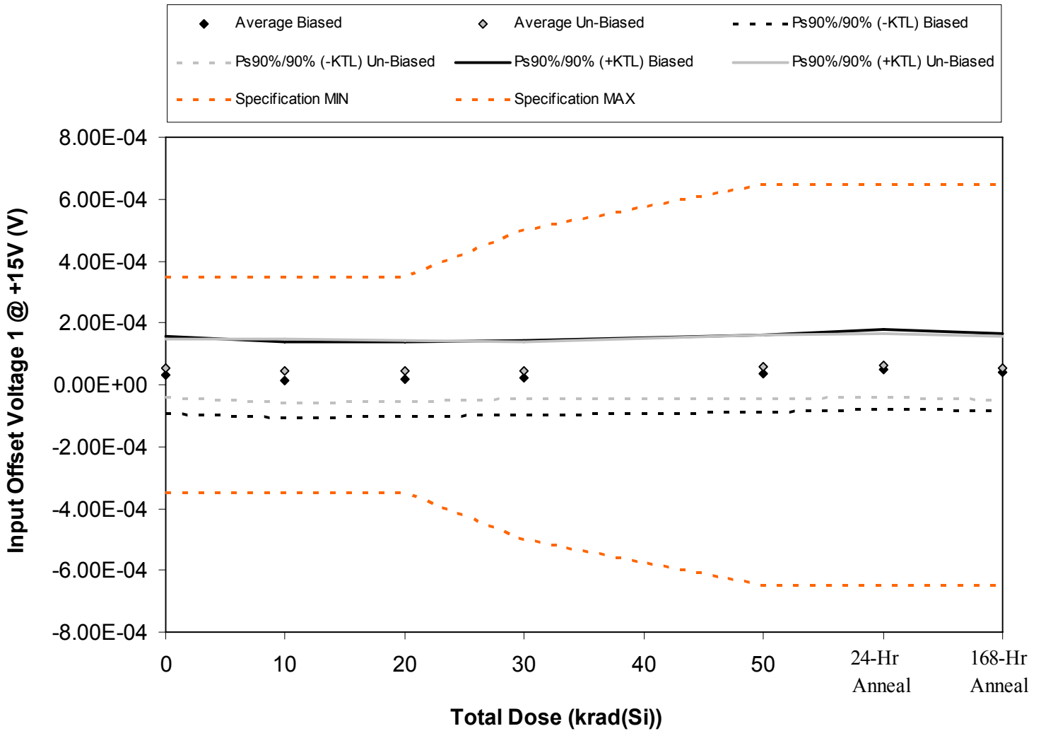
Figure 5.35. Plot of Input Offset Voltage 1 @ +15V (V) versus total dose. The solid diamonds are the average of the measured data points for the samples irradiated under electrical bias while the shaded diamonds are the average of the measured data points for the samples irradiated with all pins tied to ground. The black lines (solid and/or dashed) are the average of the data points after application of the KTL statistics on the samples irradiated under electrical bias while the gray lines (solid and/or dashed) are the average of the data points after application of the KTL statistics on the samples irradiated in the unbiased condition. The red dotted line(s) are the pre- and/or post-irradiation minimum and/or maximum specification value as defined in the datasheet and/or test plan.
