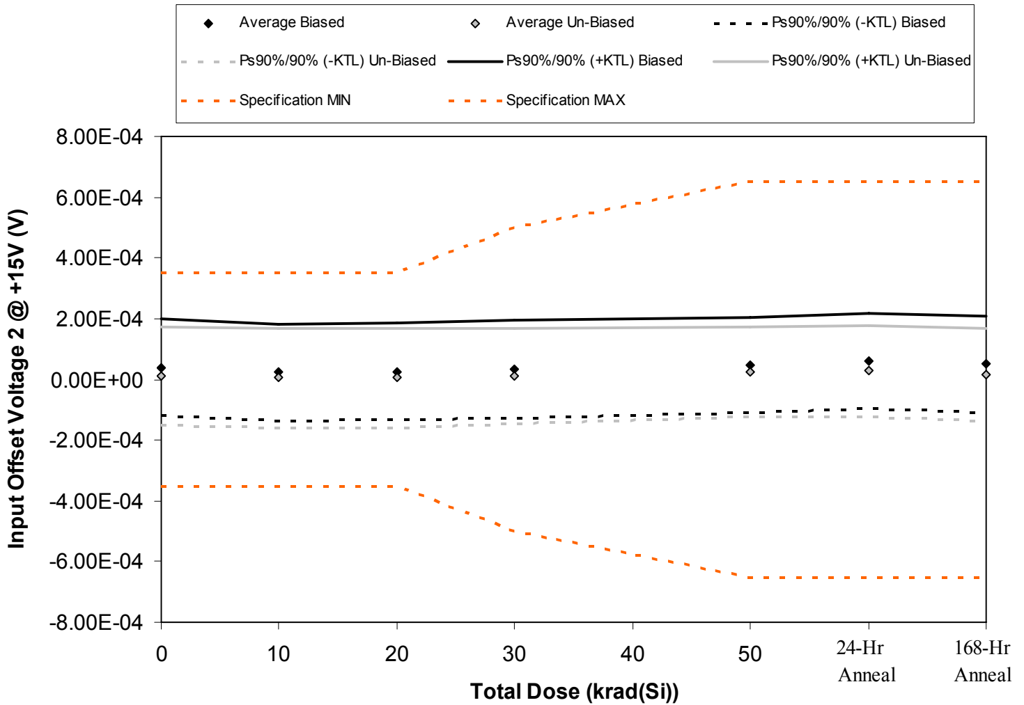
Figure 5.36. Plot of Input Offset Voltage 2 @ +15V (V) versus total dose. The solid diamonds are the average of the measured data points for the samples irradiated under electrical bias while the shaded diamonds are the average of the measured data points for the samples irradiated with all pins tied to ground. The black lines (solid and/or dashed) are the average of the data points after application of the KTL statistics on the samples irradiated under electrical bias while the gray lines (solid and/or dashed) are the average of the data points after application of the KTL statistics on the samples irradiated in the unbiased condition. The red dotted line(s) are the pre- and/or post-irradiation minimum and/or maximum specification value as defined in the datasheet and/or test plan.
