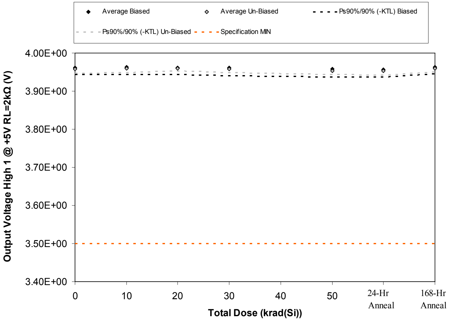
Figure 5.27. Plot of Output Voltage High 1 @ +5V RL=2kΩ (V) versus total dose. The solid diamonds are the average of the measured data points for the samples irradiated under electrical bias while the shaded diamonds are the average of the measured data points for the samples irradiated with all pins tied to ground. The black lines (solid and/or dashed) are the average of the data points after application of the KTL statistics on the samples irradiated under electrical bias while the gray lines (solid and/or dashed) are the average of the data points after application of the KTL statistics on the samples irradiated in the unbiased condition. The red dotted line(s) are the pre- and/or post-irradiation minimum and/or maximum specification value as defined in the datasheet and/or test plan.
