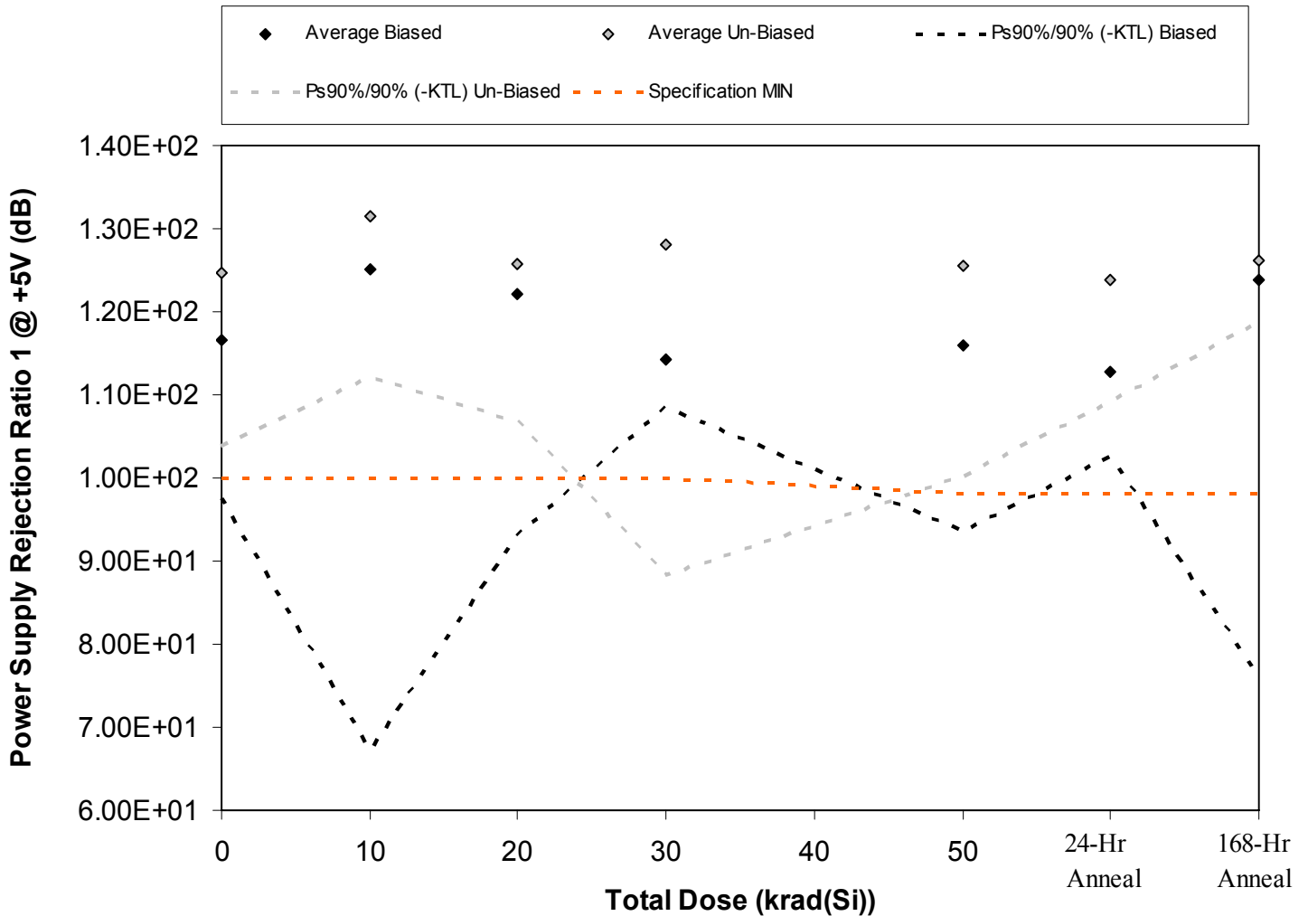
Figure 5.13. Plot of Power Supply Rejection Ratio 1 @ +5V (dB) versus total dose. The solid diamonds are the average of the measured data points for the samples irradiated under electrical bias while the shaded diamonds are the average of the measured data points for the samples irradiated with all pins tied to ground. The black lines (solid and/or dashed) are the average of the data points after application of the KTL statistics on the samples irradiated under electrical bias while the gray lines (solid and/or dashed) are the average of the data points after application of the KTL statistics on the samples irradiated in the unbiased condition. The red dotted line(s) are the pre- and/or post-irradiation minimum and/or maximum specification value as defined in the datasheet and/or test plan.
