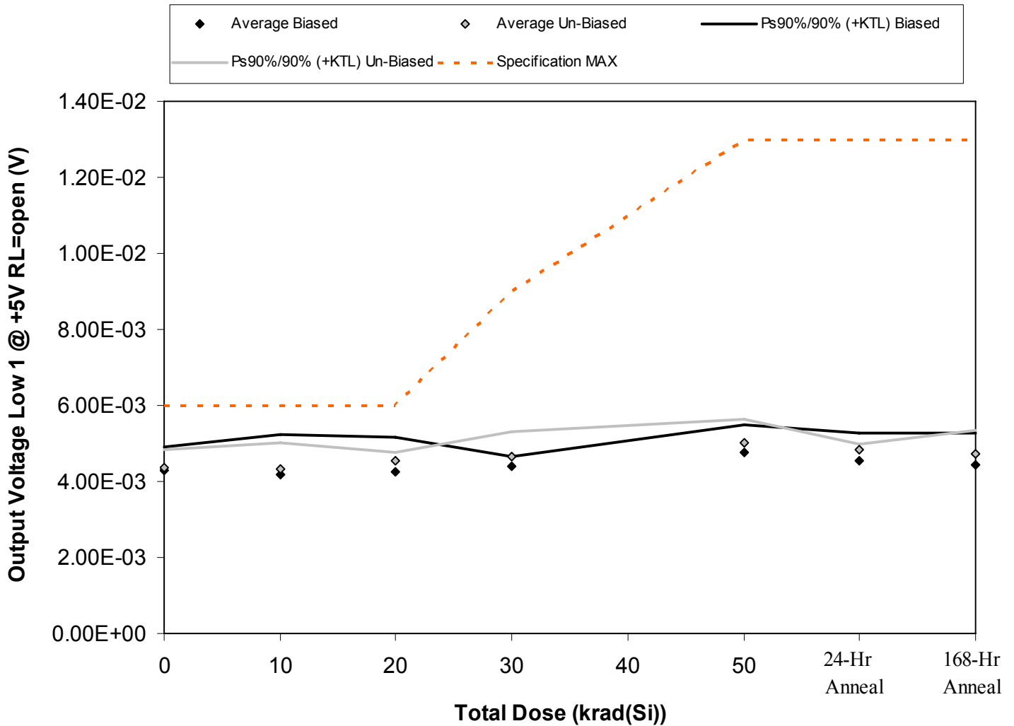
Figure 5.19. Plot of Output Voltage Low 1 @ +5V RL=open (V) versus total dose. The solid diamonds are the average of the measured data points for the samples irradiated under electrical bias while the shaded diamonds are the average of the measured data points for the samples irradiated with all pins tied to ground. The black lines (solid and/or dashed) are the average of the data points after application of the KTL statistics on the samples irradiated under electrical bias while the gray lines (solid and/or dashed) are the average of the data points after application of the KTL statistics on the samples irradiated in the unbiased condition. The red dotted line(s) are the pre- and/or post-irradiation minimum and/or maximum specification value as defined in the datasheet and/or test plan.
