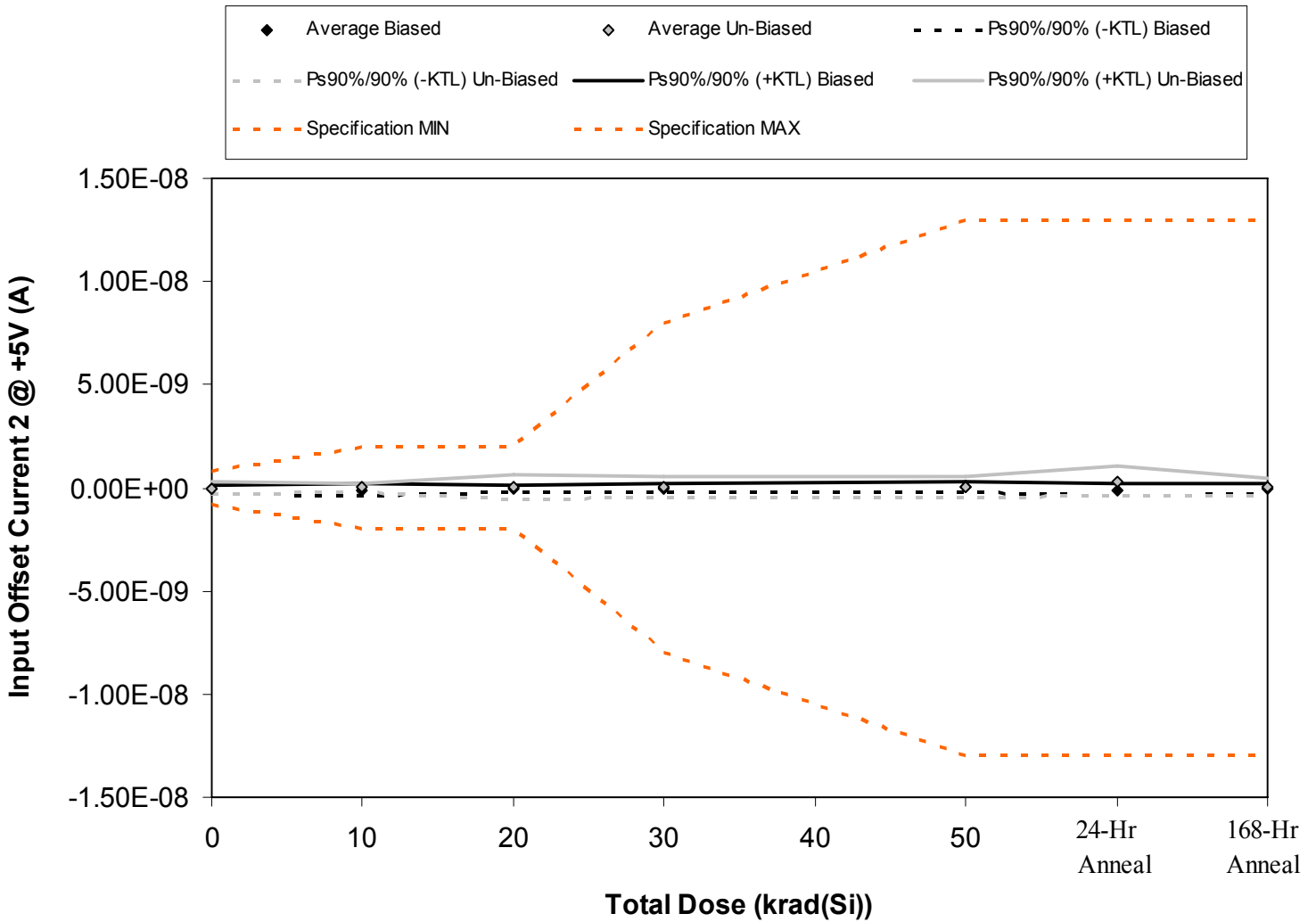
Figure 5.6. Plot of Input Offset Current 2 @ +5V (A) versus total dose. The solid diamonds are the average of the measured data points for the samples irradiated under electrical bias while the shaded diamonds are the average of the measured data points for the samples irradiated with all pins tied to ground. The black lines (solid and/or dashed) are the average of the data points after application of the KTL statistics on the samples irradiated under electrical bias while the gray lines (solid and/or dashed) are the average of the data points after application of the KTL statistics on the samples irradiated in the unbiased condition. The red dotted line(s) are the pre- and/or post-irradiation minimum and/or maximum specification value as defined in the datasheet and/or test plan.
