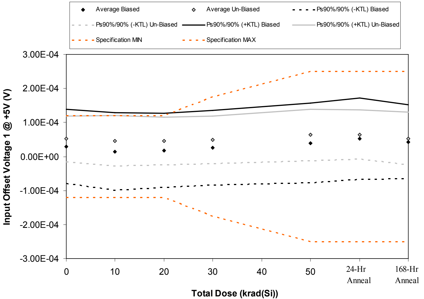
Figure 5.3. Plot of Input Offset Voltage 1 @ +5V (V) versus total dose. The solid diamonds are the average of the measured data points for the samples irradiated under electrical bias while the shaded diamonds are the average of the measured data points for the samples irradiated with all pins tied to ground. The black lines (solid and/or dashed) are the average of the data points after application of the KTL statistics on the samples irradiated under electrical bias while the gray lines (solid and/or dashed) are the average of the data points after application of the KTL statistics on the samples irradiated in the unbiased condition. The red dotted line(s) are the pre- and/or post-irradiation minimum and/or maximum specification value as defined in the datasheet and/or test plan.
