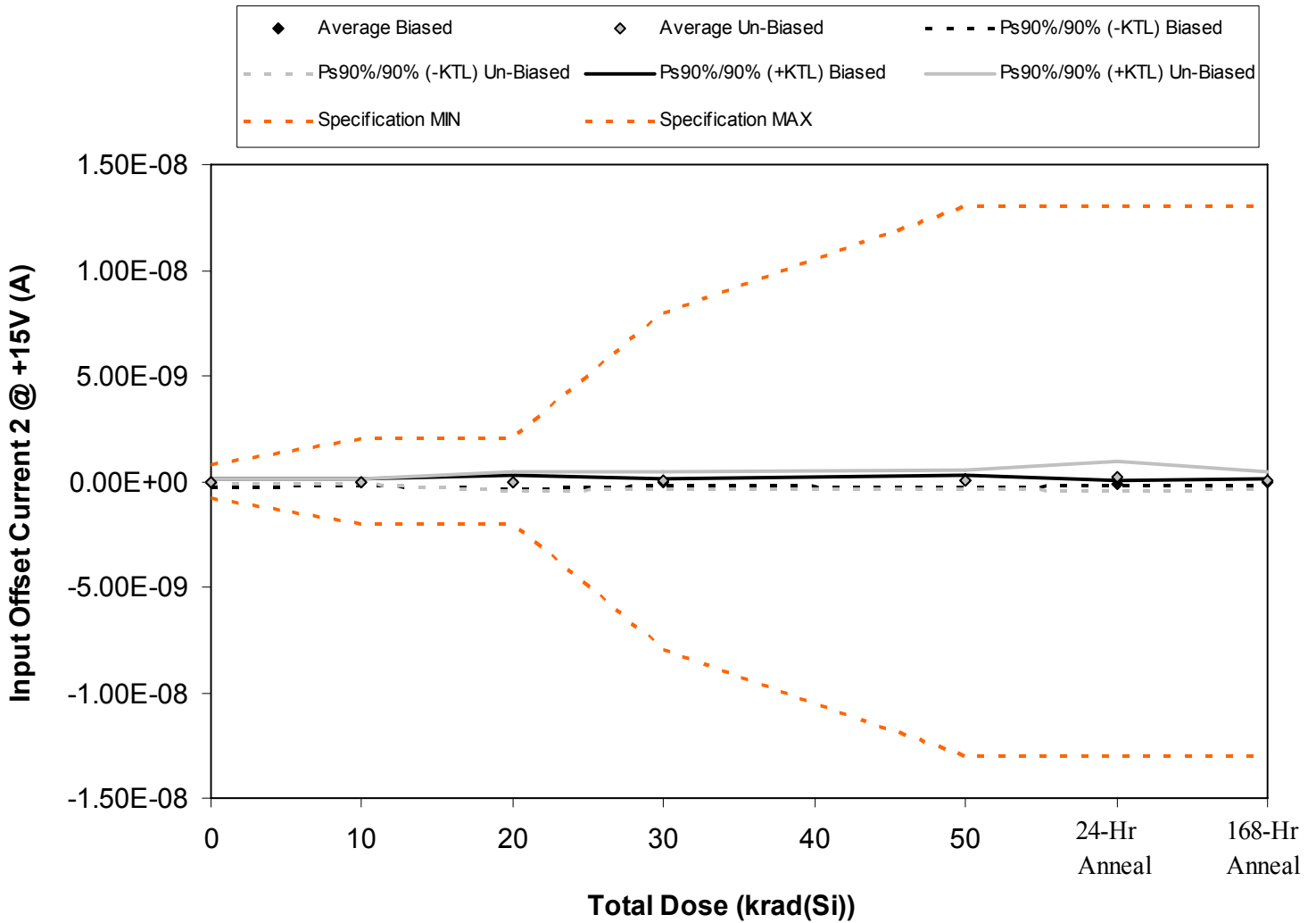
Figure 5.38. Plot of Input Offset Current 2 @ +15V (A) versus total dose. The solid diamonds are the average of the measured data points for the samples irradiated under electrical bias while the shaded diamonds are the average of the measured data points for the samples irradiated with all pins tied to ground. The black lines (solid and/or dashed) are the average of the data points after application of the KTL statistics on the samples irradiated under electrical bias while the gray lines (solid and/or dashed) are the average of the data points after application of the KTL statistics on the samples irradiated in the unbiased condition. The red dotted line(s) are the pre- and/or post-irradiation minimum and/or maximum specification value as defined in the datasheet and/or test plan.
