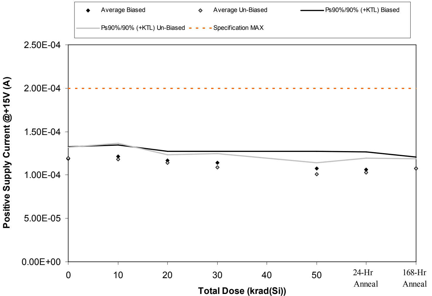
Figure 5.33. Plot of Positive Supply Current @+15V (A) versus total dose. The solid diamonds are the average of the measured data points for the samples irradiated under electrical bias while the shaded diamonds are the average of the measured data points for the samples irradiated with all pins tied to ground. The black lines (solid and/or dashed) are the average of the data points after application of the KTL statistics on the samples irradiated under electrical bias while the gray lines (solid and/or dashed) are the average of the data points after application of the KTL statistics on the samples irradiated in the unbiased condition. The red dotted line(s) are the pre- and/or post-irradiation minimum and/or maximum specification value as defined in the datasheet and/or test plan.
