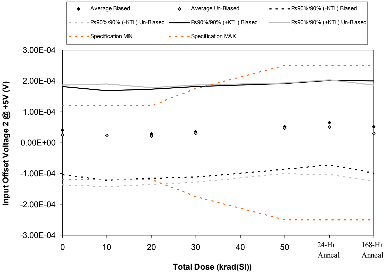
Figure 5.4. Plot of Input Offset Voltage 2 @ +5V (V) versus total dose. The solid diamonds are the average of the measured data points for the samples irradiated under electrical bias while the shaded diamonds are the average of the measured data points for the samples irradiated with all pins tied to ground. The black lines (solid and/or dashed) are the average of the data points after application of the KTL statistics on the samples irradiated under electrical bias while the gray lines (solid and/or dashed) are the average of the data points after application of the KTL statistics on the samples irradiated in the unbiased condition. The red dotted line(s) are the pre- and/or post-irradiation minimum and/or maximum specification value as defined in the datasheet and/or test plan.
