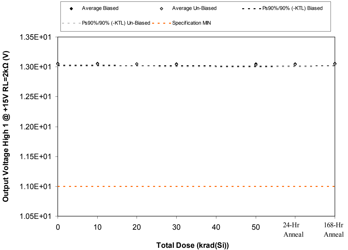
Figure 5.53. Plot of Output Voltage High 1 @ +15V RL=2kΩ (V) versus total dose. The solid diamonds are the average of the measured data points for the samples irradiated under electrical bias while the shaded diamonds are the average of the measured data points for the samples irradiated with all pins tied to ground. The black lines (solid and/or dashed) are the average of the data points after application of the KTL statistics on the samples irradiated under electrical bias while the gray lines (solid and/or dashed) are the average of the data points after application of the KTL statistics on the samples irradiated in the unbiased condition. The red dotted line(s) are the pre- and/or post-irradiation minimum and/or maximum specification value as defined in the datasheet and/or test plan.
