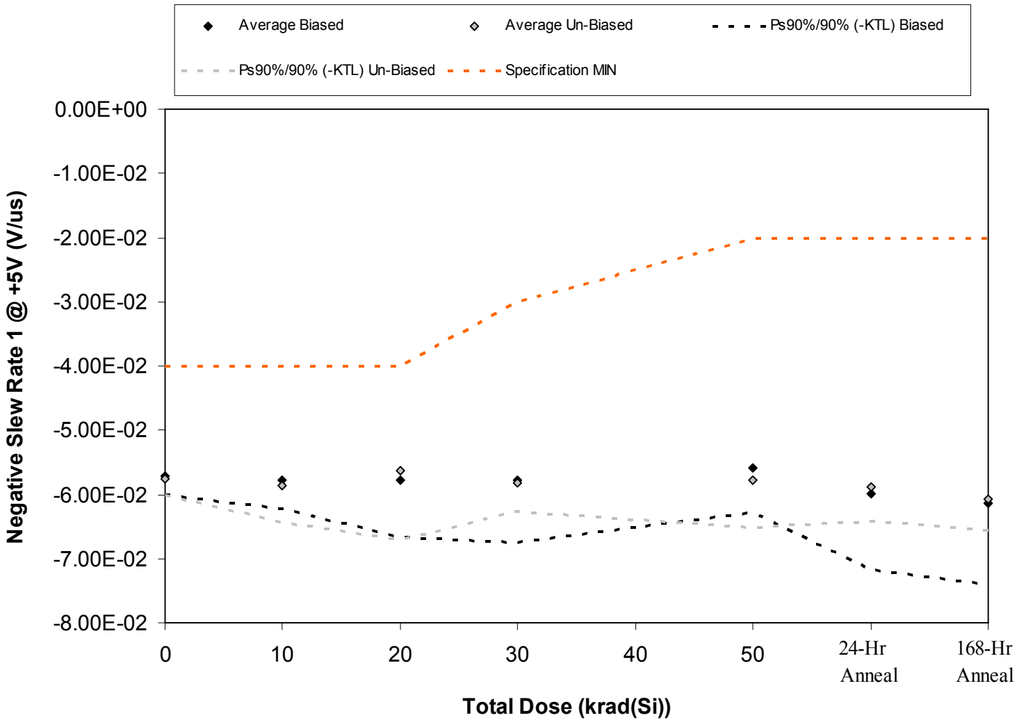
Figure 5.31. Plot of Negative Slew Rate 1 @ +5V (V/us) versus total dose. The solid diamonds are the average of the measured data points for the samples irradiated under electrical bias while the shaded diamonds are the average of the measured data points for the samples irradiated with all pins tied to ground. The black lines (solid and/or dashed) are the average of the data points after application of the KTL statistics on the samples irradiated under electrical bias while the gray lines (solid and/or dashed) are the average of the data points after application of the KTL statistics on the samples irradiated in the unbiased condition. The red dotted line(s) are the pre- and/or post-irradiation minimum and/or maximum specification value as defined in the datasheet and/or test plan.
