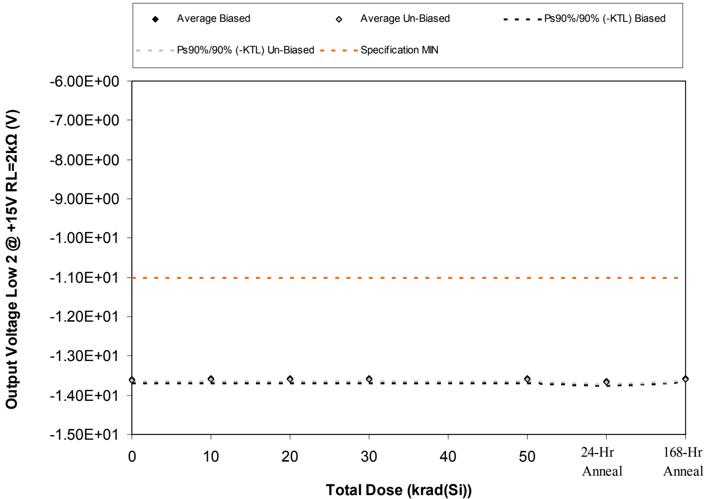
Figure 5.58. Plot of Output Voltage Low 2 @ +15V RL=2kΩ (V) versus total dose. The solid diamonds are the average of the measured data points for the samples irradiated under electrical bias while the shaded diamonds are the average of the measured data points for the samples irradiated with all pins tied to ground. The black lines (solid and/or dashed) are the average of the data points after application of the KTL statistics on the samples irradiated under electrical bias while the gray lines (solid and/or dashed) are the average of the data points after application of the KTL statistics on the samples irradiated in the unbiased condition. The red dotted line(s) are the pre- and/or post-irradiation minimum and/or maximum specification value as defined in the datasheet and/or test plan.
