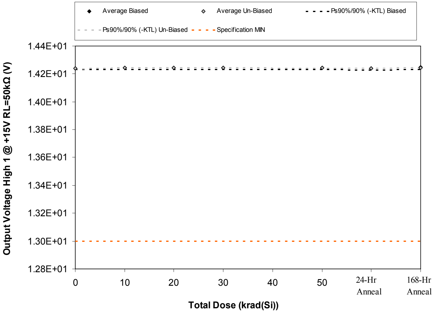
Figure 5.51. Plot of Output Voltage High 1 @ +15V RL=50kΩ (V) versus total dose. The solid diamonds are the average of the measured data points for the samples irradiated under electrical bias while the shaded diamonds are the average of the measured data points for the samples irradiated with all pins tied to ground. The black lines (solid and/or dashed) are the average of the data points after application of the KTL statistics on the samples irradiated under electrical bias while the gray lines (solid and/or dashed) are the average of the data points after application of the KTL statistics on the samples irradiated in the unbiased condition. The red dotted line(s) are the pre- and/or post-irradiation minimum and/or maximum specification value as defined in the datasheet and/or test plan.
