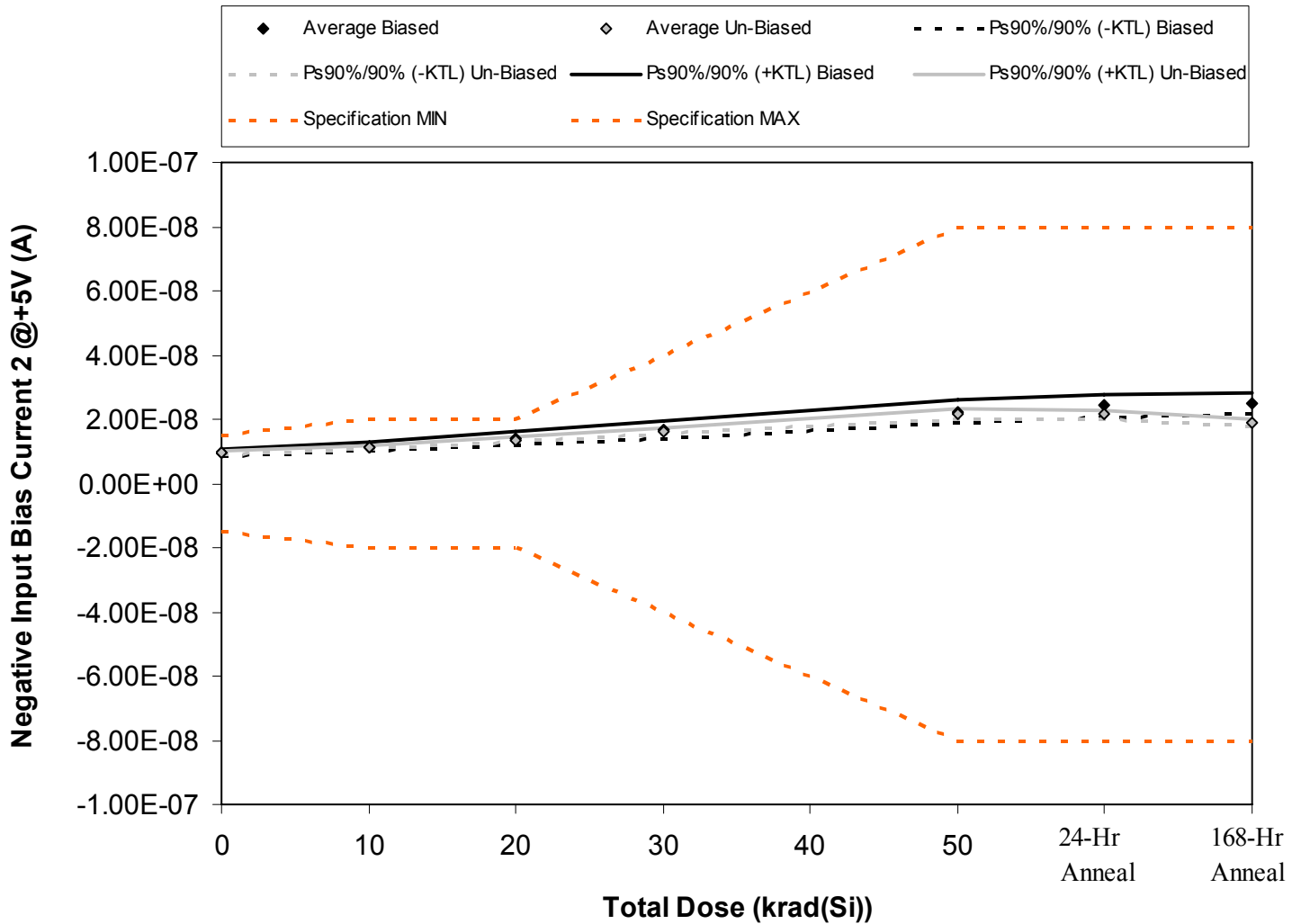
Figure 5.10. Plot of Negative Input Bias Current 2 @+5V (A) versus total dose. The solid diamonds are the average of the measured data points for the samples irradiated under electrical bias while the shaded diamonds are the average of the measured data points for the samples irradiated with all pins tied to ground. The black lines (solid and/or dashed) are the average of the data points after application of the KTL statistics on the samples irradiated under electrical bias while the gray lines (solid and/or dashed) are the average of the data points after application of the KTL statistics on the samples irradiated in the unbiased condition. The red dotted line(s) are the pre- and/or post-irradiation minimum and/or maximum specification value as defined in the datasheet and/or test plan.
