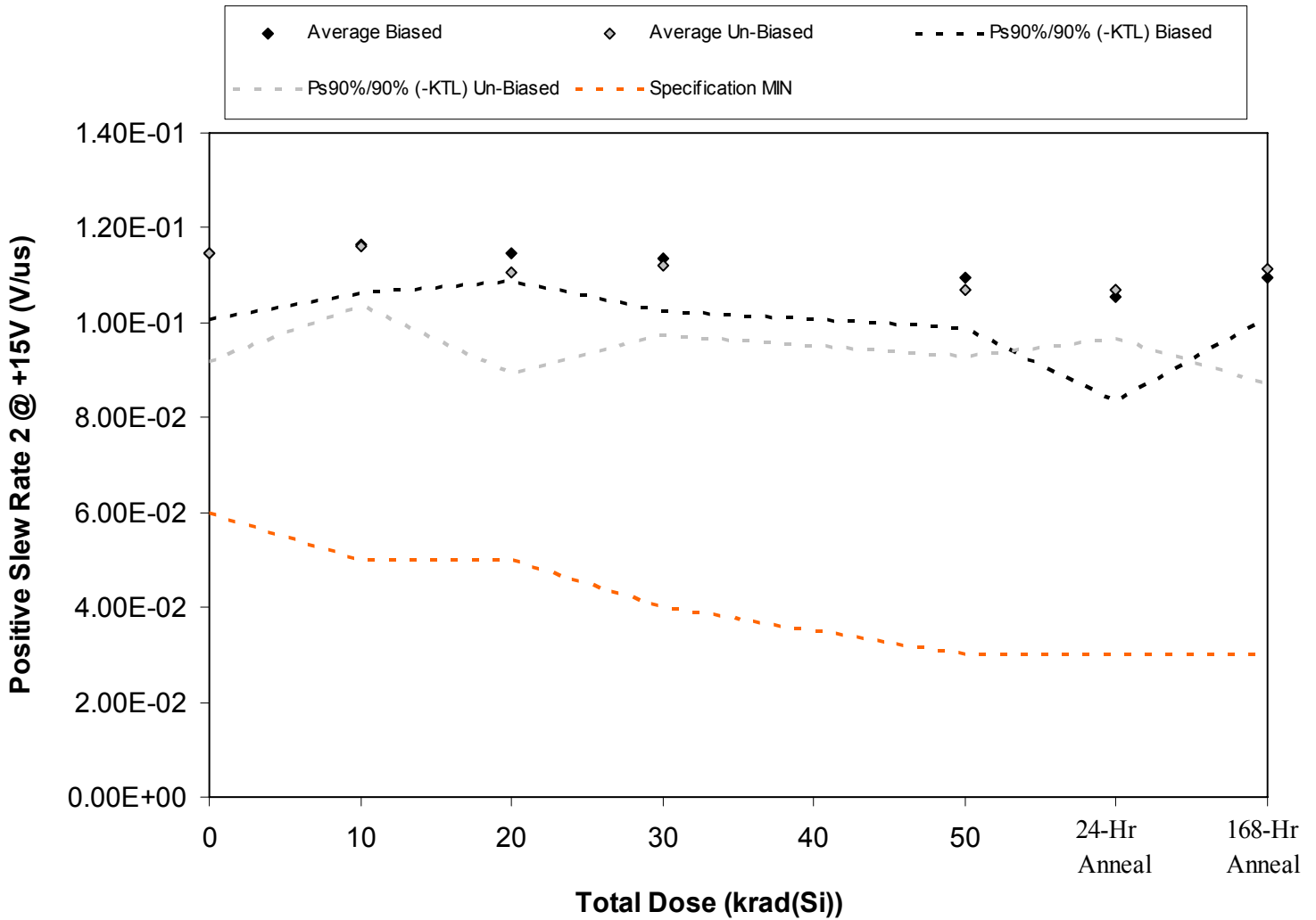
Figure 5.60. Plot of Positive Slew Rate 2 @ +15V (V/us) versus total dose. The solid diamonds are the average of the measured data points for the samples irradiated under electrical bias while the shaded diamonds are the average of the measured data points for the samples irradiated with all pins tied to ground. The black lines (solid and/or dashed) are the average of the data points after application of the KTL statistics on the samples irradiated under electrical bias while the gray lines (solid and/or dashed) are the average of the data points after application of the KTL statistics on the samples irradiated in the unbiased condition. The red dotted line(s) are the pre- and/or post-irradiation minimum and/or maximum specification value as defined in the datasheet and/or test plan.
