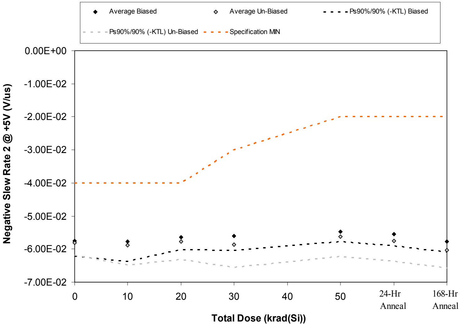
Figure 5.32. Plot of Negative Slew Rate 2 @ +5V (V/us) versus total dose. The solid diamonds are the average of the measured data points for the samples irradiated under electrical bias while the shaded diamonds are the average of the measured data points for the samples irradiated with all pins tied to ground. The black lines (solid and/or dashed) are the average of the data points after application of the KTL statistics on the samples irradiated under electrical bias while the gray lines (solid and/or dashed) are the average of the data points after application of the KTL statistics on the samples irradiated in the unbiased condition. The red dotted line(s) are the pre- and/or post-irradiation minimum and/or maximum specification value as defined in the datasheet and/or test plan.
