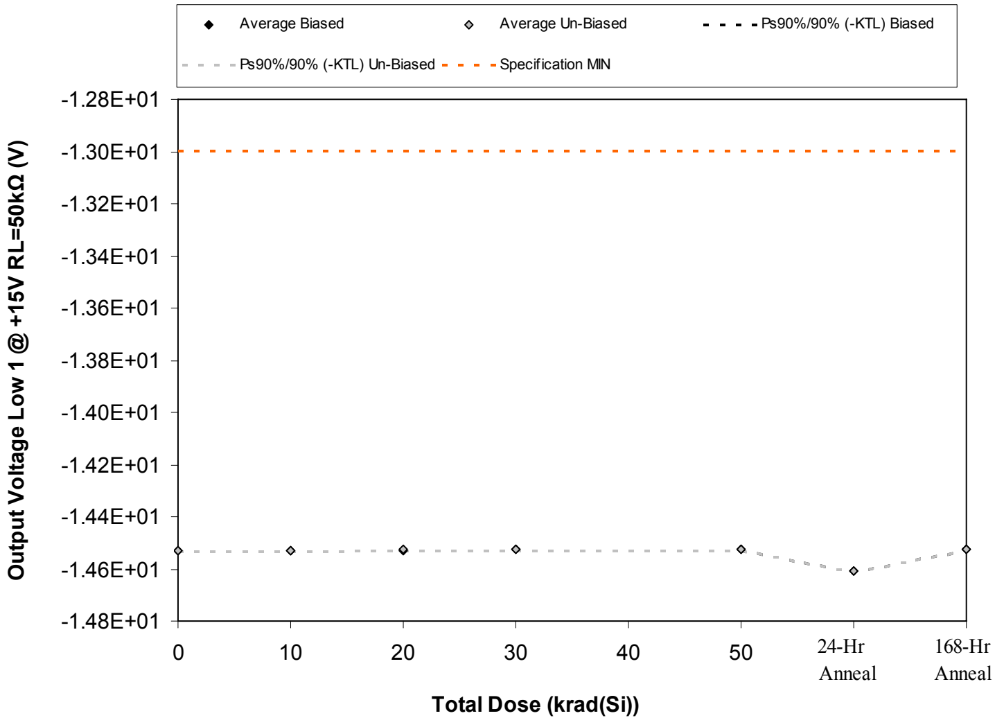
Figure 5.55. Plot of Output Voltage Low 1 @ +15V RL=50kΩ (V) versus total dose. The solid diamonds are the average of the measured data points for the samples irradiated under electrical bias while the shaded diamonds are the average of the measured data points for the samples irradiated with all pins tied to ground. The black lines (solid and/or dashed) are the average of the data points after application of the KTL statistics on the samples irradiated under electrical bias while the gray lines (solid and/or dashed) are the average of the data points after application of the KTL statistics on the samples irradiated in the unbiased condition. The red dotted line(s) are the pre- and/or post-irradiation minimum and/or maximum specification value as defined in the datasheet and/or test plan.
