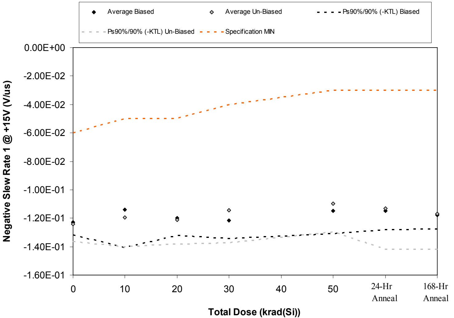
Figure 5.61. Plot of Negative Slew Rate 1 @ +15V (V/us) versus total dose. The solid diamonds are the average of the measured data points for the samples irradiated under electrical bias while the shaded diamonds are the average of the measured data points for the samples irradiated with all pins tied to ground. The black lines (solid and/or dashed) are the average of the data points after application of the KTL statistics on the samples irradiated under electrical bias while the gray lines (solid and/or dashed) are the average of the data points after application of the KTL statistics on the samples irradiated in the unbiased condition. The red dotted line(s) are the pre- and/or post-irradiation minimum and/or maximum specification value as defined in the datasheet and/or test plan.
