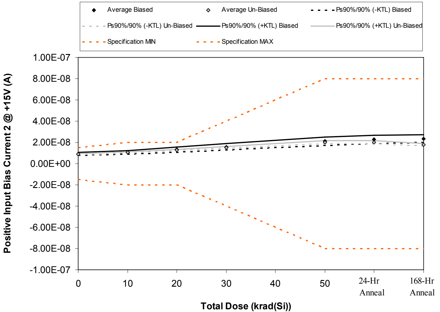
Figure 5.40. Plot of Positive Input Bias Current 2 @ +15V (A) versus total dose. The solid diamonds are the average of the measured data points for the samples irradiated under electrical bias while the shaded diamonds are the average of the measured data points for the samples irradiated with all pins tied to ground. The black lines (solid and/or dashed) are the average of the data points after application of the KTL statistics on the samples irradiated under electrical bias while the gray lines (solid and/or dashed) are the average of the data points after application of the KTL statistics on the samples irradiated in the unbiased condition. The red dotted line(s) are the pre- and/or post-irradiation minimum and/or maximum specification value as defined in the datasheet and/or test plan.
