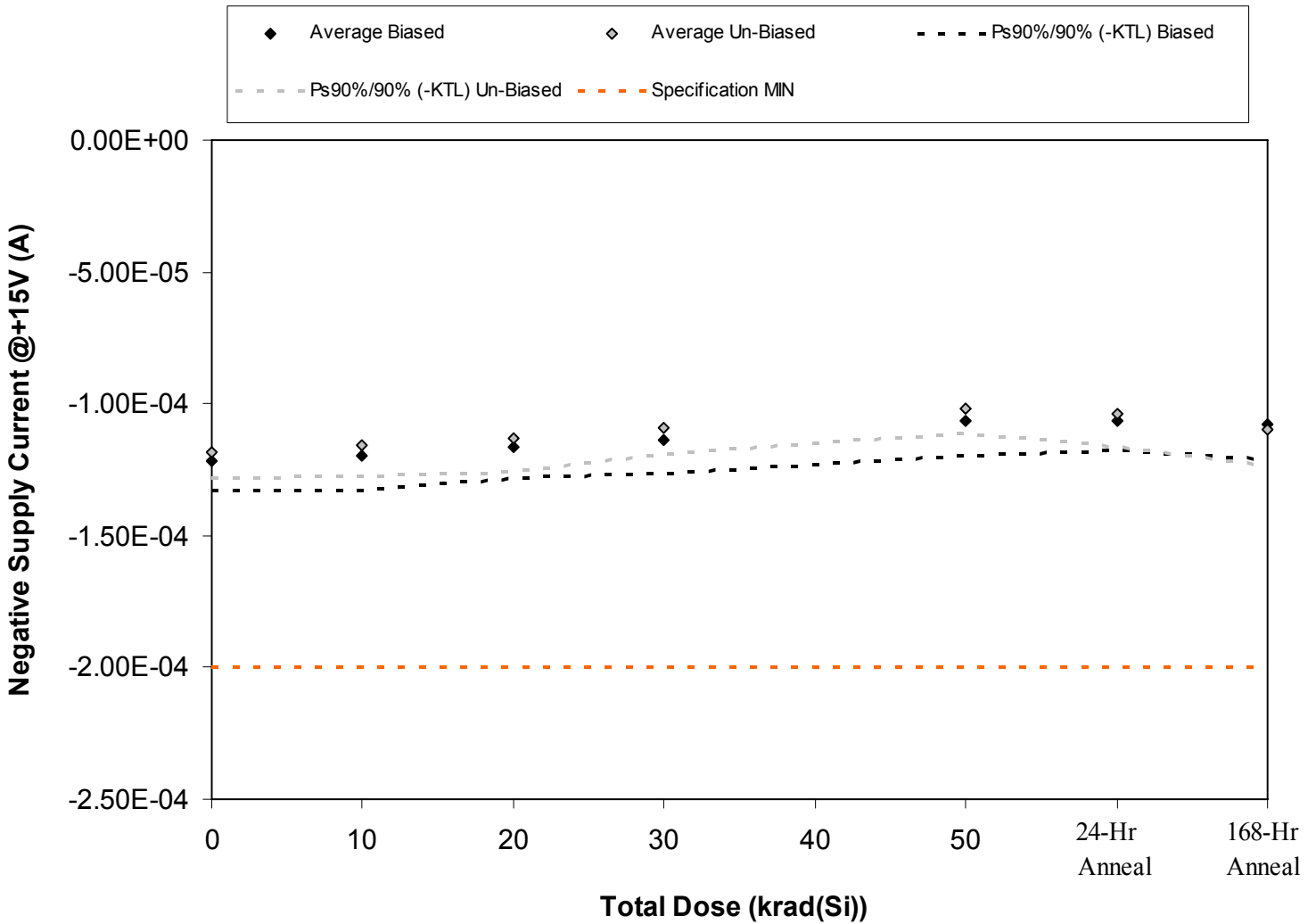
Figure 5.34. Plot of Negative Supply Current @+15V (A) versus total dose. The solid diamonds are the average of the measured data points for the samples irradiated under electrical bias while the shaded diamonds are the average of the measured data points for the samples irradiated with all pins tied to ground. The black lines (solid and/or dashed) are the average of the data points after application of the KTL statistics on the samples irradiated under electrical bias while the gray lines (solid and/or dashed) are the average of the data points after application of the KTL statistics on the samples irradiated in the unbiased condition. The red dotted line(s) are the pre- and/or post-irradiation minimum and/or maximum specification value as defined in the datasheet and/or test plan.
