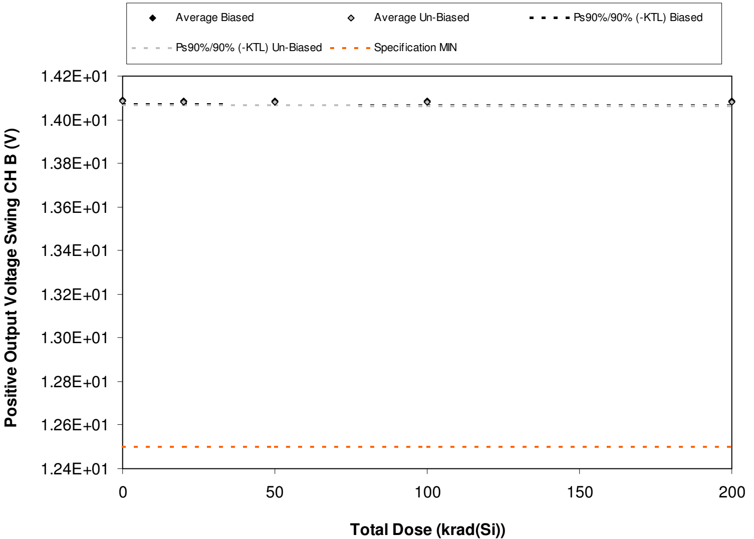
Figure 5.18. Plot of positive output voltage swing for channel B versus total dose. The data show no significant decrease with total dose. The solid diamonds are the average of measured data points from the biased sample (devices irradiated with an electrical bias) while the shaded diamonds are the average from the un-biased sample. The black lines show the effects on the data after application of the biased KTL statistics (solid and/or dashed lines) while the gray lines show the effects on the data after application of the unbiased KTL statistics (solid and/or dashed lines). The red dashed lines are the minimum and/or maximum specification values as defined in the datasheet and/or test plan.
