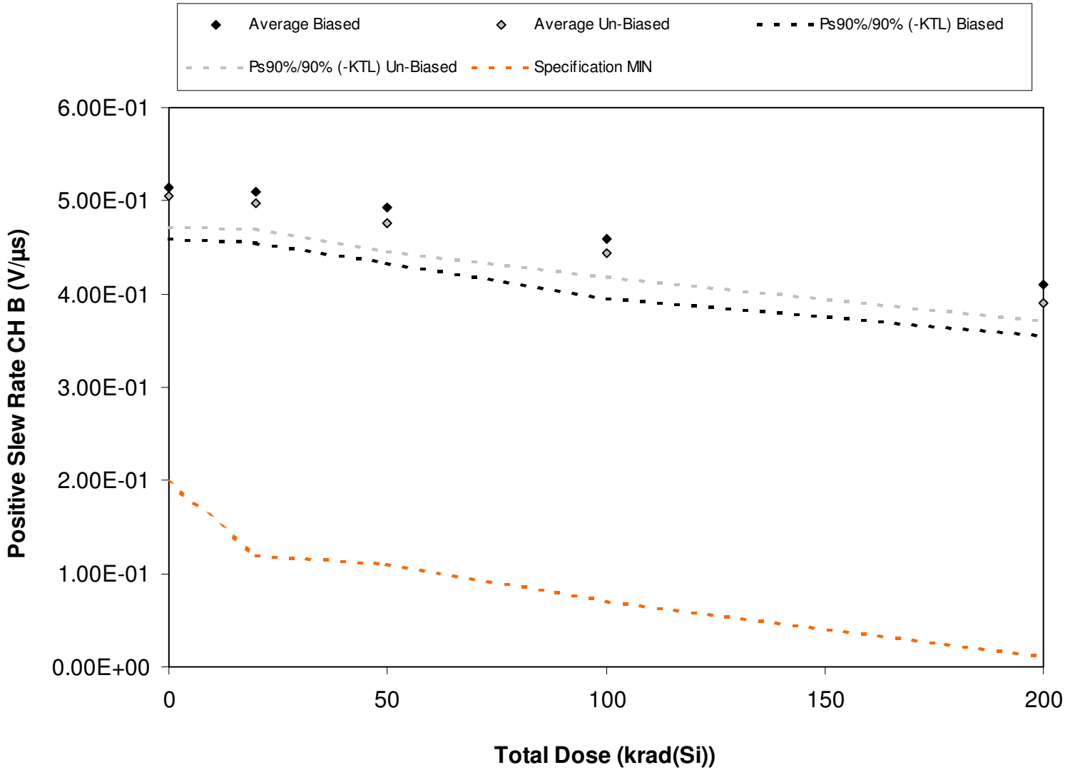
Figure 5.22. Plot of positive slew rate for channel B versus total dose. The data show a moderate decrease with total dose, however not sufficient to fall below the specification, even after application of the KTL statistics. The solid diamonds are the average of measured data points from the biased sample (devices irradiated with an electrical bias) while the shaded diamonds are the average from the un-biased sample. The black lines show the effects on the data after application of the biased KTL statistics (solid and/or dashed lines) while the gray lines show the effects on the data after application of the unbiased KTL statistics (solid and/or dashed lines). The red dashed lines are the minimum and/or maximum specification values as defined in the datasheet and/or test plan.
