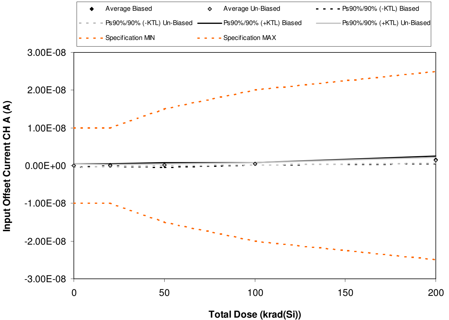
Figure 5.5. Plot of input offset current, channel A @ +/-15V (A) versus total dose. The data show no significant degradation with total dose, however the degradation is not sufficient to cause the KTL statistics to go out of specification. The solid diamonds are the average of measured data points from the biased sample (devices irradiated with an electrical bias) while the shaded diamonds are the average from the un-biased sample. The black lines show the effects on the data after application of the biased KTL statistics (solid and dashed lines) while the gray lines show the effects on the data after application of the unbiased KTL statistics (solid and dashed lines). The red dashed lines are the minimum and maximum specification values as defined in the datasheet and/or test plan.
