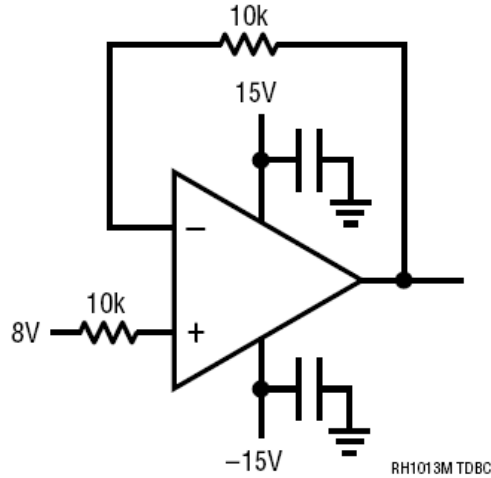
Figure A.1. Irradiation bias drawing for the units to be irradiated under electrical bias. This figure was extracted from the LINEAR TECHNOLOGY CORPORATION RH1013M Dual Precision Operational Amplifier Datasheet.
