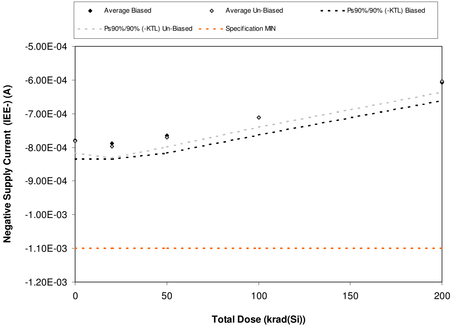
Figure 5.2. Plot of Negative Supply Current @ +/-15V (A) versus total dose. The data show a general improvement with total dose. The solid diamonds are the average of the measured data points for the sample irradiated under electrical bias while the shaded diamonds are the average of the measured data points for the units irradiated with all pins tied to ground. The black lines (solid or dashed) are the average of the data points after application of the KTL statistics on the sample irradiated in the biased condition while the shaded lines (solid or dashed) are the average of the data points after application of the KTL statistics on the sample irradiated in the unbiased condition. The red dotted line(s) are the pre- and/or post-irradiation minimum and/or maximum specification value as defined in the datasheet and/or test plan.
