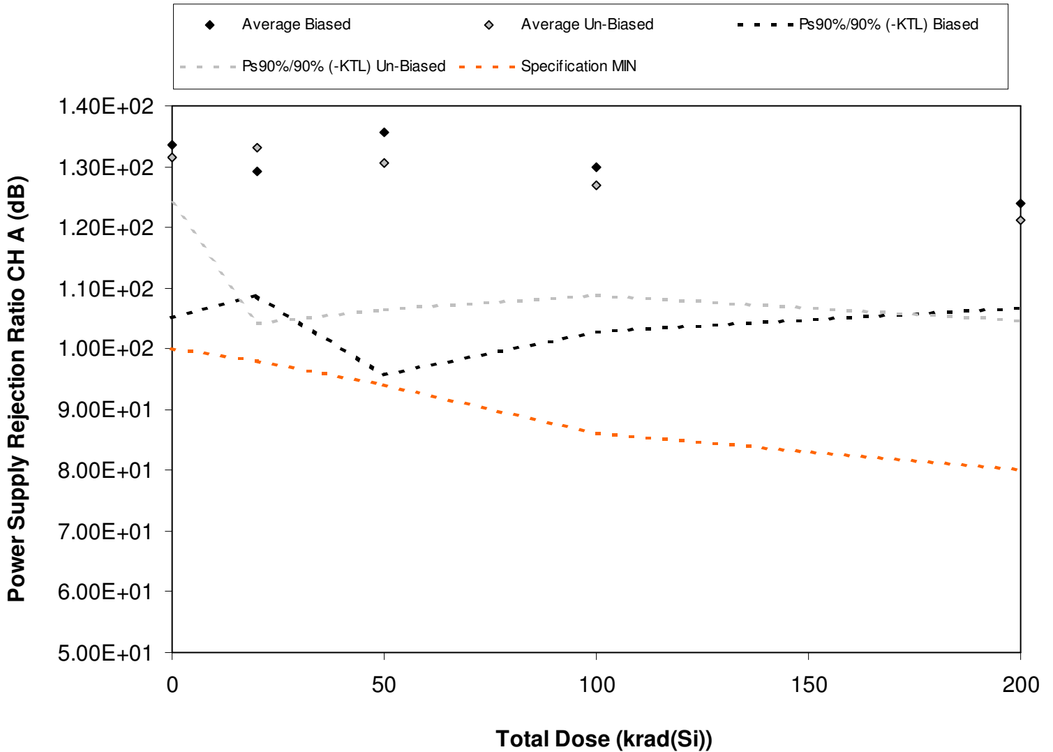
Figure 5.13. Plot of power supply rejection ratio for channel A versus total dose. Although the data show a decrease with total dose, it is not sufficient to fall below the specification value. The solid diamonds are the average of measured data points from the biased sample (devices irradiated with an electrical bias) while the shaded diamonds are the average from the un-biased sample. The black lines show the effects on the data after application of the biased KTL statistics (solid and/or dashed lines) while the gray lines show the effects on the data after application of the unbiased KTL statistics (solid and/or dashed lines). The red dashed lines are the minimum and/or maximum specification values as defined in the datasheet and/or test plan.
