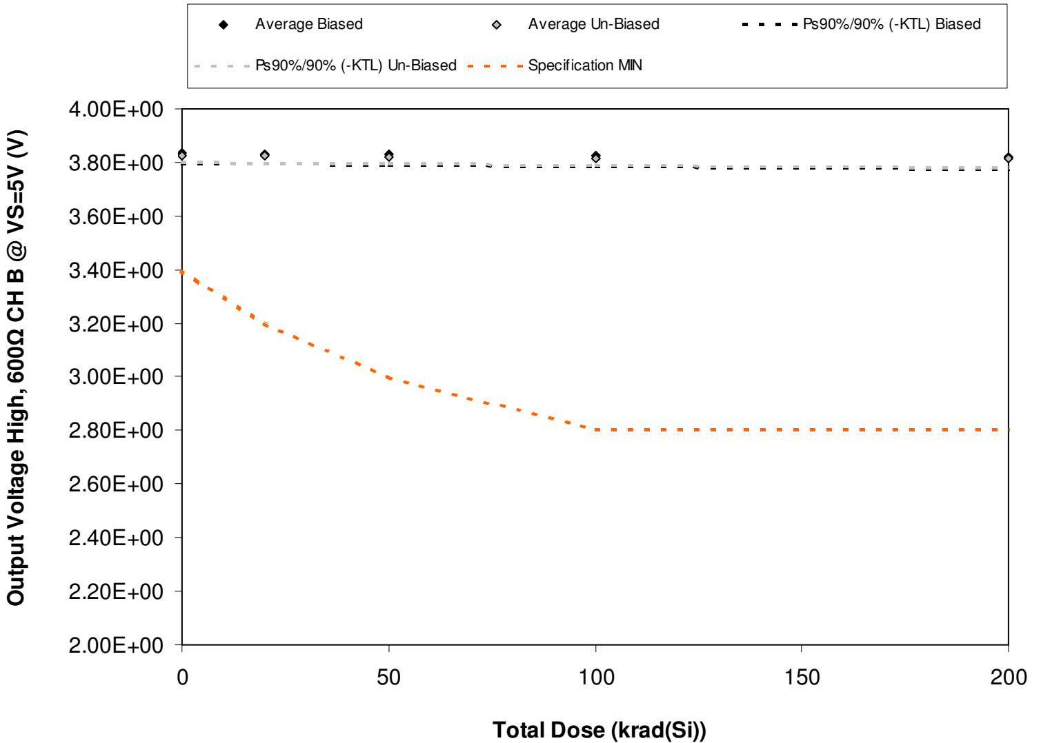
Figure 5.38. Plot of the output voltage high (600Ω load) at 5V for channel B versus total dose. The data show no significant change with total dose. The solid diamonds are the average of measured data points from the biased sample (devices irradiated with an electrical bias) while the shaded diamonds are the average from the un-biased sample. The black line(s) show the effects on the data after application of the biased KTL statistics (solid and/or dashed lines) while the gray line(s) show the effects on the data after application of the unbiased KTL statistics (solid and/or dashed lines). The red dashed line(s) are the minimum and/or maximum specification values as defined in the datasheet and/or test plan.
