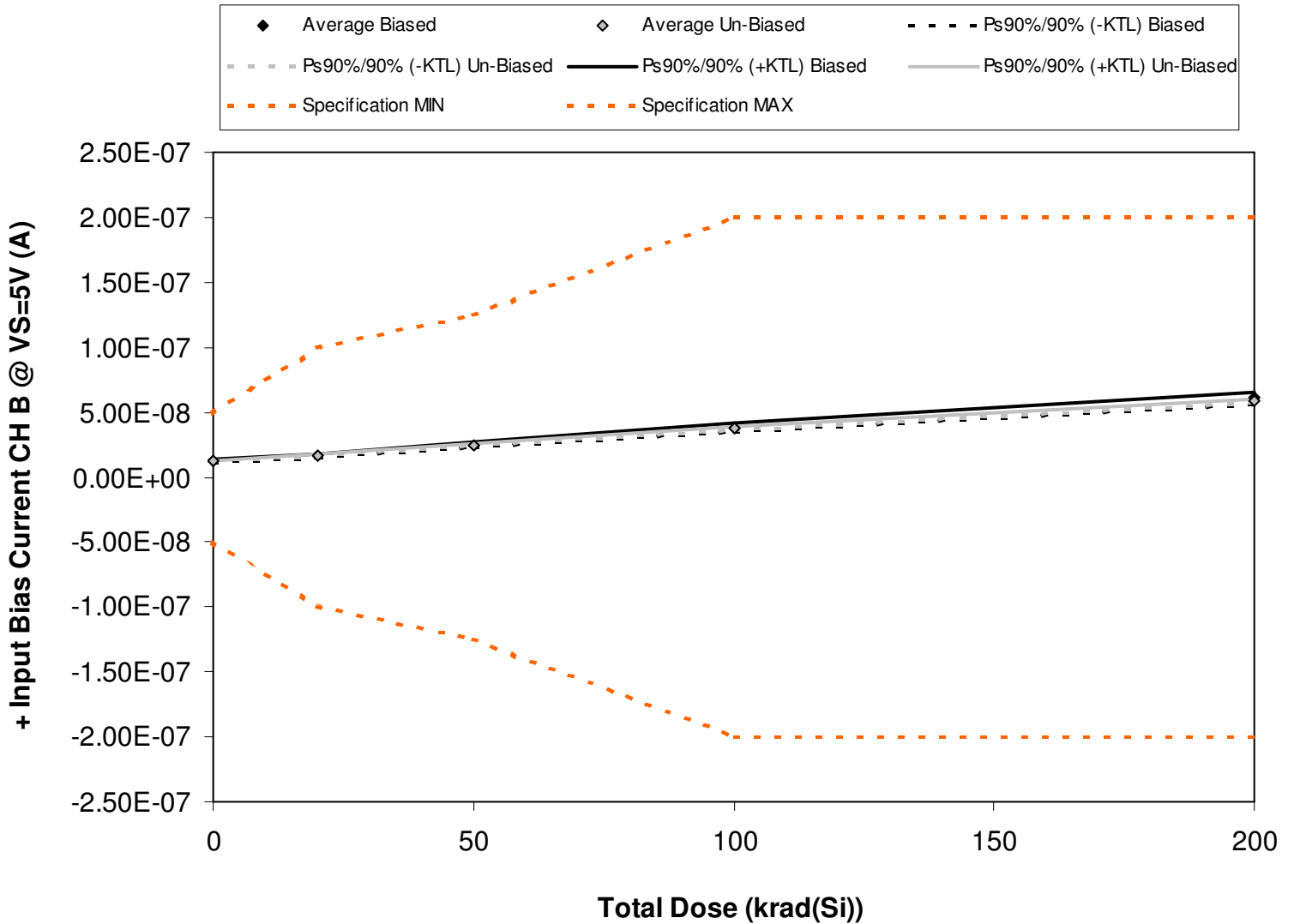
Figure 5.32. Plot of input bias current, non-inverting input at 5V for channel B versus total dose. The data show a slight increase with total dose, however not sufficient for the parameter to exceed specification, including after application of the KTL statistics. The solid diamonds are the average of measured data points from the biased sample (devices irradiated with an electrical bias) while the shaded diamonds are the average from the un-biased sample. The black line(s) show the effects on the data after application of the biased KTL statistics (solid and/or dashed lines) while the gray line(s) show the effects on the data after application of the unbiased KTL statistics (solid and/or dashed lines). The red dashed line(s) are the minimum and/or maximum specification values as defined in the datasheet and/or test plan.
