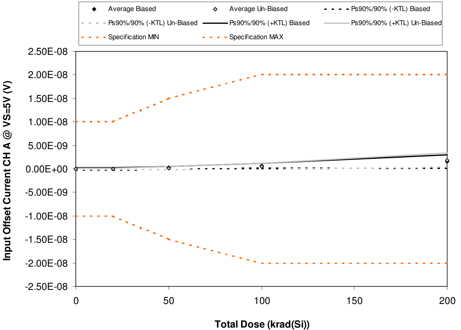
Figure 5.29. Plot of input offset current at 5V for channel A versus total dose. The data show a very slight increase with total dose, however not sufficient for the parameter to exceed specification, including after application of the KTL statistics. The solid diamonds are the average of measured data points from the biased sample (devices irradiated with an electrical bias) while the shaded diamonds are the average from the un-biased sample. The black line(s) show the effects on the data after application of the biased KTL statistics (solid and/or dashed lines) while the gray line(s) show the effects on the data after application of the unbiased KTL statistics (solid and/or dashed lines). The red dashed line(s) are the minimum and/or maximum specification values as defined in the datasheet and/or test plan.
