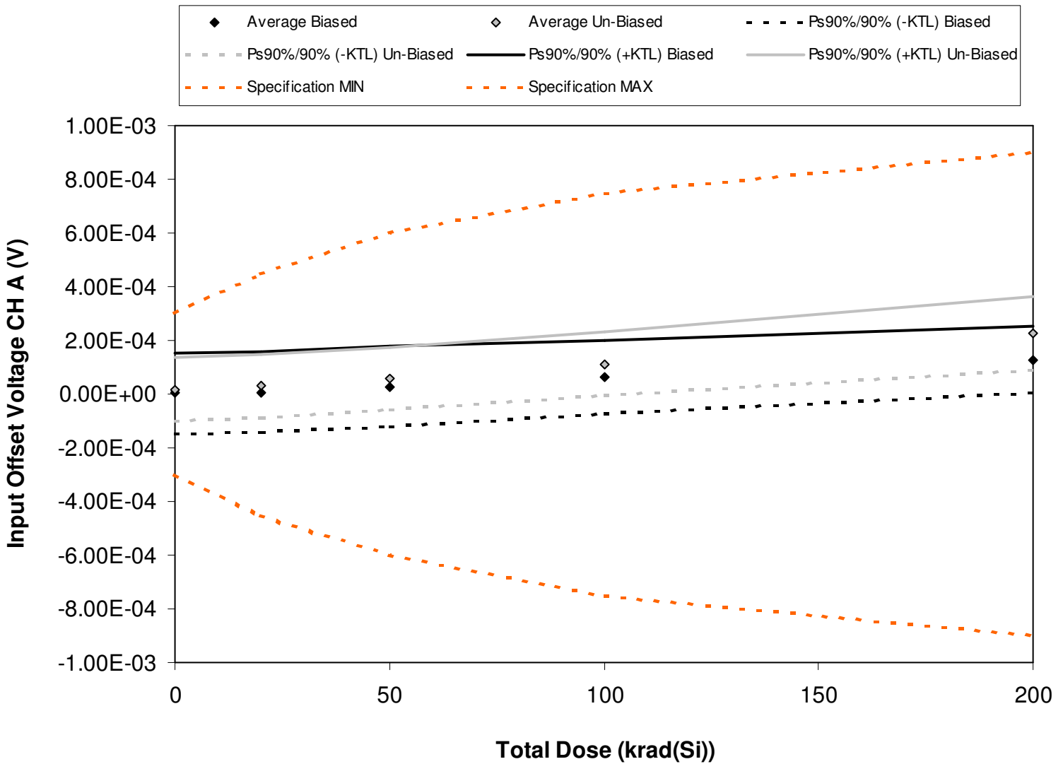
Figure 5.3. Plot of input offset voltage for channel A @ +/-15V (A) versus total dose. The data show some increase with total dose. The solid diamonds are the average of the measured data points for the sample irradiated under electrical bias while the shaded diamonds are the average of the measured data points for the units irradiated with all pins tied to ground. The black lines (solid or dashed) are the average of the data points after application of the KTL statistics on the sample irradiated in the biased condition while the shaded lines (solid or dashed) are the average of the data points after application of the KTL statistics on the sample irradiated in the unbiased condition. The red dotted line(s) are the pre- and/or post-irradiation minimum and/or maximum specification value as defined in the datasheet and/or test plan
