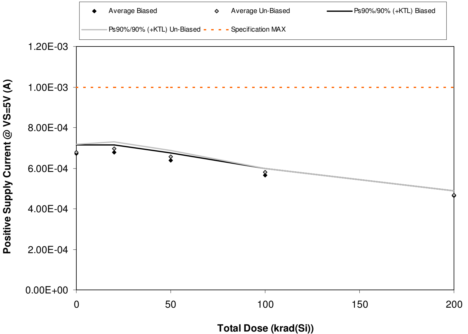
Figure 5.25. Plot of positive supply current at 5V versus total dose. The data show a slight decrease (improvement) with total dose. The solid diamonds are the average of measured data points from the biased sample (devices irradiated with an electrical bias) while the shaded diamonds are the average from the unbiased sample. The black line(s) show the effects on the data after application of the biased KTL statistics (solid and/or dashed lines) while the gray line(s) show the effects on the data after application of the unbiased KTL statistics (solid and/or dashed lines). The red dashed line(s) are the minimum and/or maximum specification values as defined in the datasheet and/or test plan.
