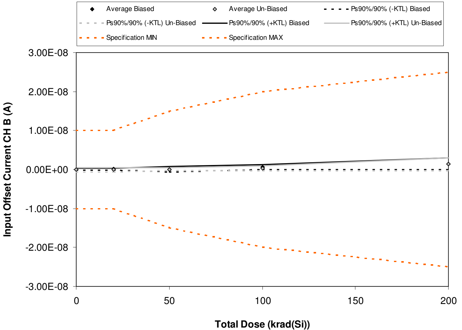
Figure 5.6. Plot of input offset current, channel B @ +/-15V (A) versus total dose. The data show no significant degradation with total dose, however the degradation is not sufficient to cause the KTL statistics to go out of specification. The solid diamonds are the average of measured data points from the biased sample (devices irradiated with an electrical bias) while the shaded diamonds are the average from the un-biased sample. The black lines show the effects on the data after application of the biased KTL statistics (solid and dashed lines) while the gray lines show the effects on the data after application of the unbiased KTL statistics (solid and dashed lines). The red dashed lines are the minimum and maximum specification values as defined in the datasheet and/or test plan.
