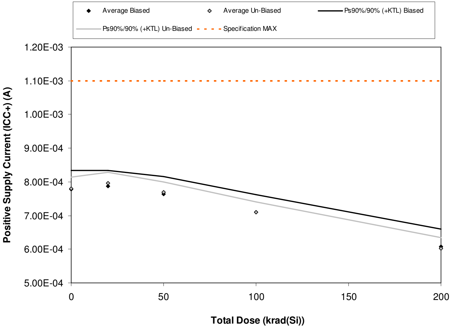
Figure 5.1. Plot of positive supply current ( \pm 15V ) versus total dose. The data shows a general improvement with total dose. The solid diamonds are the average of the measured data points for the sample irradiated under electrical bias while the shaded diamonds are the average of the measured data points for the units irradiated with all pins tied to ground. The black lines (solid or dashed) are the average of the data points after application of the KTL statistics on the sample irradiated in the biased condition while the shaded lines (solid or dashed) are the average of the data points after application of the KTL statistics on the sample irradiated in the unbiased condition. The red dotted line(s) are the pre- and/or post-irradiation minimum and/or maximum specification value as defined in the datasheet and/or test plan.
