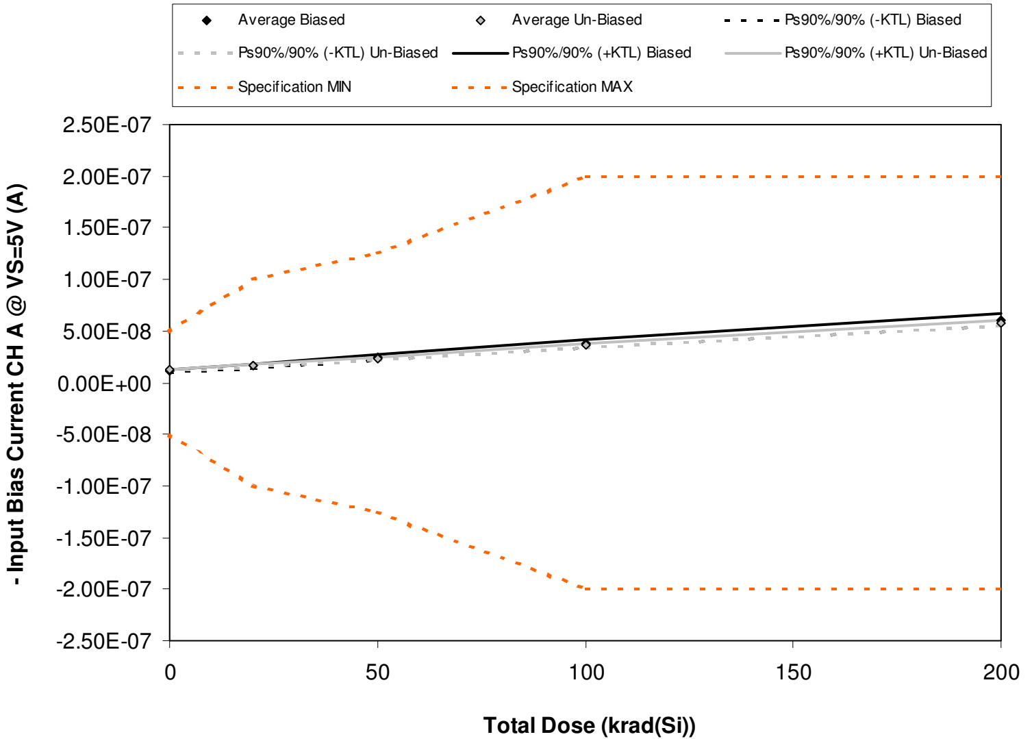
Figure 5.33. Plot of input bias current, inverting input at 5V for channel A versus total dose. The data show a slight increase with total dose, however not sufficient for the parameter to exceed specification, including after application of the KTL statistics. The solid diamonds are the average of measured data points from the biased sample (devices irradiated with an electrical bias) while the shaded diamonds are the average from the un-biased sample. The black line(s) show the effects on the data after application of the biased KTL statistics (solid and/or dashed lines) while the gray line(s) show the effects on the data after application of the unbiased KTL statistics (solid and/or dashed lines). The red dashed line(s) are the minimum and/or maximum specification values as defined in the datasheet and/or test plan.
