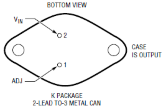
Figure B.2. K Package drawing (for reference only). This figure was extracted from Linear Technology Linear Technology RH117 Datasheet Revision B.
