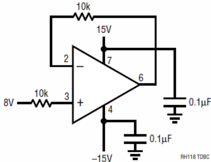
Figure B.1. Irradiation bias circuit. This figure was extracted from Linear Technology RH118 Datasheet. Pin Numbers refers to the H or J8 package, not the W package tested here.
