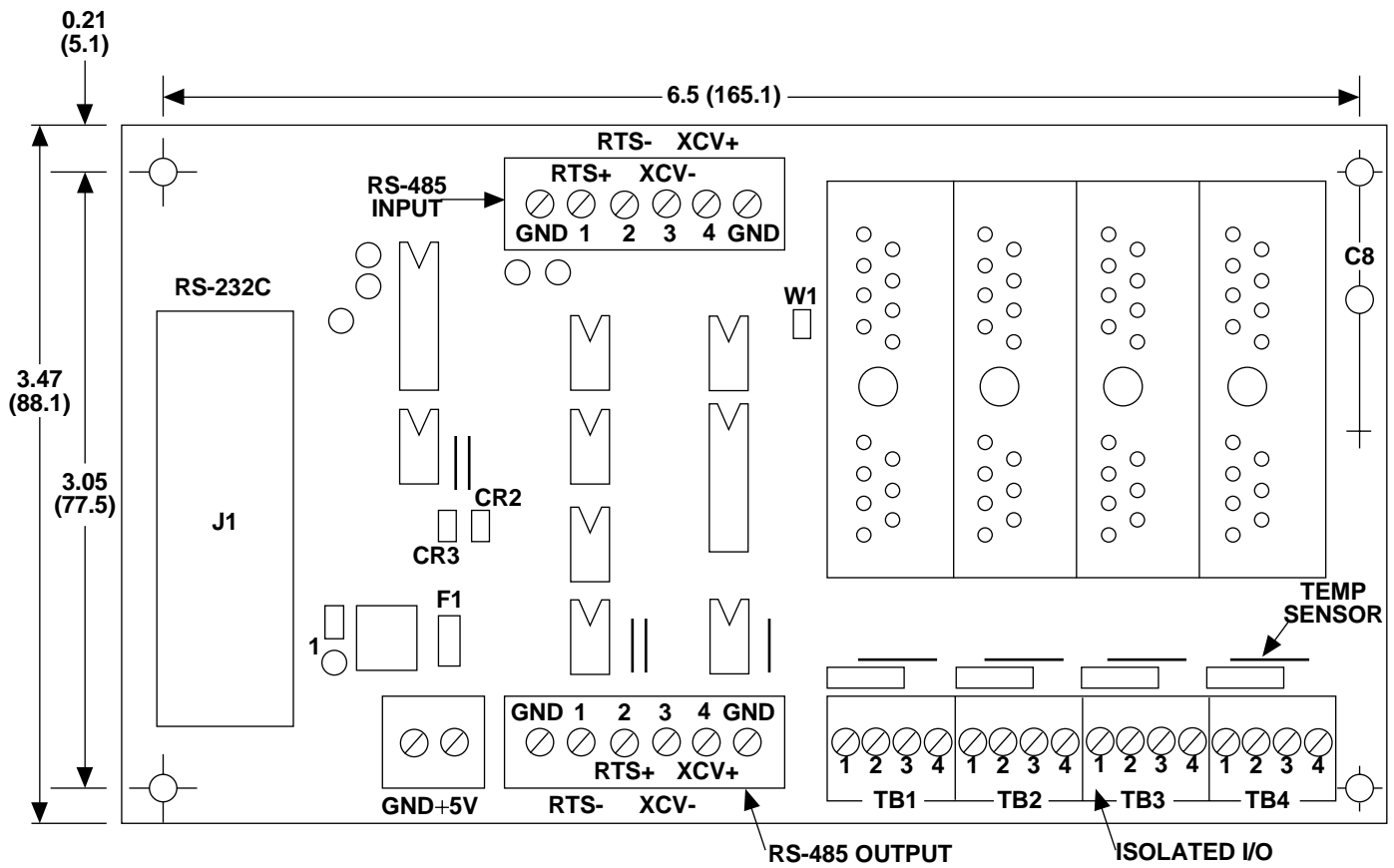
Models 6BP04-1, 6BP04HV-1, 6BP04-2, and 6BP04HV-2 Backplanes.
