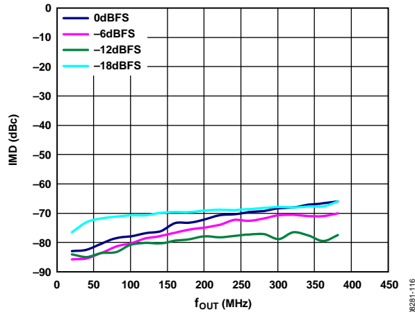
Figure 19. IMD vs. f_{OUT} over Digital Scale, 2x Interpolation, f_{DATA} = 400 MSPS, f_{SC} = 20 mA
