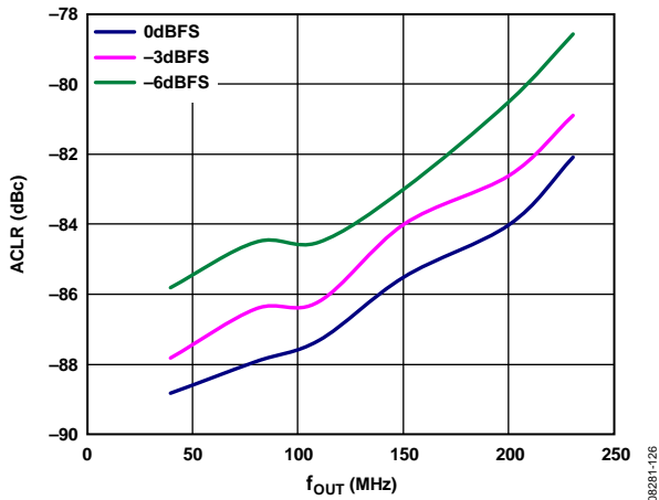
Figure 29. 1-Carrier W-CDMA ACLR vs. f_{OUT} over f_{DAC} , Alternate Channel, PLL Off
