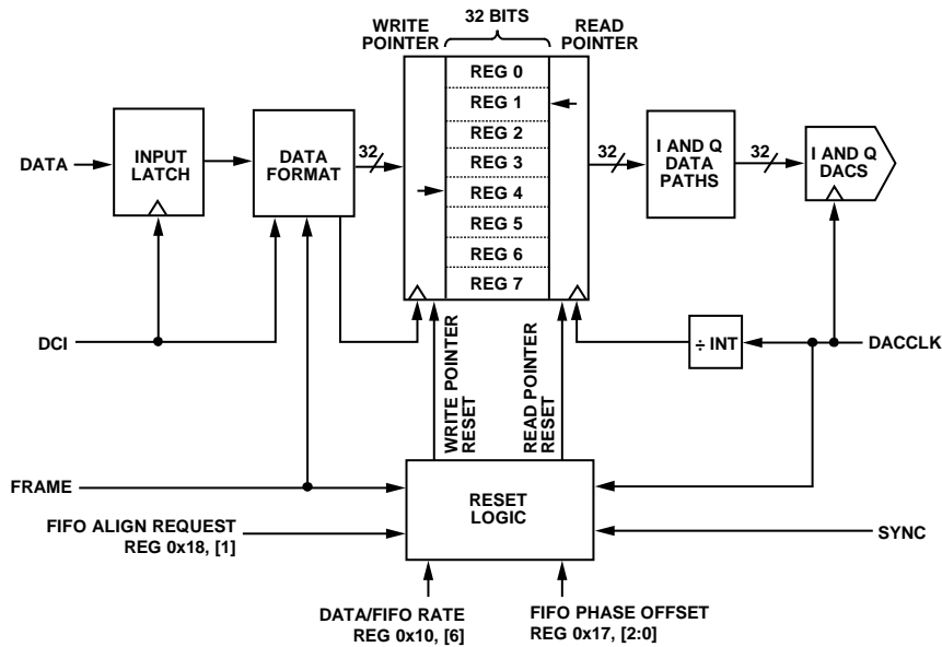
Figure 47. Block Diagram of FIFO
