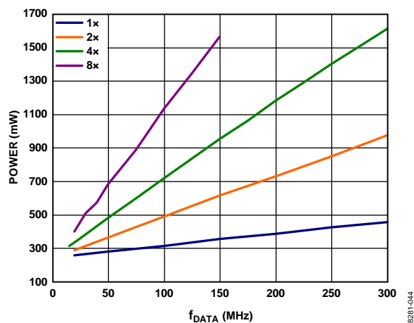
Figure 76. Total Power Dissipation vs. f_{DATA} Without PLL, Fine NCO, and Inverse Sinc
