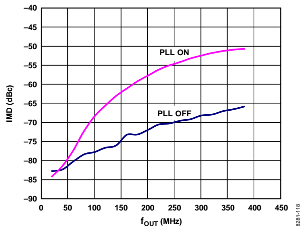
Figure 21. IMD vs. f_{OUT} , PLL On vs. PLL Off, 4x Interpolation, f_{DATA} = 200 MSPS, Digital Scale = 0 dBFS, f_{SC} = 20 mA
