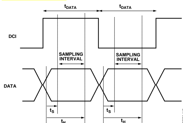
Figure 44. Timing Diagram for Input Data Ports
