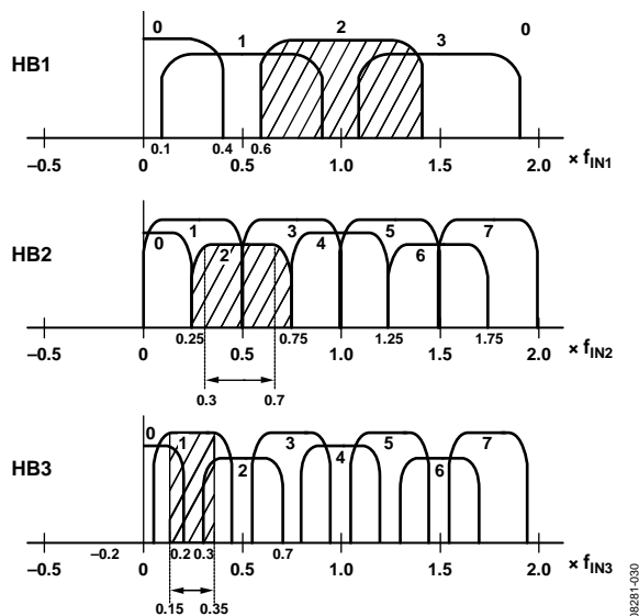
Figure 60. Signal Propagation for 8x Interpolation ( f_{DATA} Modulation)
