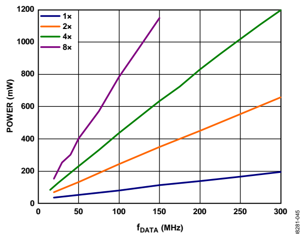
Figure 77. DVDD18 Power Dissipation vs. f_{DATA} Without Fine NCO and Inverse Sinc
