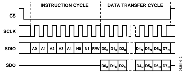
Figure 40. Serial Register Interface Timing LSB-First
