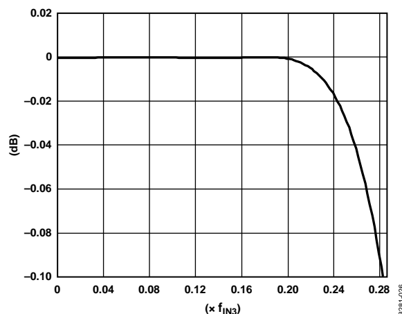
Figure 56. Pass-Band Detail of HB3
