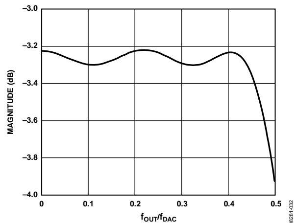
Figure 62. Sample Composite Responses of the \text{Sinc}^{-1} Filter with \sin(x)/x Roll-Off
