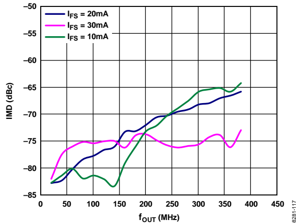
Figure 20. IMD vs. f_{OUT} over f_{SC} , 2x Interpolation, f_{DATA} = 400 MSPS, Digital Scale = 0 dBFS
