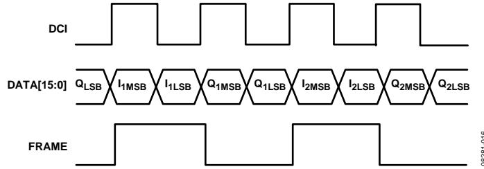
Figure 45. Timing Diagram for Byte Mode
