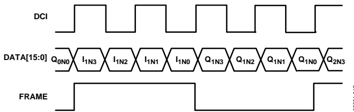
Figure 46. Timing Diagram for Nibble Mode
