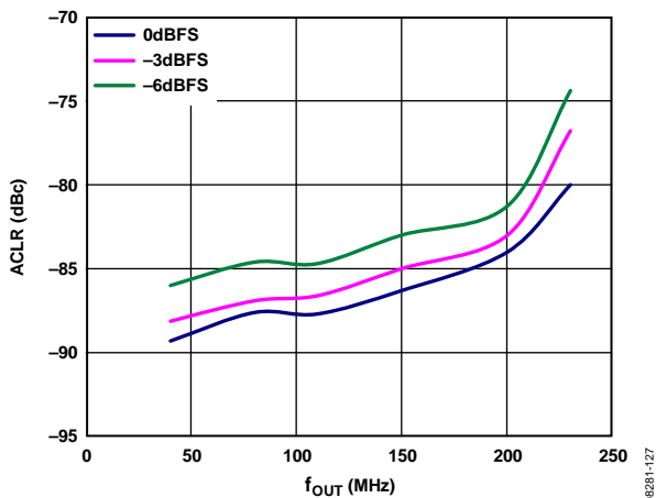
Figure 30. 1-Carrier W-CDMA ACLR vs. f_{OUT} over f_{DAC} , Second Alternate Channel, PLL Off
