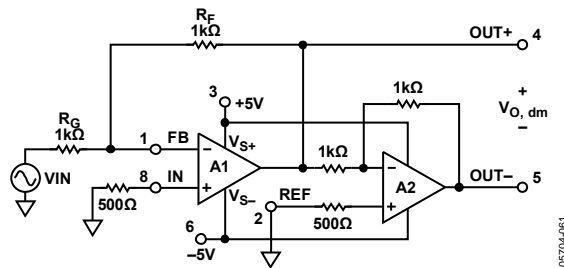
Figure 57. Gain of -2 Configuration
