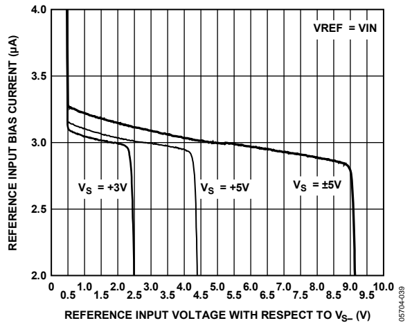
Figure 40. REF Input Bias Current vs. REF Input Voltage
