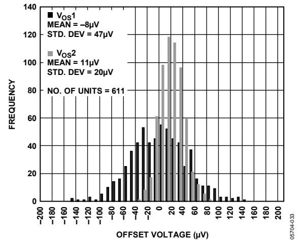
Figure 34. Differential Output Offset Distribution
