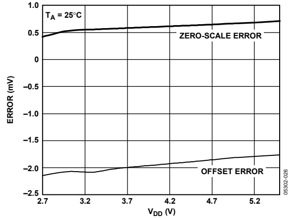
Figure 26. Zero-Scale Error and Offset Error vs. Supply Voltage
