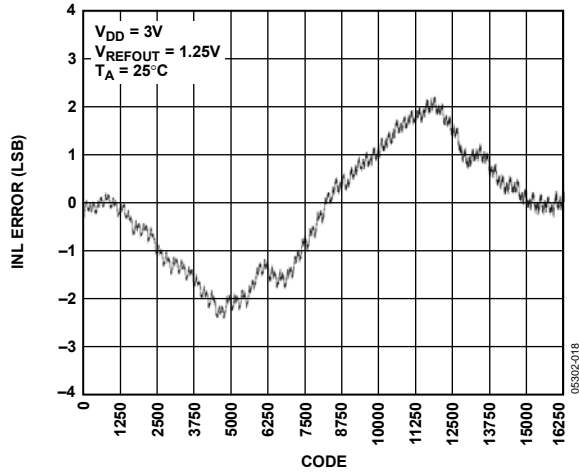
Figure 18. INL AD5648-1
