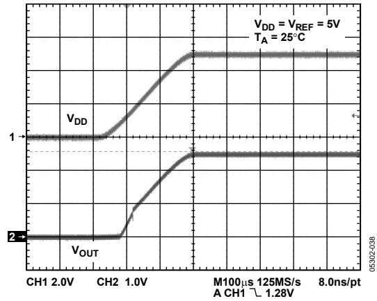
Figure 38. Power-On Reset to Midscale
