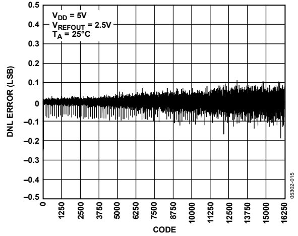
Figure 15. DNL AD5648-2
