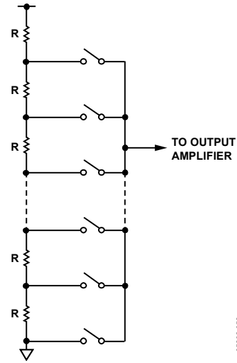
Figure 52. Resistor String
