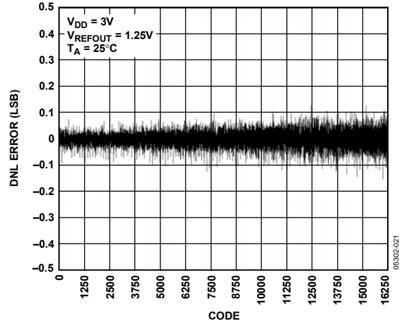
Figure 21. DNL AD5648-1
