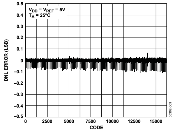
Figure 9. DNL AD5648—External Reference
