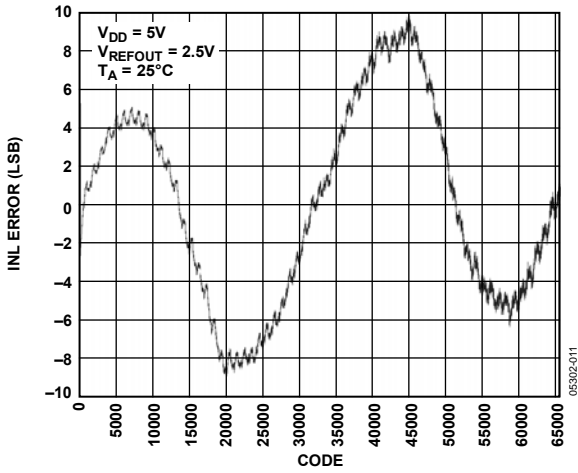
Figure 11. INL AD5668-2/AD5668-3
