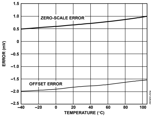
Figure 24. Zero-Scale Error and Offset Error vs. Temperature
