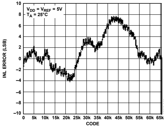
Figure 5. INL AD5668—External Reference
