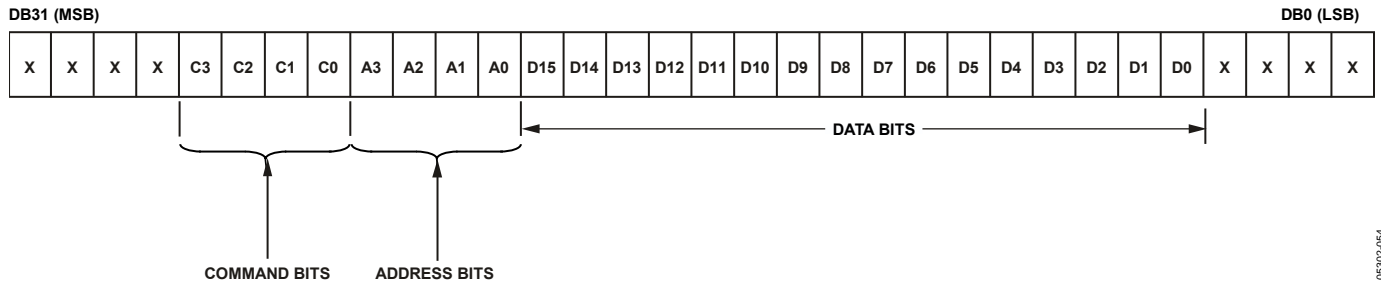
Figure 53. AD5668 Input Register Contents
