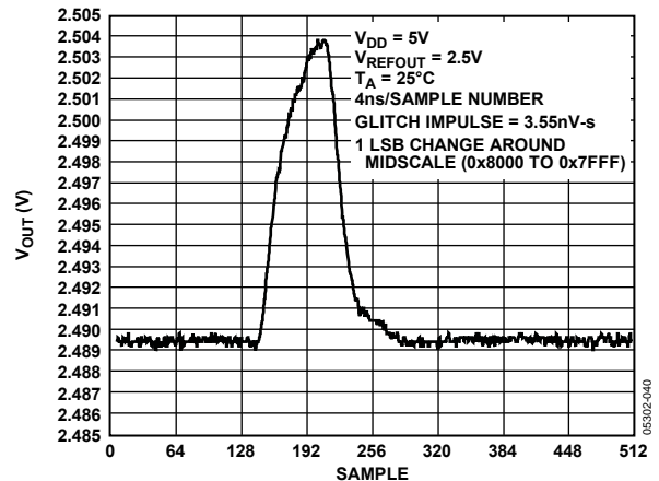
Figure 40. Digital-to-Analog Glitch Impulse (Negative)
