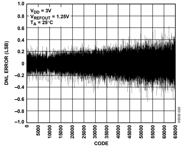
Figure 20. DNL AD5668-1
