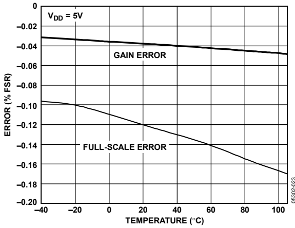
Figure 23. Gain Error and Full-Scale Error vs. Temperature
