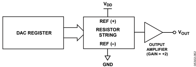
Figure 51. DAC Architecture
