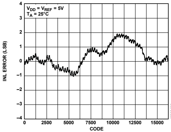
Figure 6. INL AD5648—External Reference
