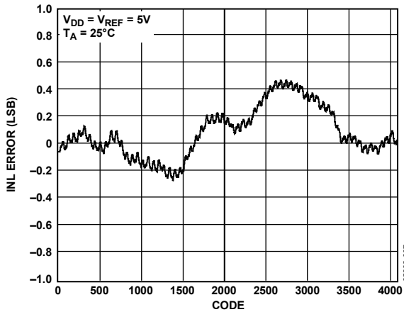
Figure 7. INL AD5628—External Reference
