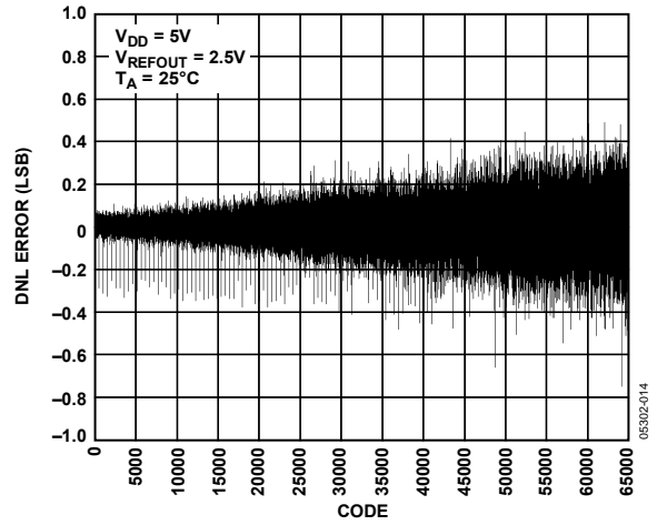
Figure 14. DNL AD5668-2/AD5668-3
