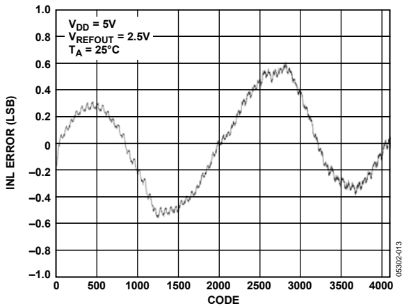
Figure 13. INL AD5628-2
