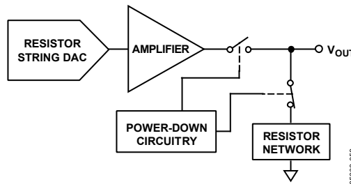
Figure 57. Output Stage During Power-Down
