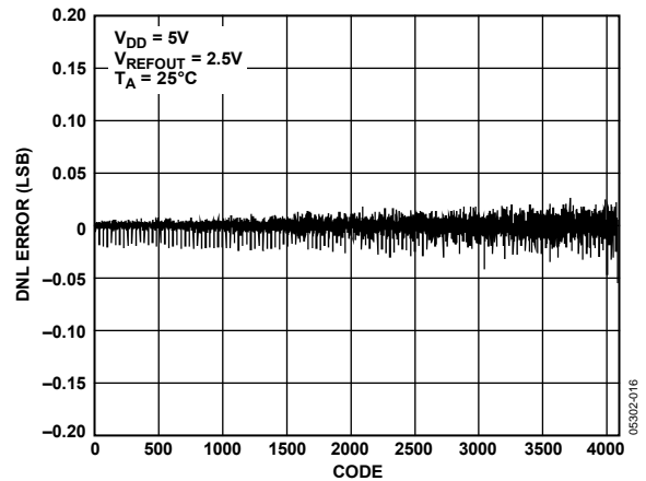
Figure 16. DNL AD5628-2
