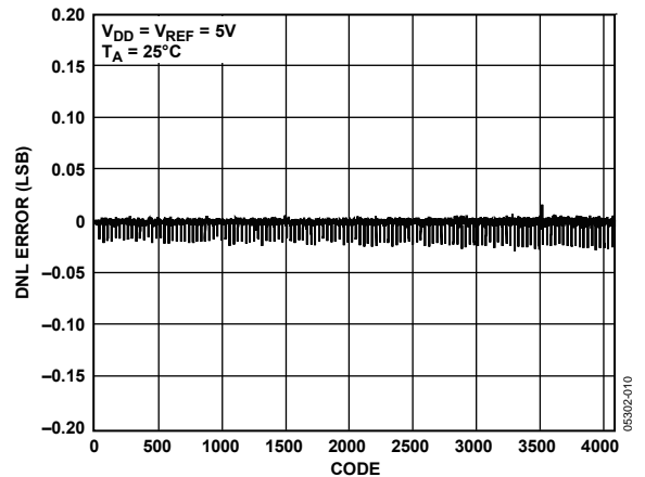
Figure 10. DNL AD5628—External Reference
