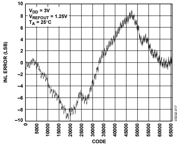
Figure 17. INL AD5668-1
