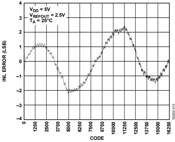
Figure 12. INL AD5648-2
