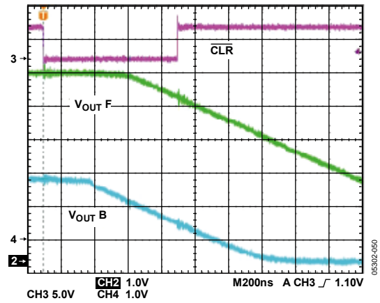
Figure 49. Hardware \overline{CLR}
