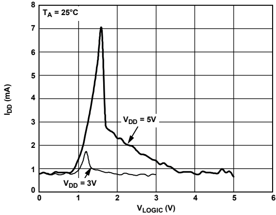
Figure 35. Supply Current vs. Logic Input Voltage
