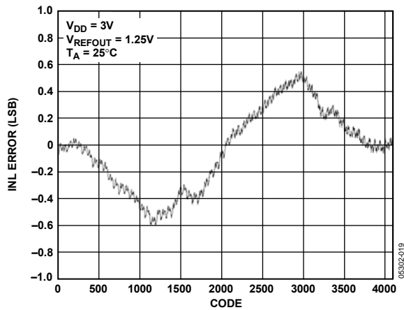
Figure 19. INL AD5628-1
