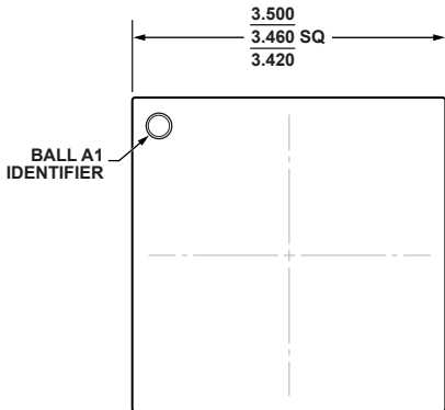
TOP VIEW (BALL SIDE DOWN)
