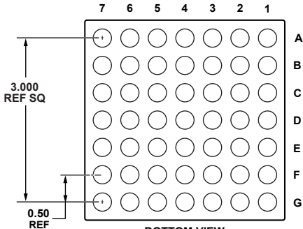
BOTTOM VIEW (BALL SIDE UP)
