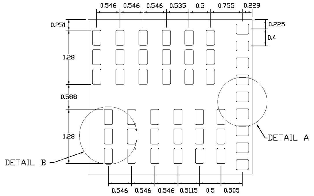
BOTTOM VIEW
