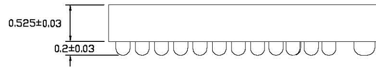
SIDE VIEW
