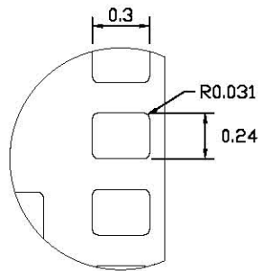
DETAIL A TYP. 9PL
