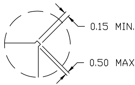
DETAIL 'C' EXPOSED PAD CORNER TAB DETAIL
