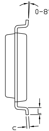
END VIEW
