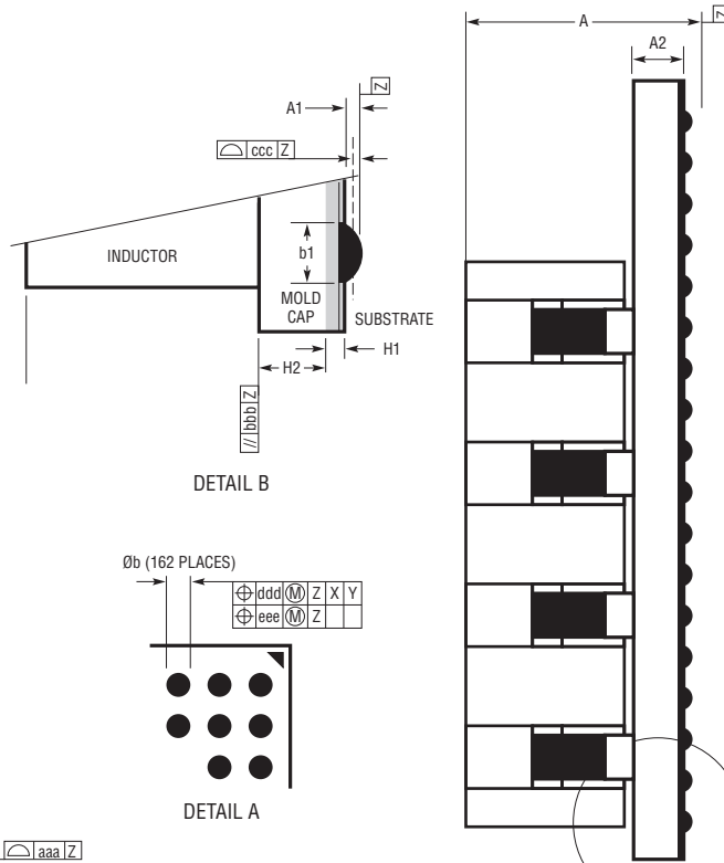
PACKAGE SIDE VIEW
