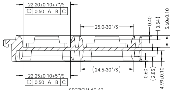
SECTION AT-AT SCALE 1.5 : 1
