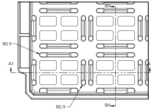
DETAIL AD SCALE 1.5 : 1
