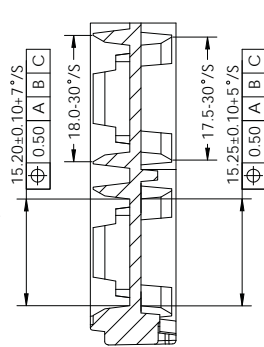
SECTION BH-BH SCALE 1.5 : 1
