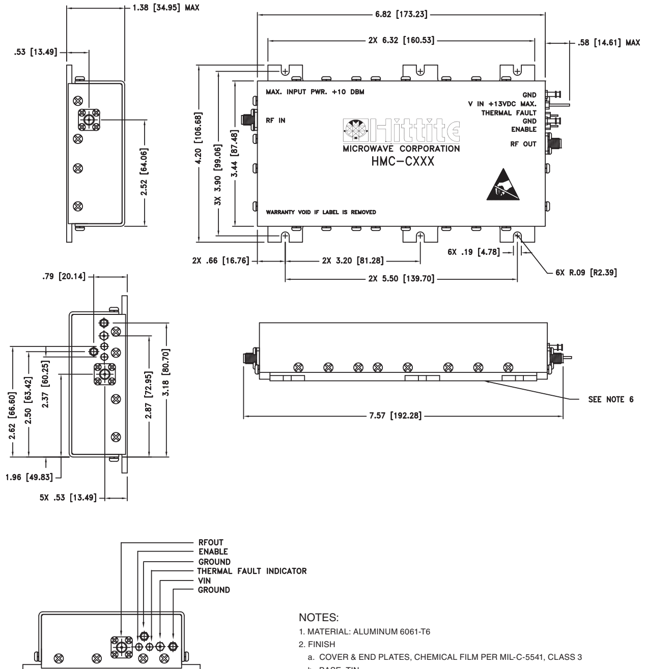
C-7 Package Outline Drawing
