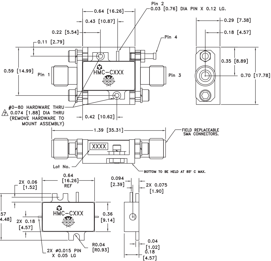
C-1 Package Outline Drawing
