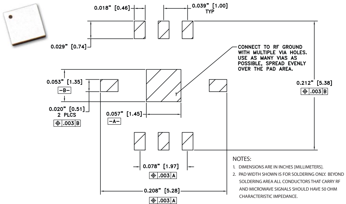
Suggested LM1 PCB Land Pattern
