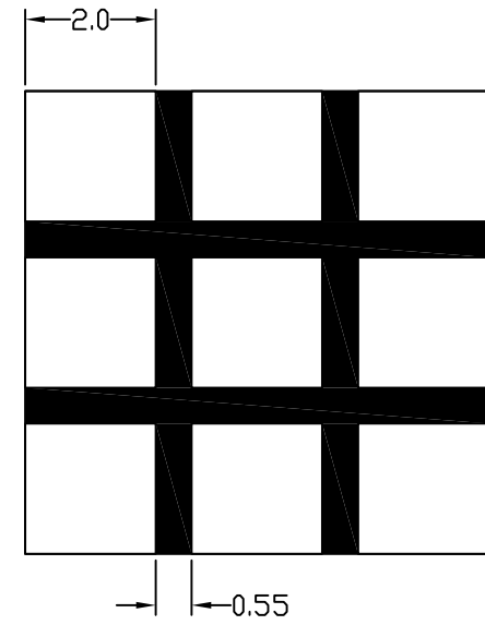
RECOMMENDED GND SOLDER PAD
