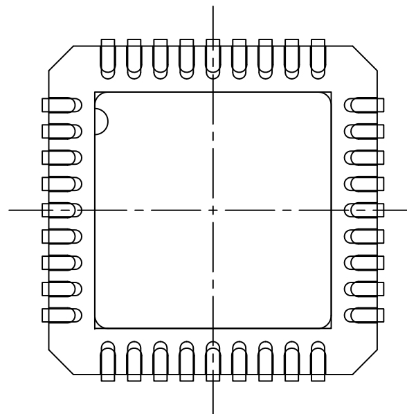
PACKAGE OVERLAY
